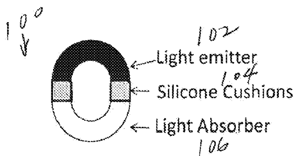
Coronal section of the sensor
