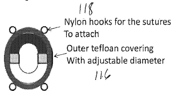
Coronal section of the sensor with outer covering
