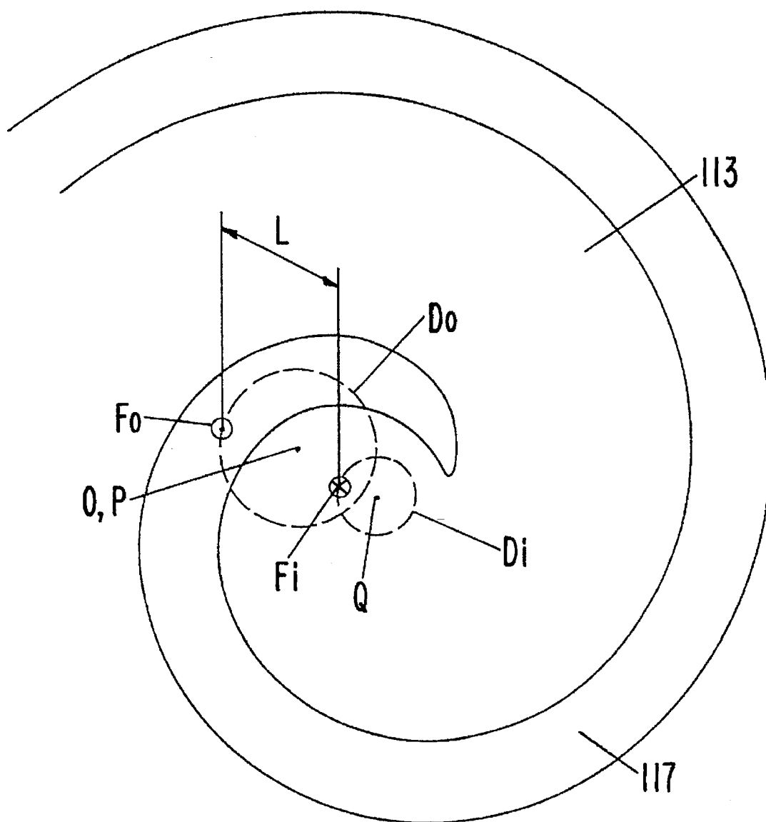
FIG. 16 (PRIOR ART)
