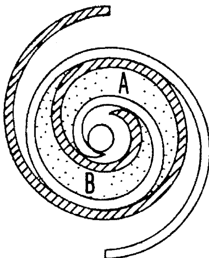
FIG. 15C (PRIOR ART)
