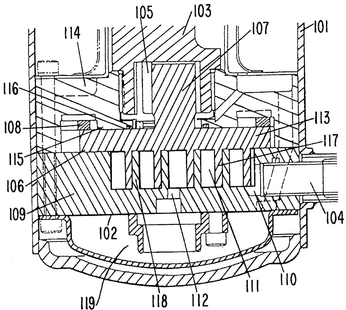
FIG. 14 (PRIOR ART)
