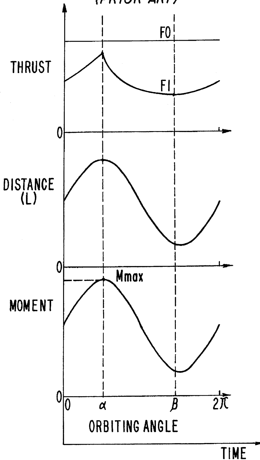
FIG. 17 (PRIOR ART)
