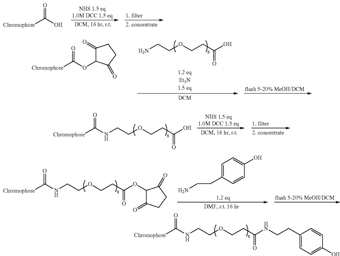
Scheme 2
