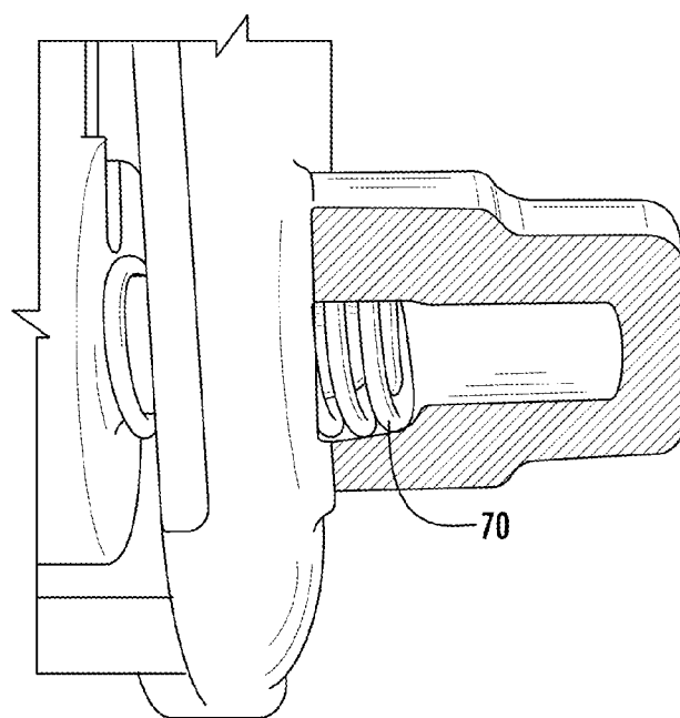
FIG. 8 PRIOR ART
