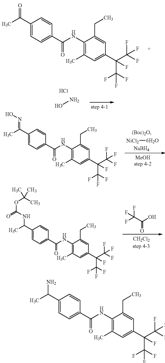
Scheme 4:
