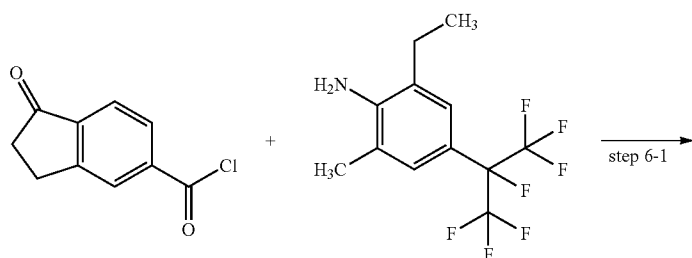
Scheme 6:
