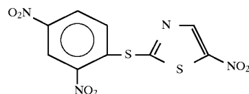
COMPOUND 12
