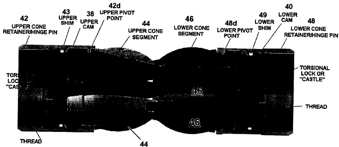
EXPANDABLE/COLLAPSIBLE CONE ASSY - FULL COLLAPSED POSITION
