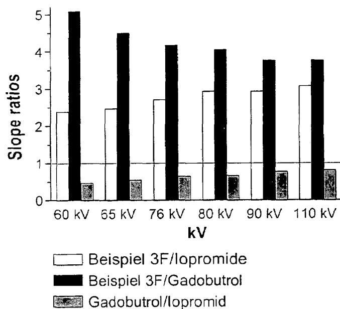
Figure 6: Relative X-ray Absorption of Example 3F in Comparison with Gadobutrol and Iopromide at Various Anode Voltages of X-ray Tubes (Stenoscope D6, General Electric). [Key to Fig. 6:] Beispiel = Example, Ipromid = Iopromide
