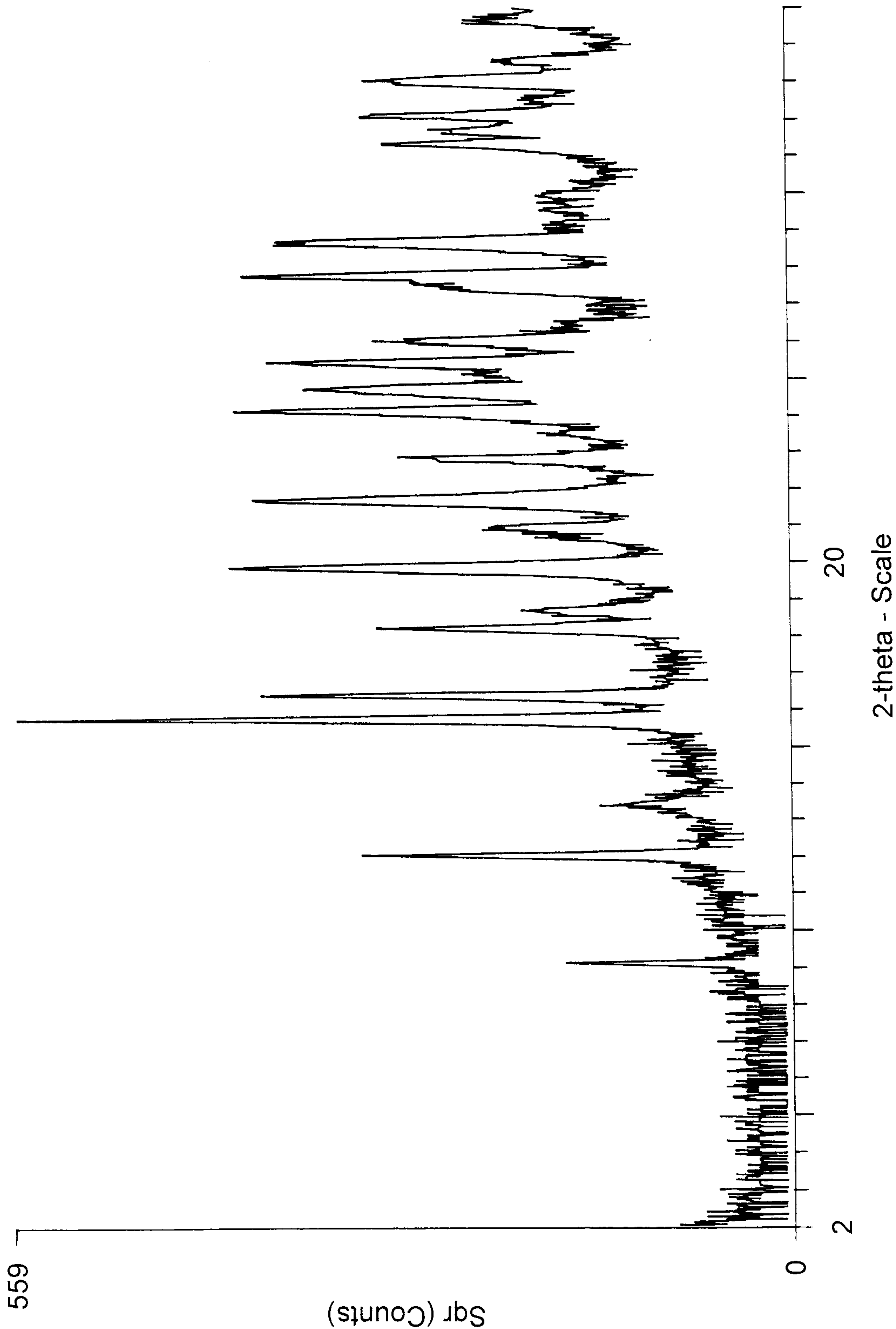
Fig. 2 X-Ray Powder Diffraction Pattern of Hydrochloride Hydrate
