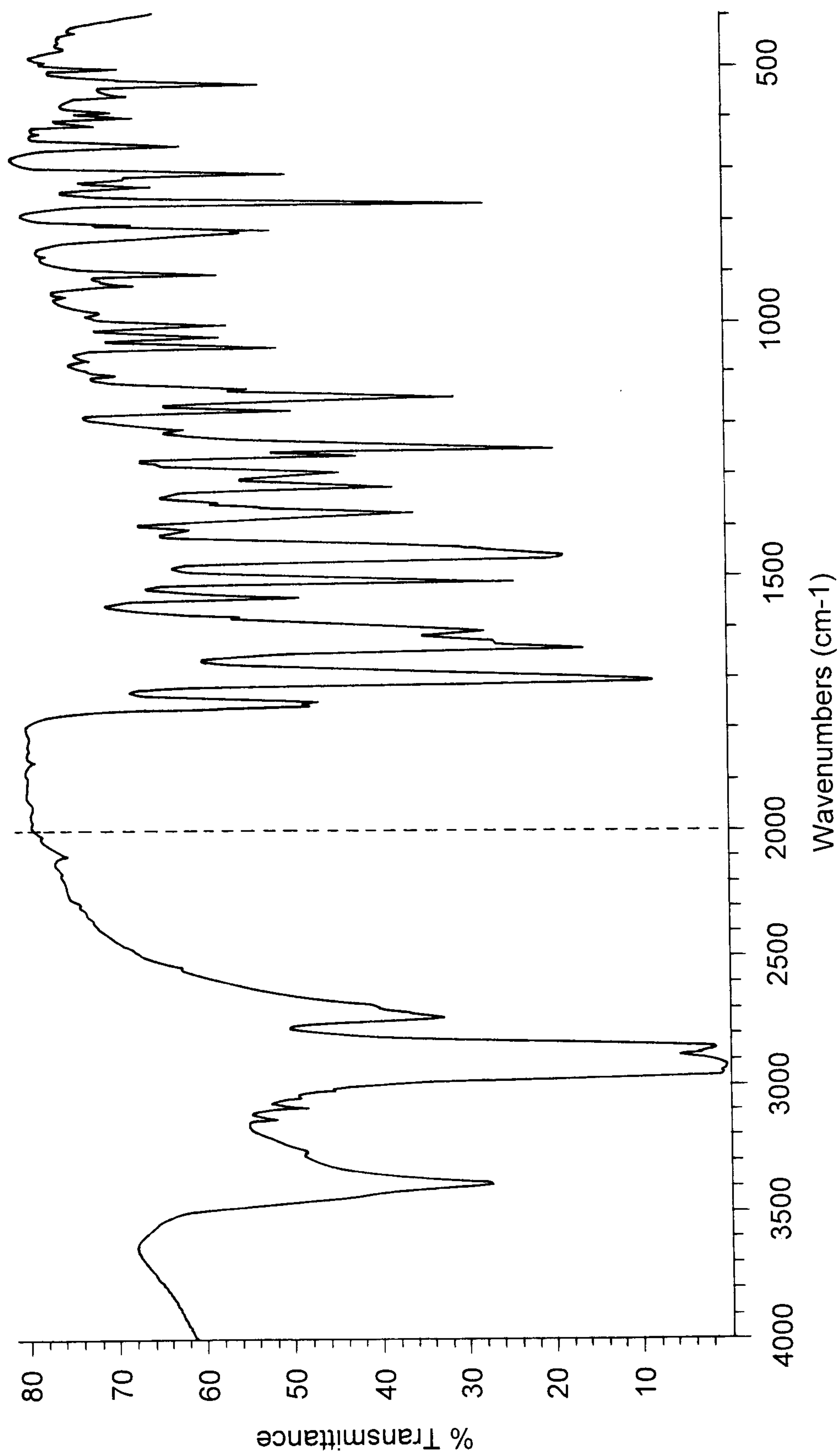
Fig. 1 Infrared Spectrum of Hydrochloride Hydrate.
