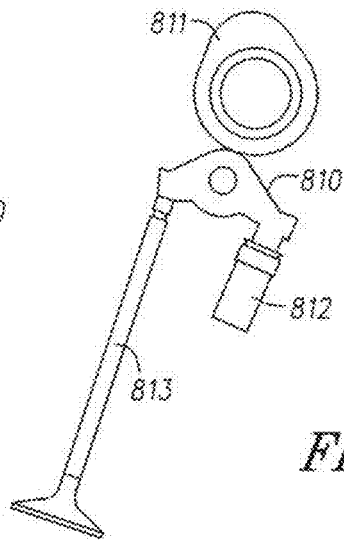
FIXED LIFT EXHAUST VALVE LINE
