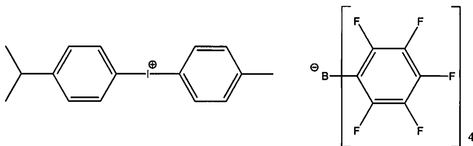
tetrakis(2,3,4,5,6-pentafluorophenyl)borate(1-)[4-(1-methylethyl)phenyl] (4-methylphenyl)-Iodonium
