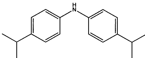
bis(4-isopropylphenyl)amine
