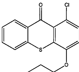
1-chloro-4-propoxy-9H-Thioxanthen-9-one
