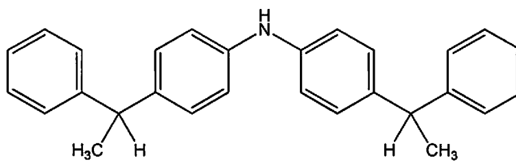
bis(4-(1-phenylethyl)phenyl)amine
