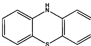
10H-Phenothiazine
