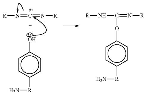
Reaction E:
