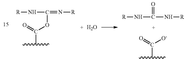
Reaction G:
