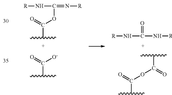
Reaction H:
