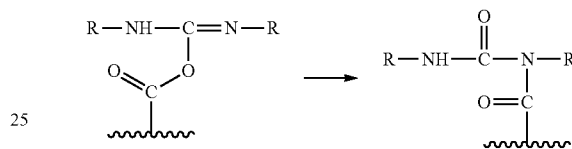
Reaction H:
