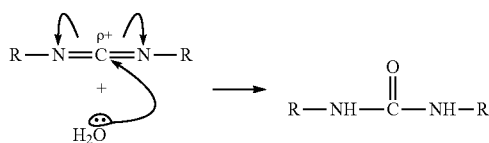
Reaction E:
