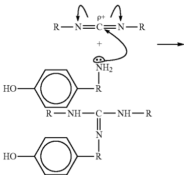
Reaction D:
