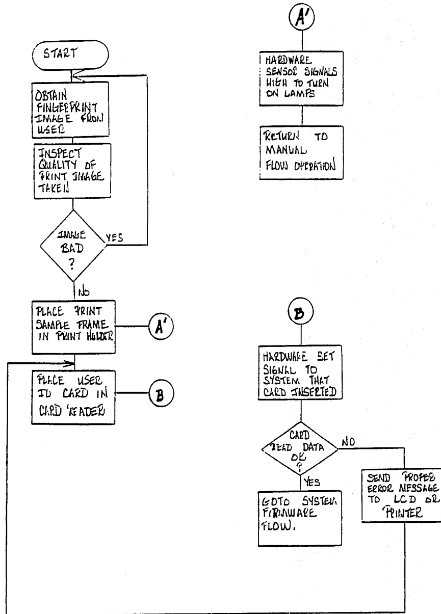
SYSTEM MANUAL & HARDWARE FLOW
