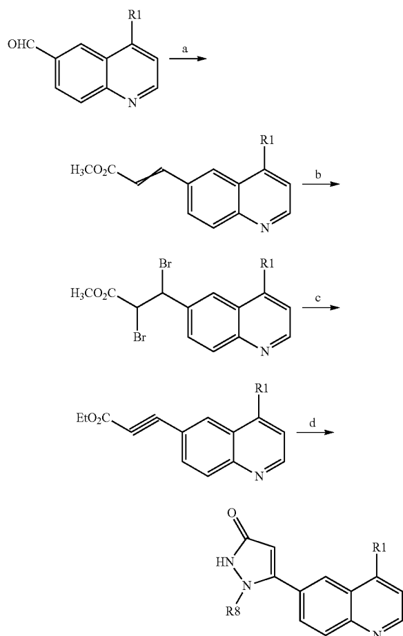
Scheme 15:
