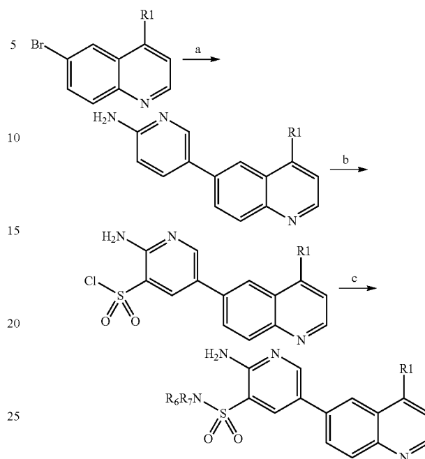
Scheme 8:
