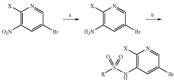
Scheme 14:
