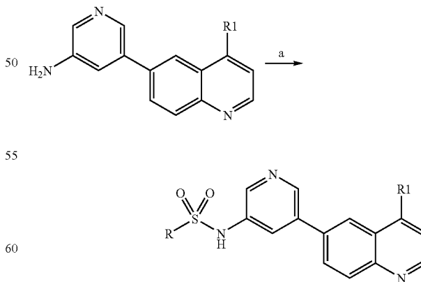
Scheme 11:
