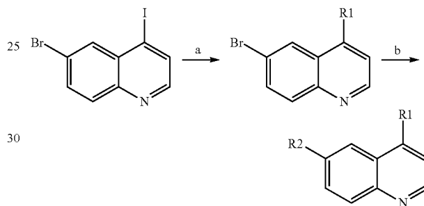
Scheme 16:
