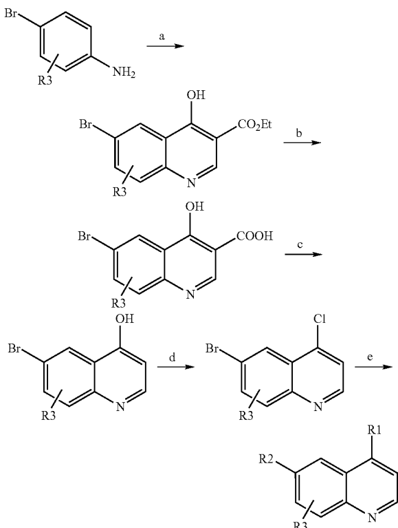
Scheme 7:
