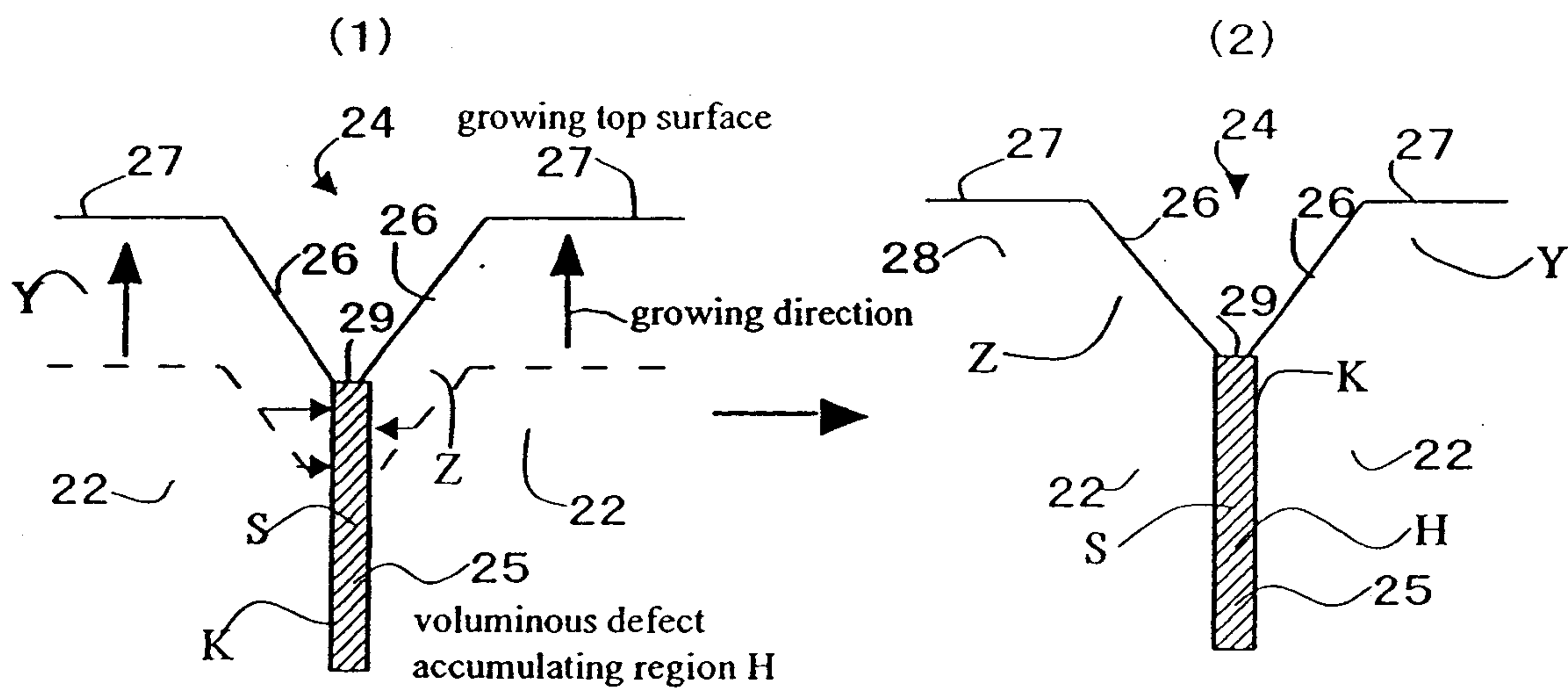
Fig.4 Growing method of the present invention
