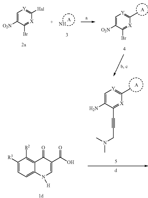
Scheme 2. Preparation of Compounds of Formula I
