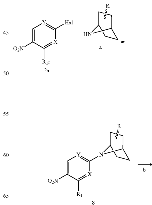
40 Scheme 3. Preparation of Compounds of Formula I Where R is H or OH)
