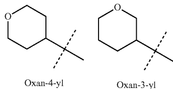
Oxan-4-yl
