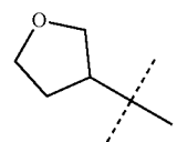
Tetrahydrofuran-3-yl
