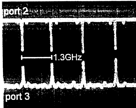
Figure 6. Spectral scans measured at taper ports #2 and #3 when a single frequency tunable laser source is input at port 1 and scanned in this case by approximately 5 GHz. The extinctions of optical power in the upper traces correspond to excitation of whispering gallery modes of the microsphere. These extinctions exceed 23 dB. Correspondingly, the energy that is coupled from the upper taper is transferred to the lower fiber taper with high efficiency. To date we estimate efficiencies better than 99%.
