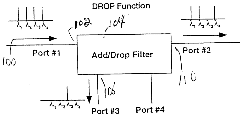
Figure 1A Illustration of the Drop function in an add/drop filter. The channel at wavelength \lambda_j is shown being dropped in the schematic.
