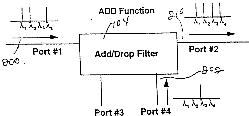
Figure 1B Illustration of the Add function in an add/drop filter. A vacant channel slot at \lambda_j is filled by input at port #4.
