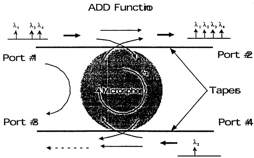
Figure 4. Illustration of the Add function in the present invention.
