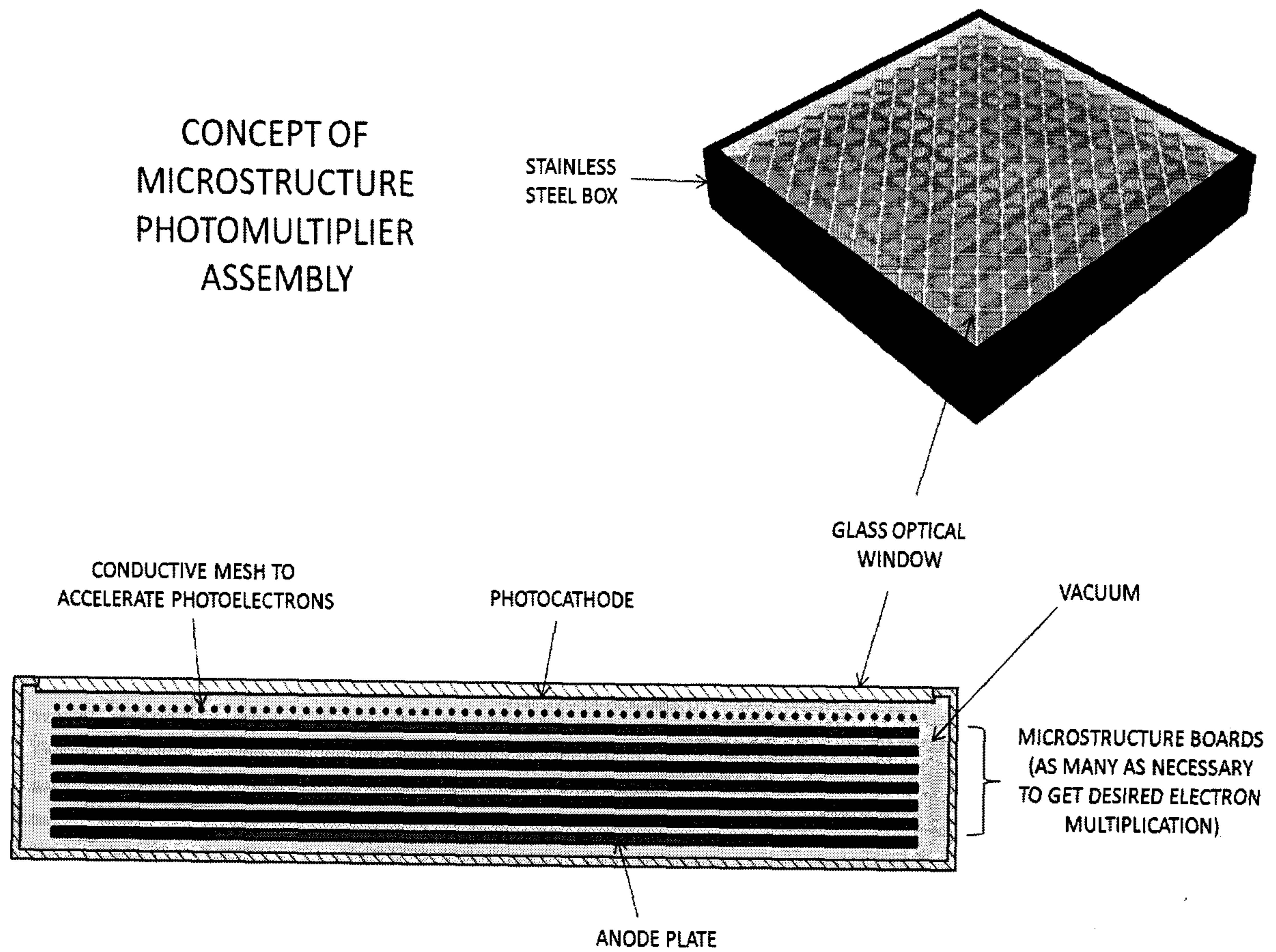
Figure 1: Concept of Microstructure Photomultiplier Assembly
