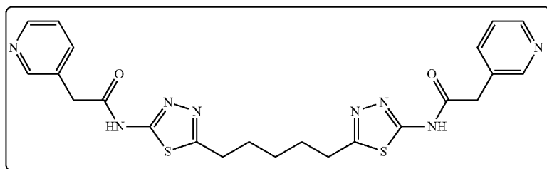
N,N'-(5,5'-(pentane-1,5-diyl)bis(1,3,4-thiadiazole-5,2-diyl))bis(2-(pyridin-3-yl)acetamide) (10)
