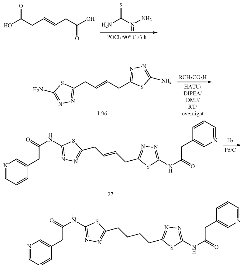
Scheme 22
