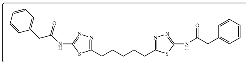
N,N'-(5,5'-(pentane-1,5-diyl)bis(1,3,4-thiadiazole-5,2-diyl))bis(2-phenylacetamide) (2)
