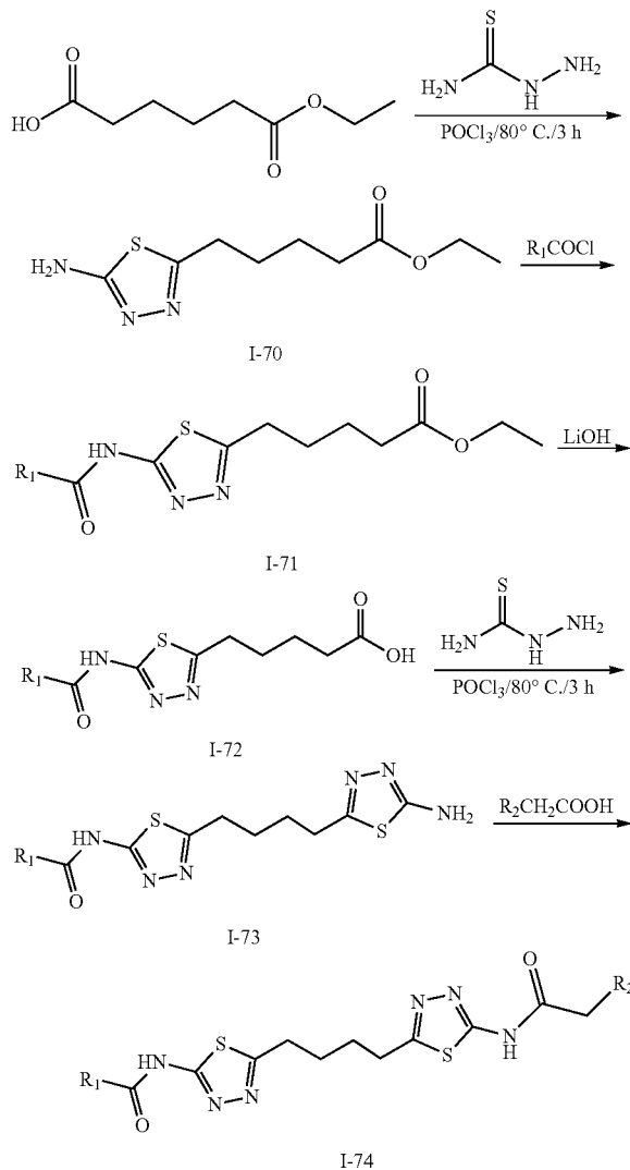
Scheme 17
