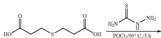
Scheme 25
