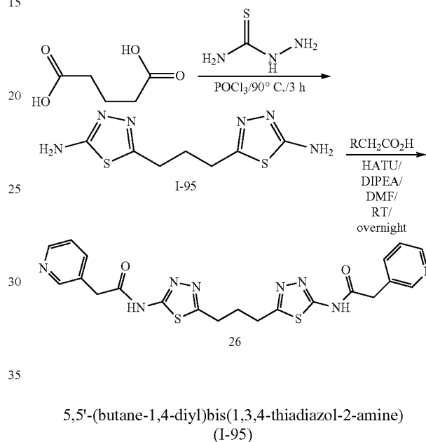
Scheme 21
