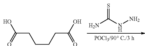
Scheme 23
