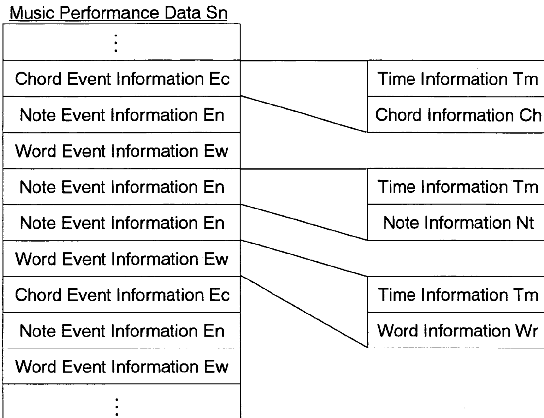
Fig.5 Format of Music Performance Data
