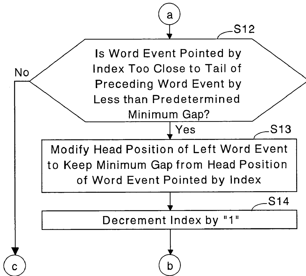
Fig. 4c Processing for Creating Word Display Data (Part 3)
