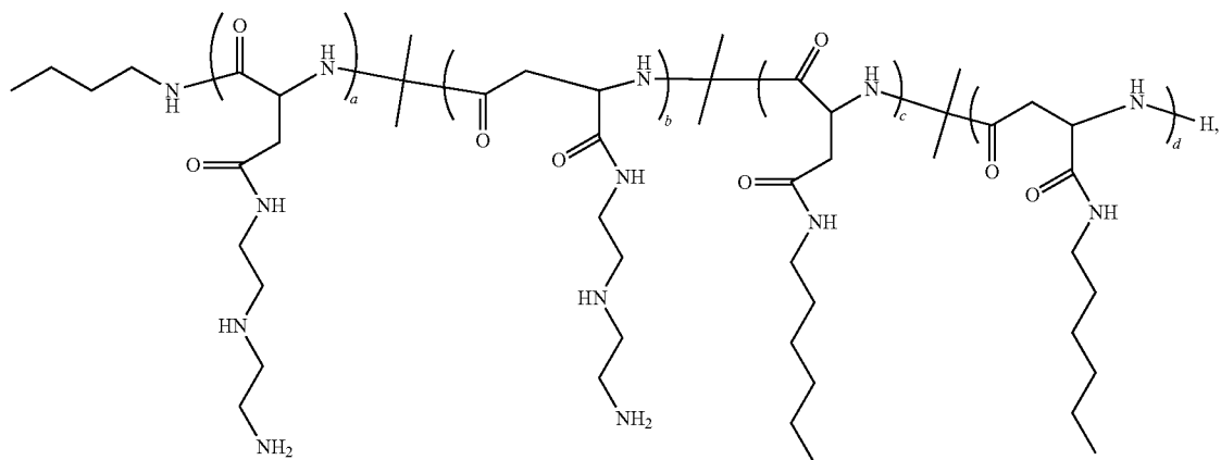
Polymer 13
