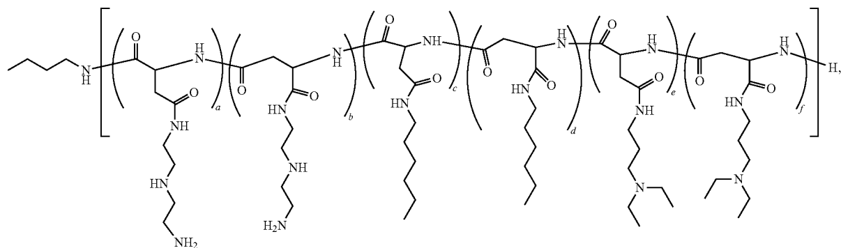
Polymer 54
