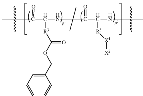
Formula 7
