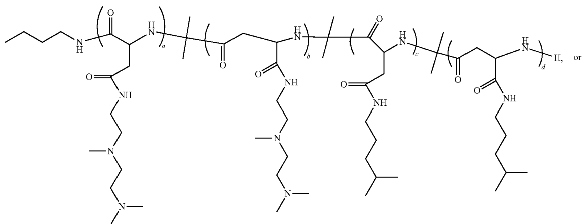
Polymer 35
