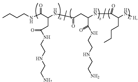
Polymer 5
