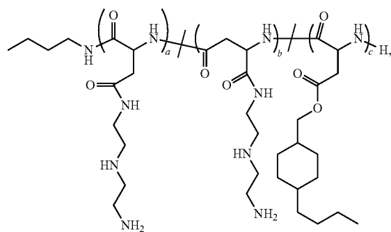
Polymer 11
