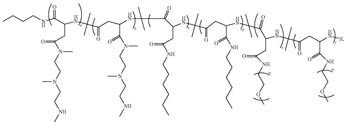
Polymer 83
