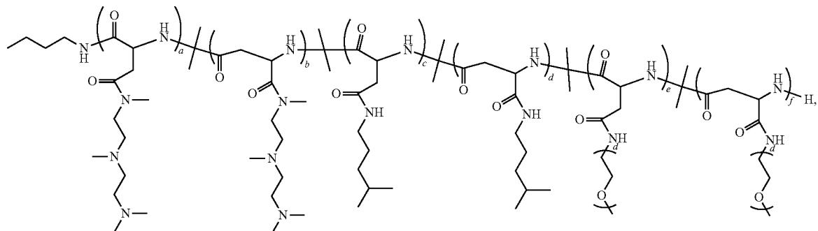
Polymer 82
