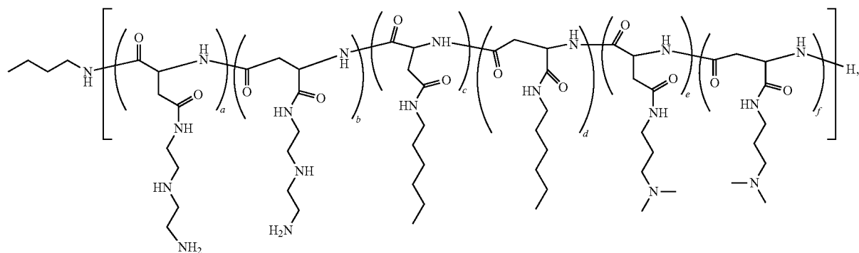
Polymer 53
