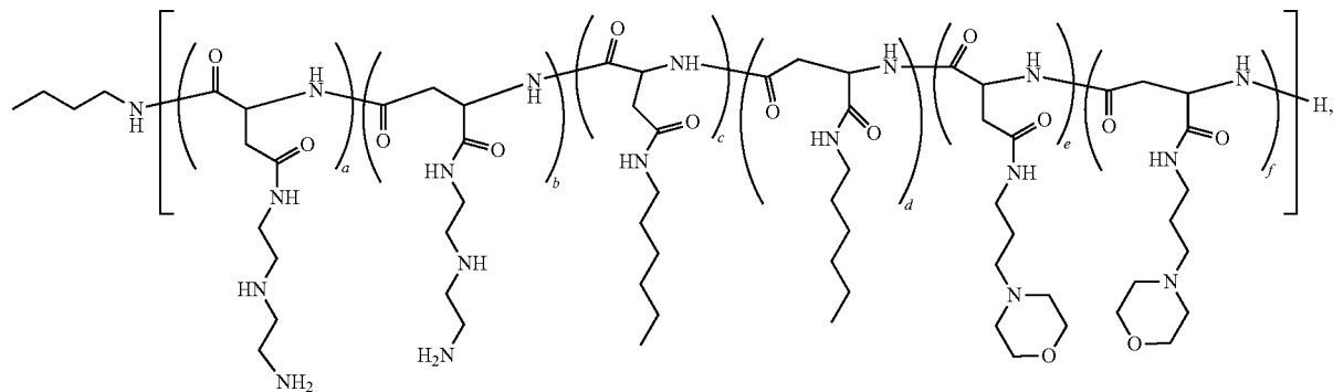
Polymer 57
