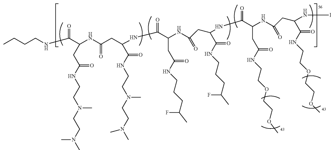
2K-PEG-Fluoro-Polymer
