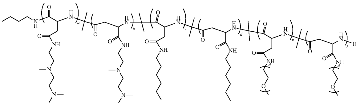
Polymer 72
