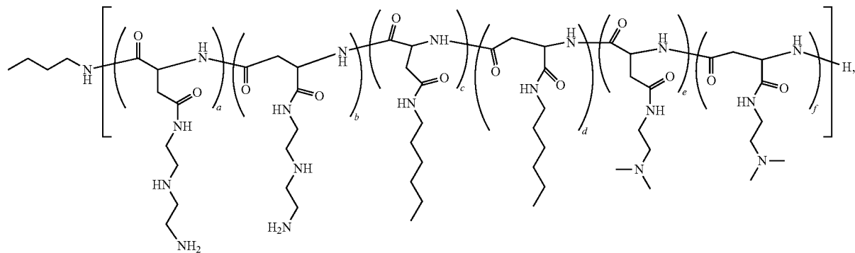
Polymer 45
