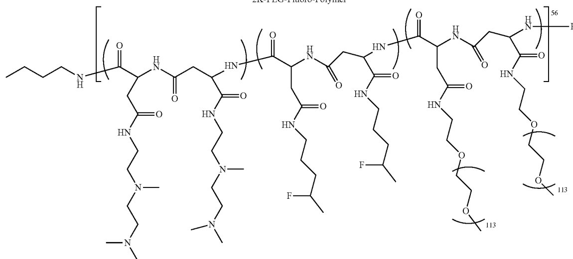
5K-PEG-Fluoro-Polymer
