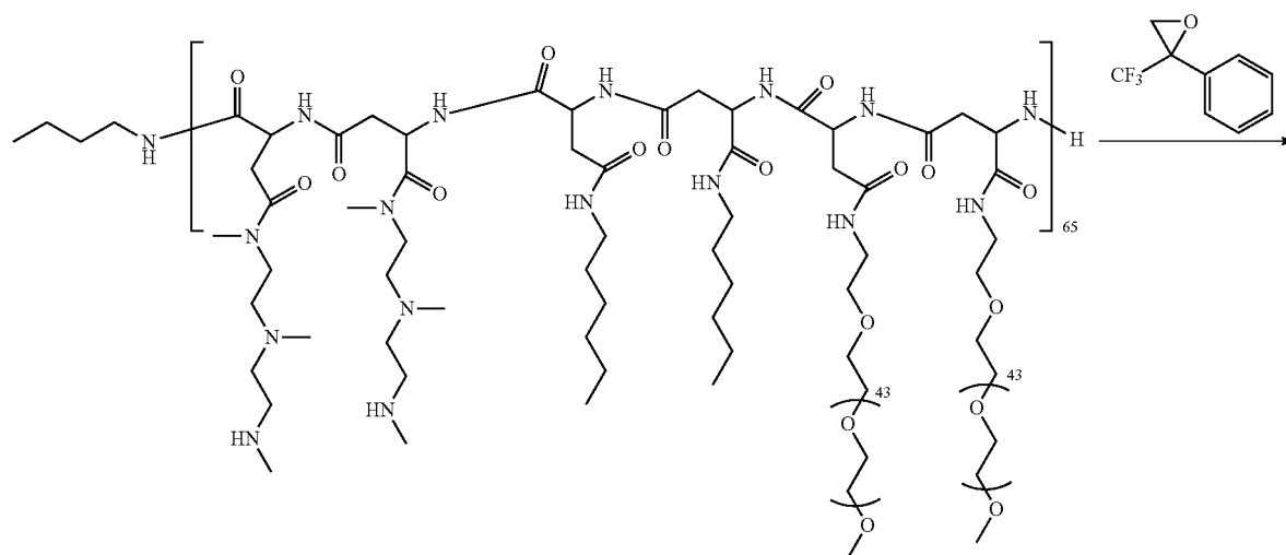
Scheme 3A
