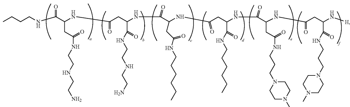
Polymer 57
