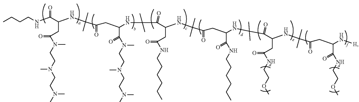
Polymer 81
