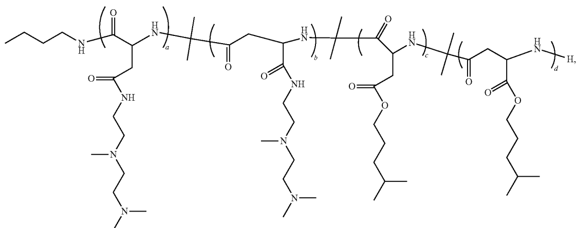
Polymer 36
