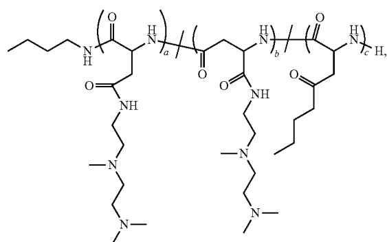
Polymer 24
