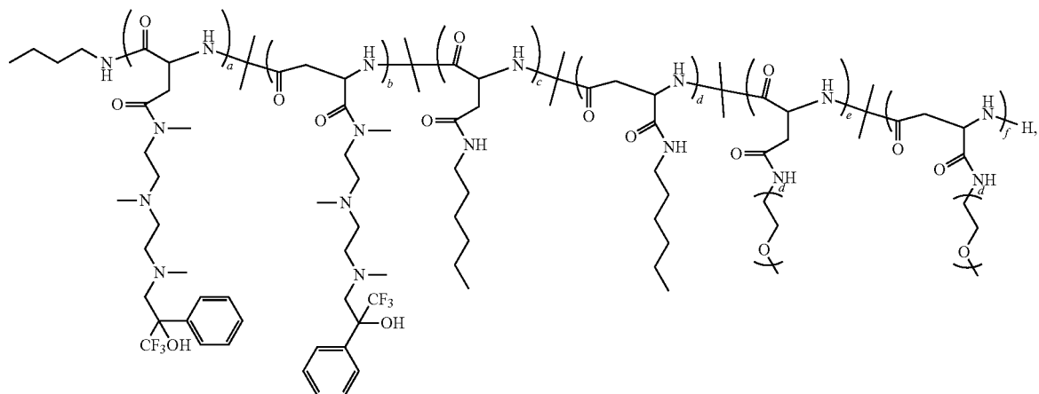
Polymer 84
