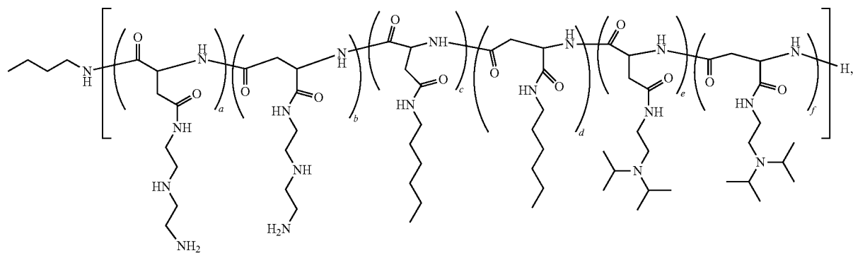
Polymer 47
