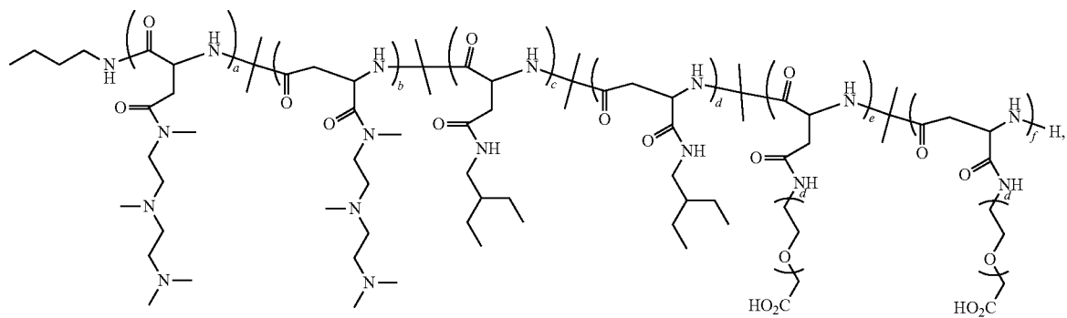
Polymer 87
