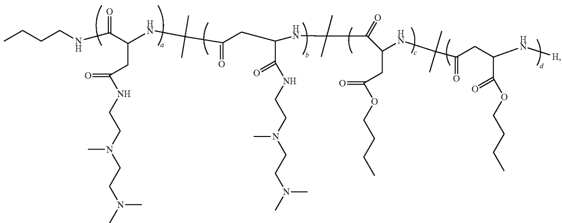
Polymer 28
