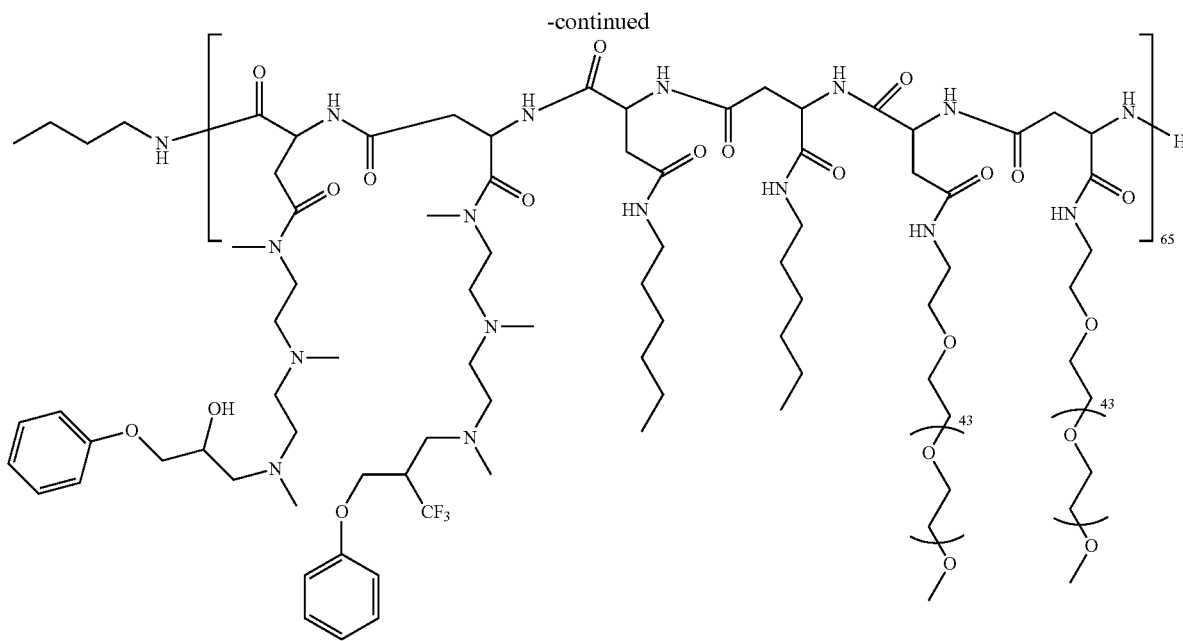
(P2K-B12)
