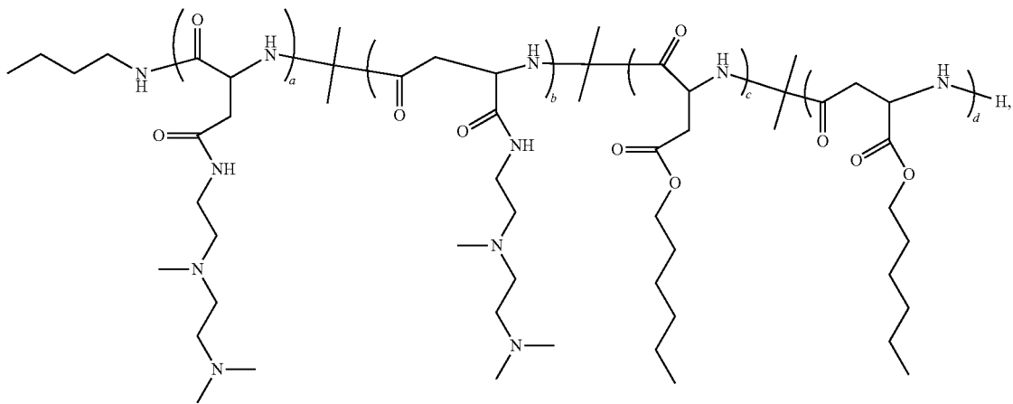
Polymer 30
