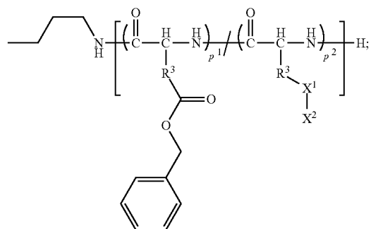
Formula 7B
