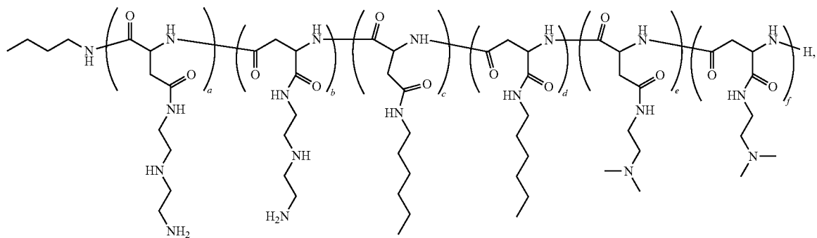
Polymer 44
