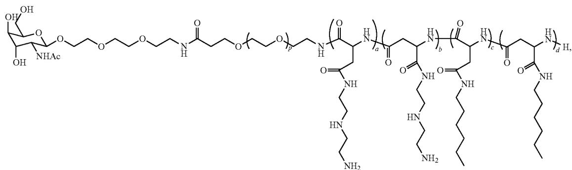
Polymer 70
