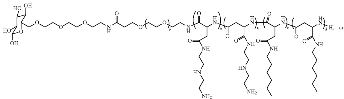
Polymer 71
