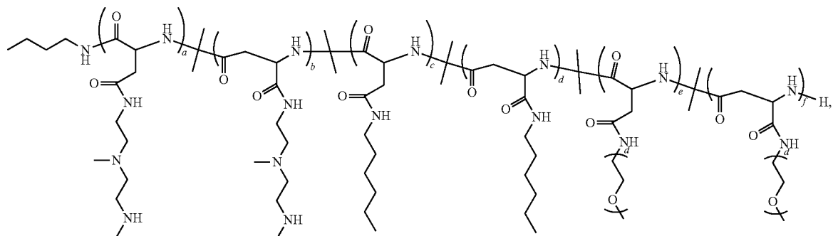
Polymer 75
