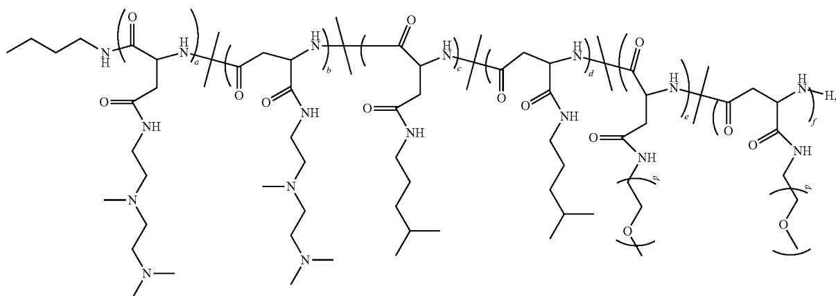
Polymer 73
