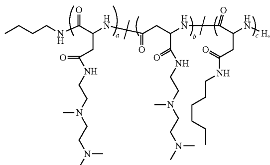
Polymer 21
