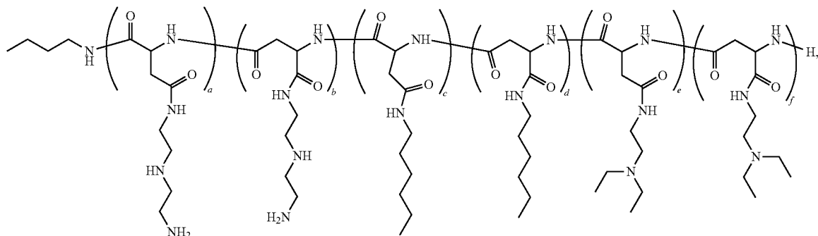
Polymer 45
