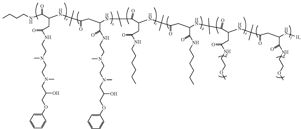
Polymer 77
