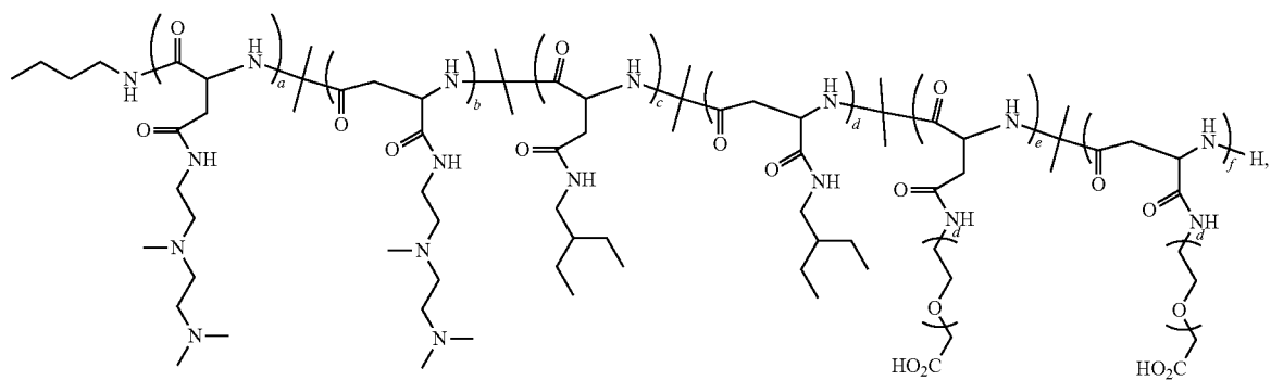
Polymer 80
