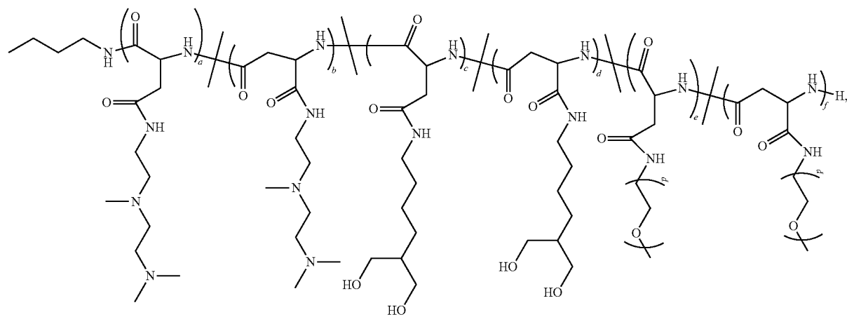
Polymer 78
