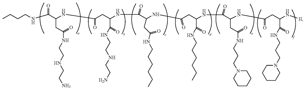
Polymer 56
