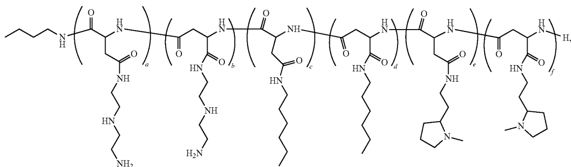
Polymer 51
