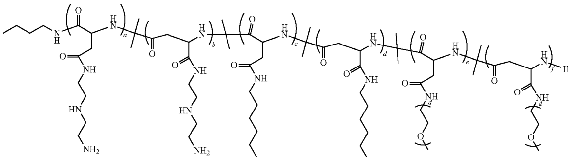
Polymer 74
