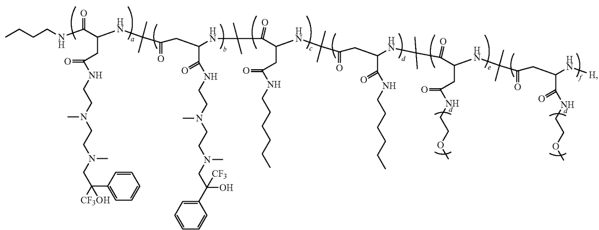
Polymer 76
