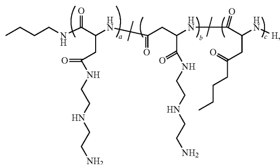
Polymer 6
