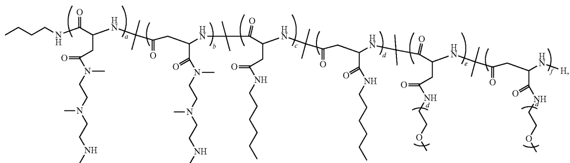
Polymer 83
