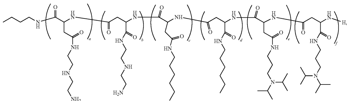
Polymer 54
