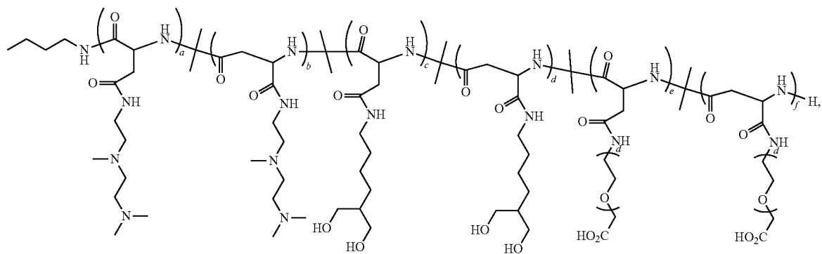
Polymer 81
