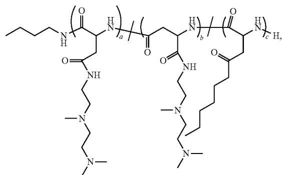
Polymer 18
