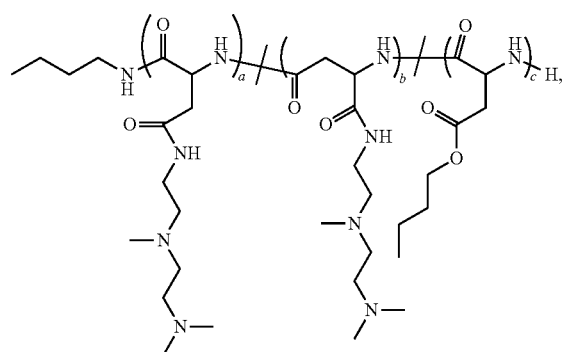
Polymer 26
