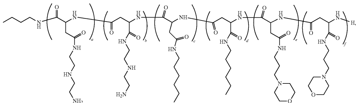
Polymer 56
