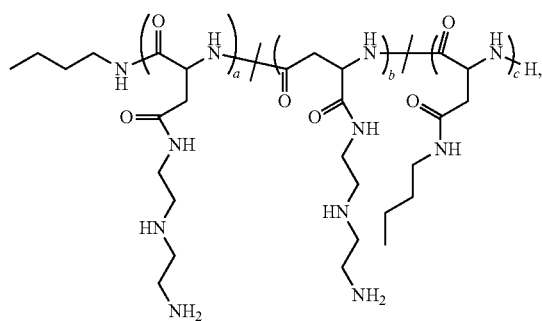
Polymer 9
