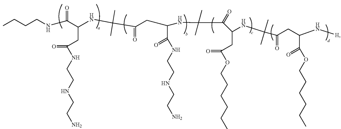
Polymer 14
