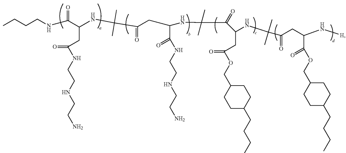
Polymer 16
