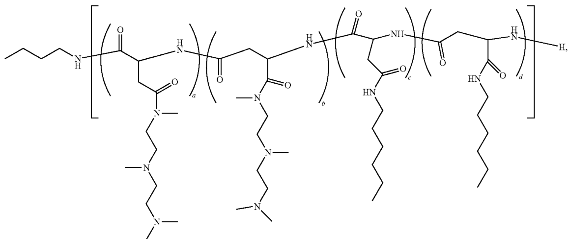
Polymer 40
