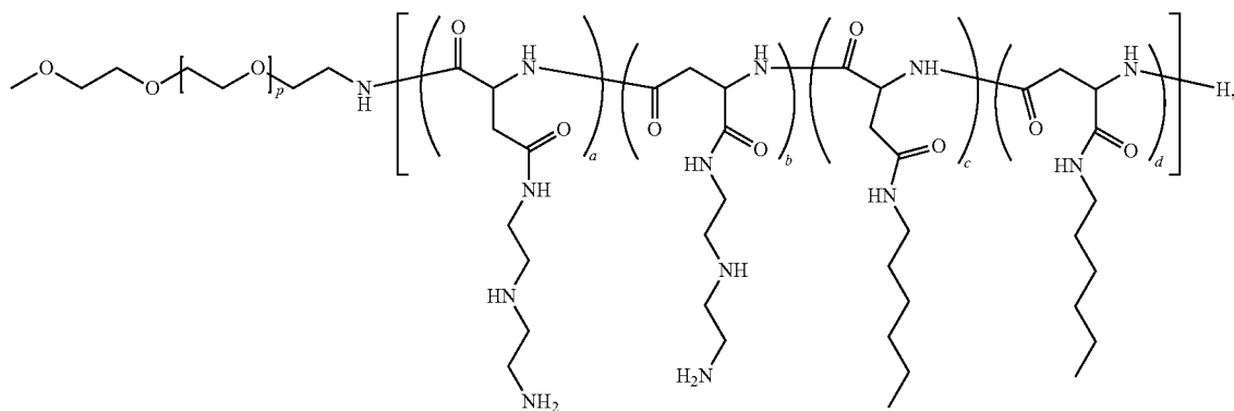
Polymer 69
