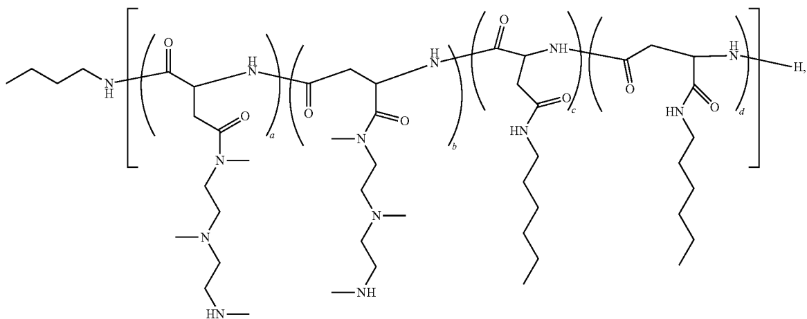
Polymer 41
