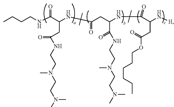
Polymer 22
