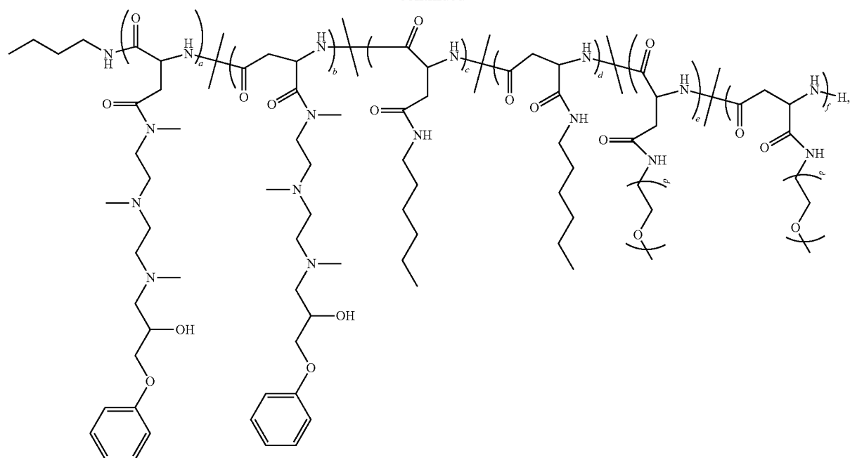
Polymer 85
