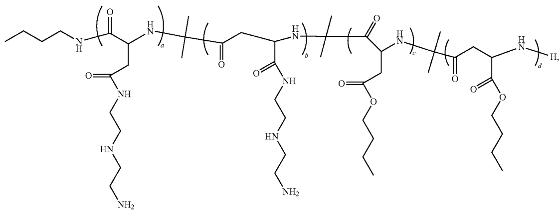
Polymer 12
