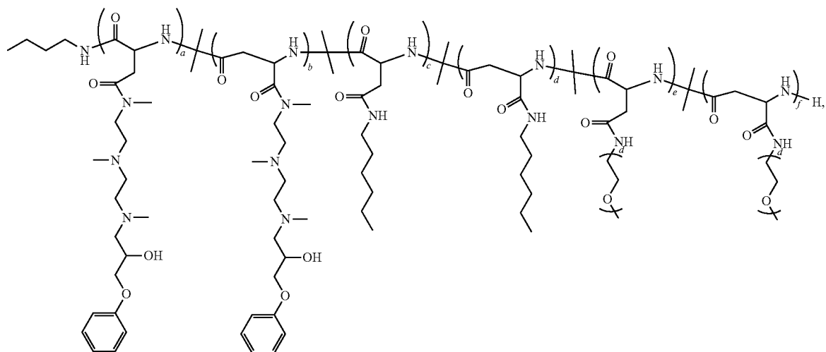
Polymer 85
