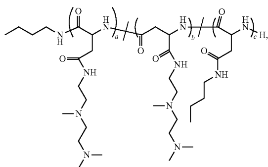
Polymer 25
