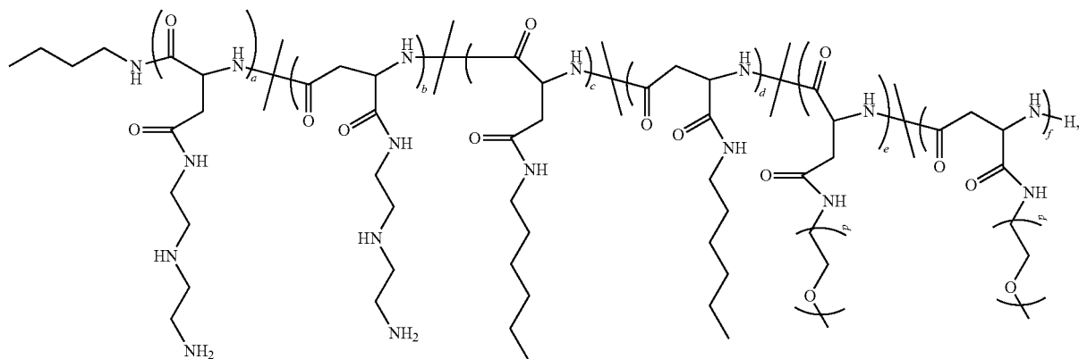
Polymer 74
