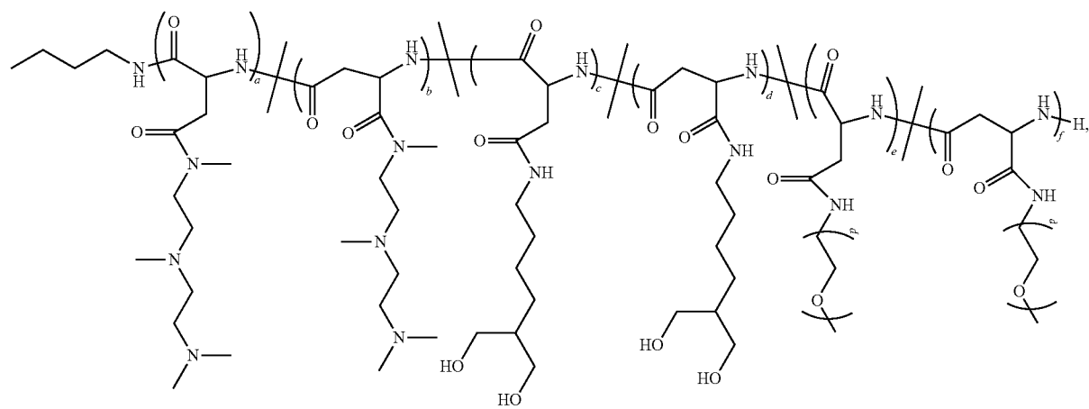
Polymer 86
