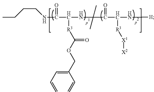
Formula 9b
