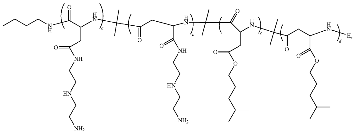
Polymer 34
