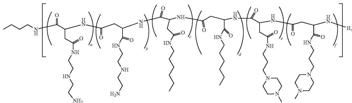
Polymer 58
