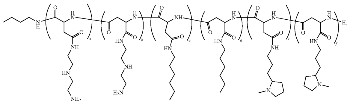
Polymer 58
