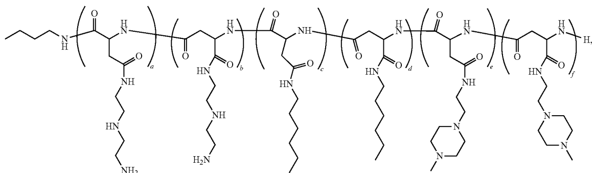
Polymer 49
