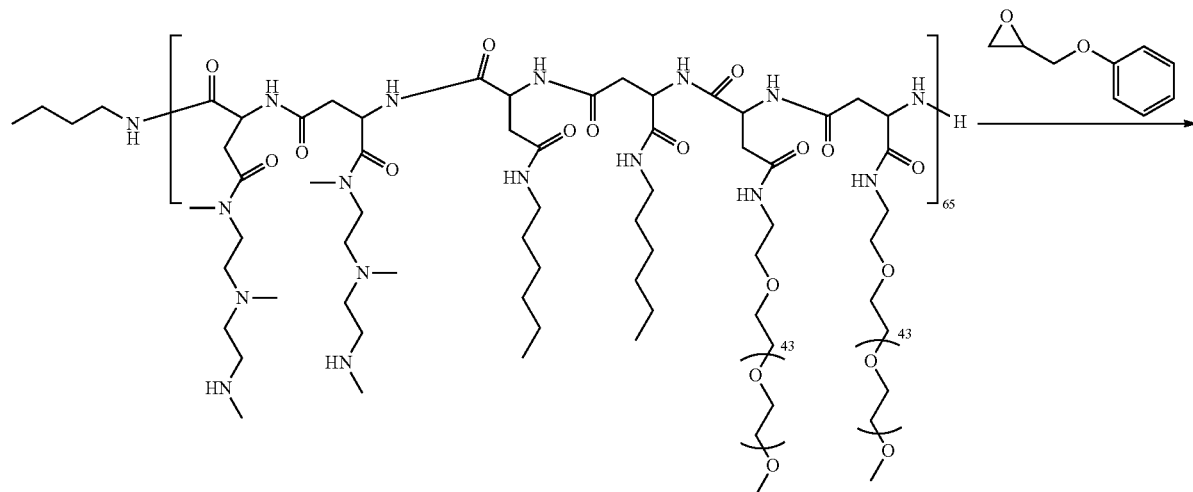
Scheme 3B
