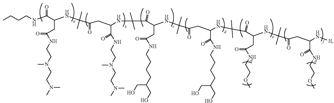
Polymer 79
