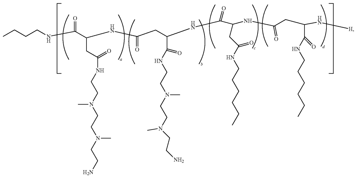
Polymer 41
