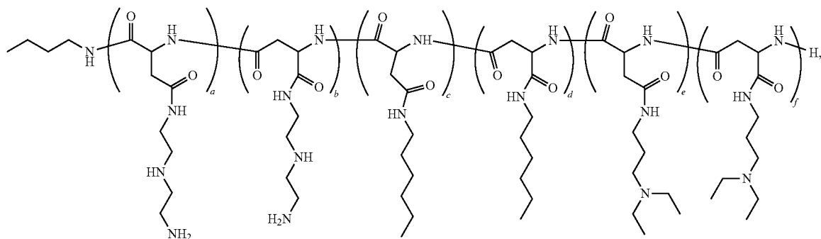
Polymer 53
