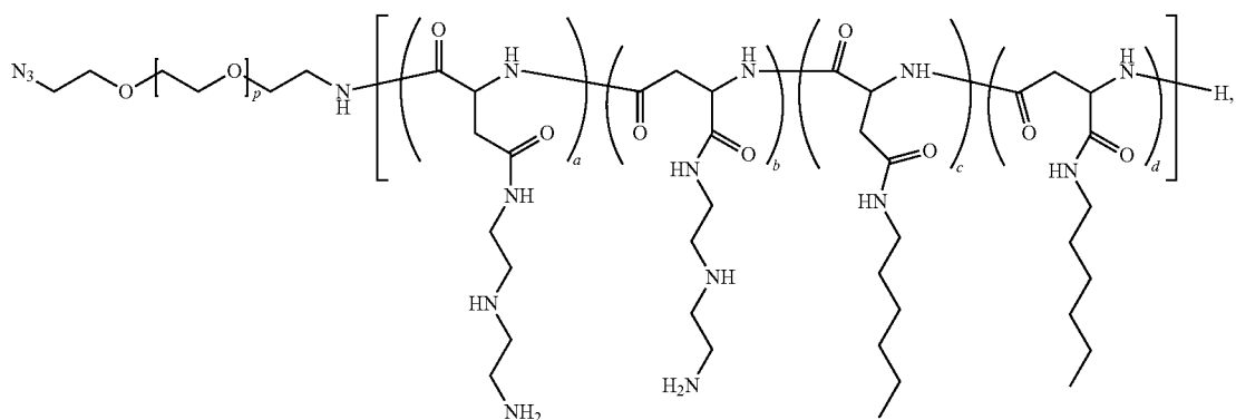
Polymer 71
