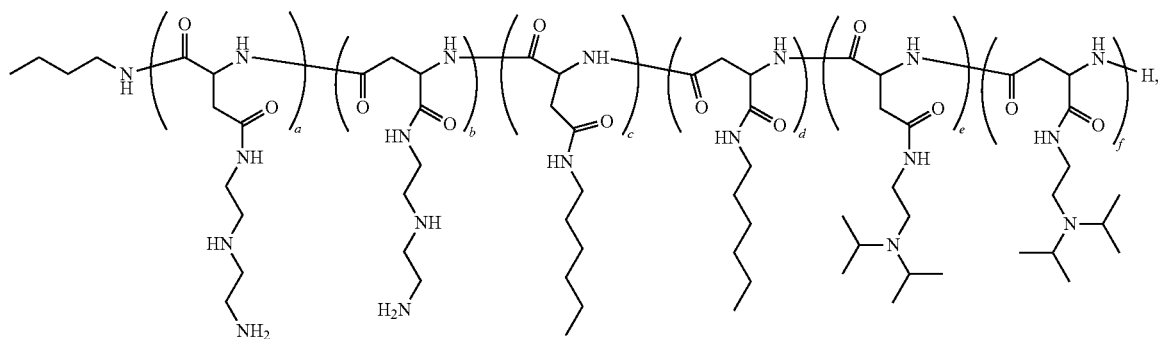
Polymer 47
