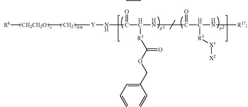
Formula 7A
