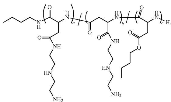
Polymer 10
