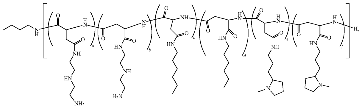
Polymer 59
