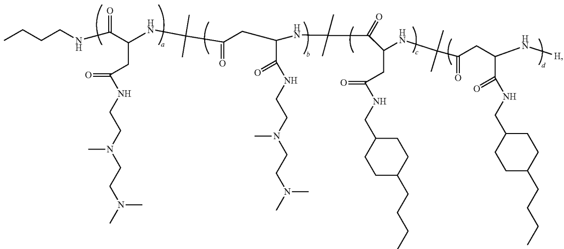
Polymer 31
