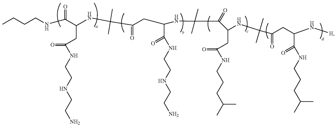
Polymer 33
