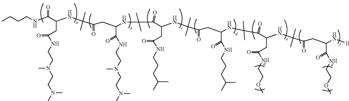
Polymer 73
