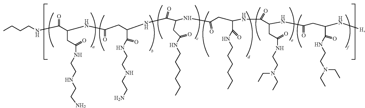
Polymer 46
