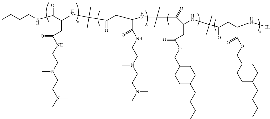
Polymer 33
