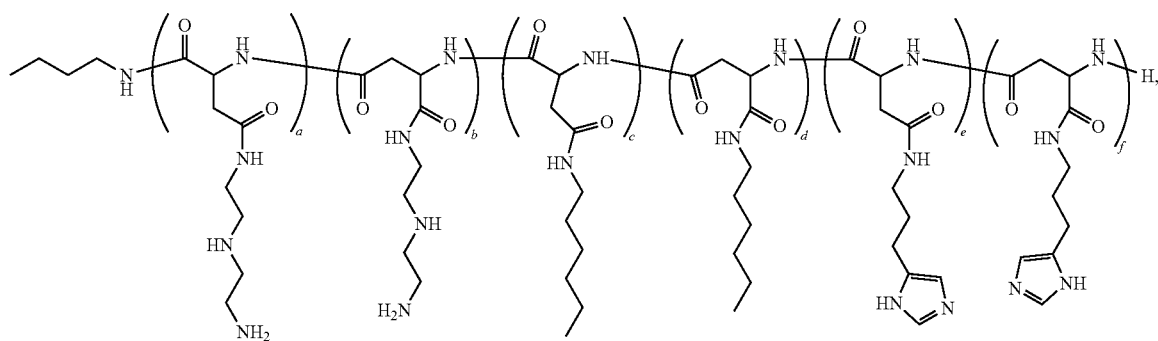
Polymer 59
