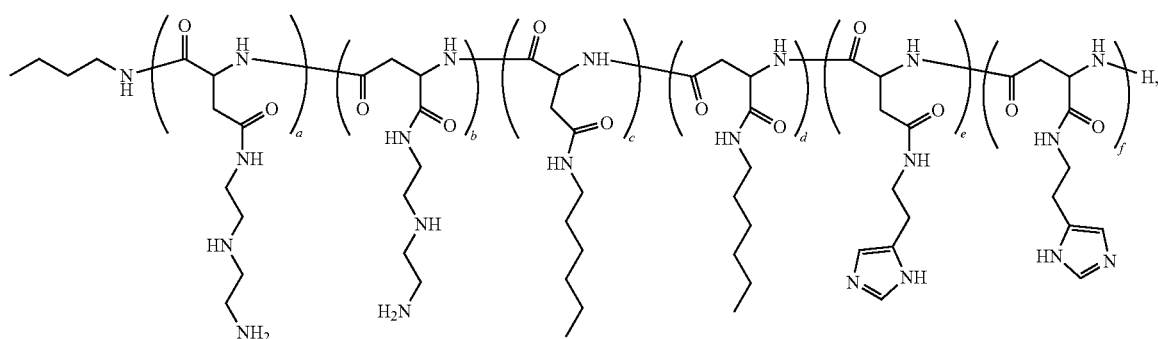
Polymer 52
