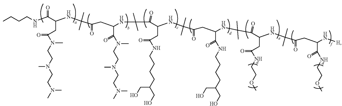
Polymer 86
