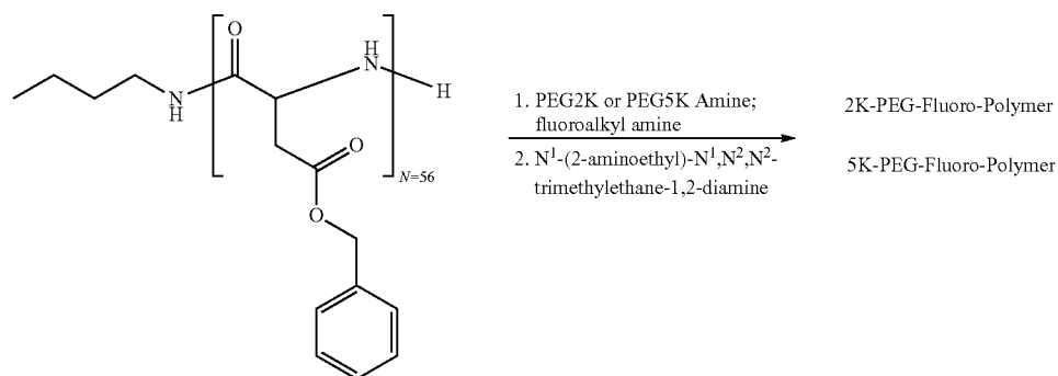
Scheme 6
