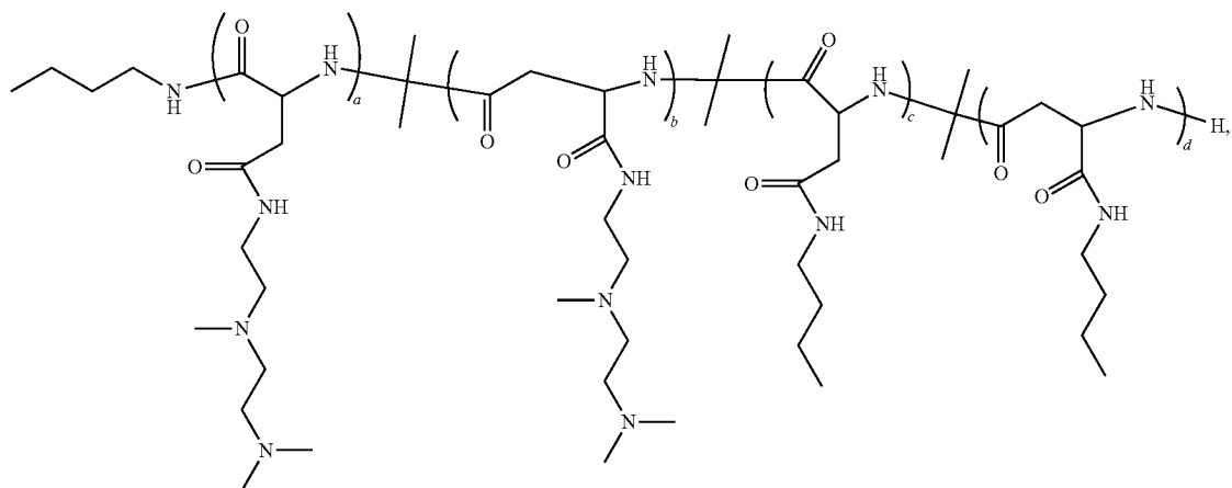
Polymer 27
