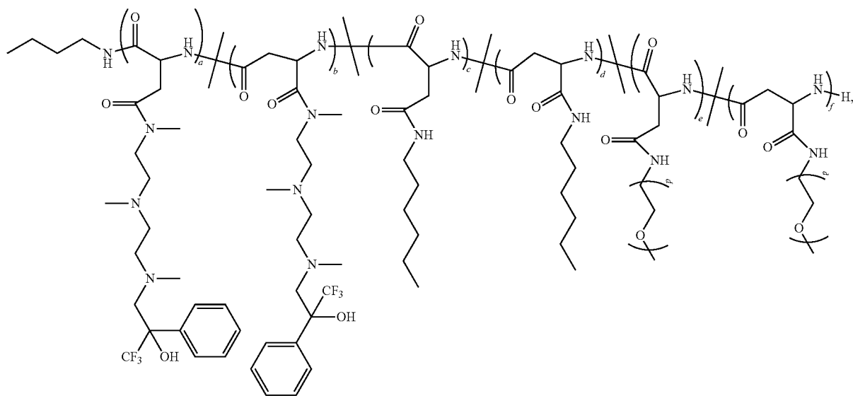
Polymer 84
