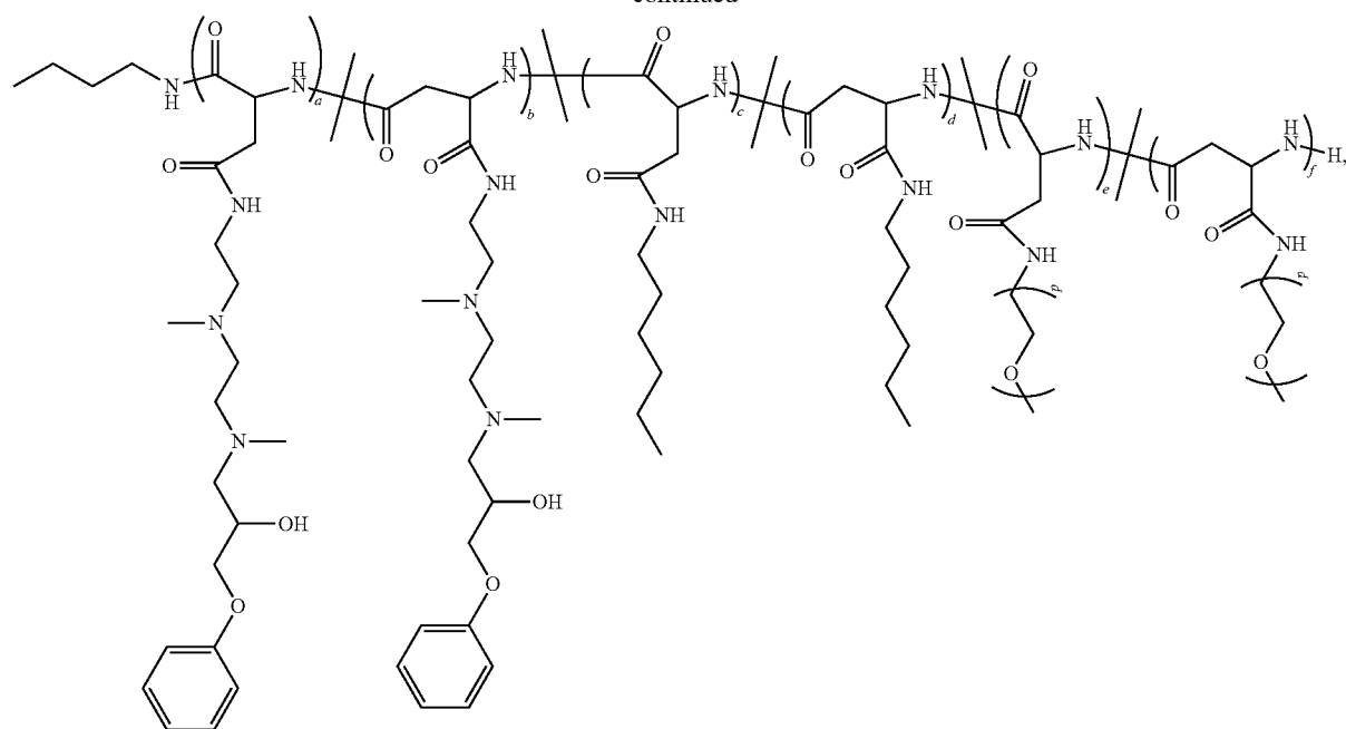
Polymer 77
