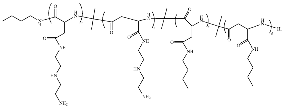
Polymer 11
