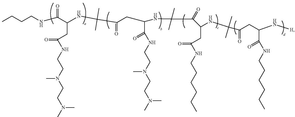
Polymer 29
