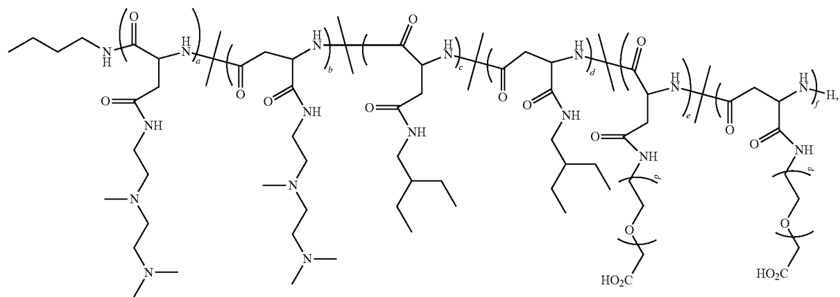
Polymer 79
