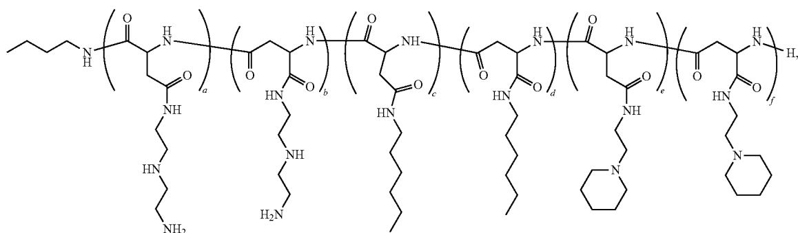
Polymer 48
