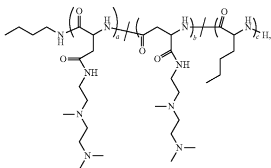
Polymer 23
