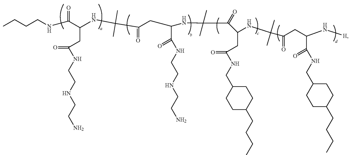
Polymer 15
