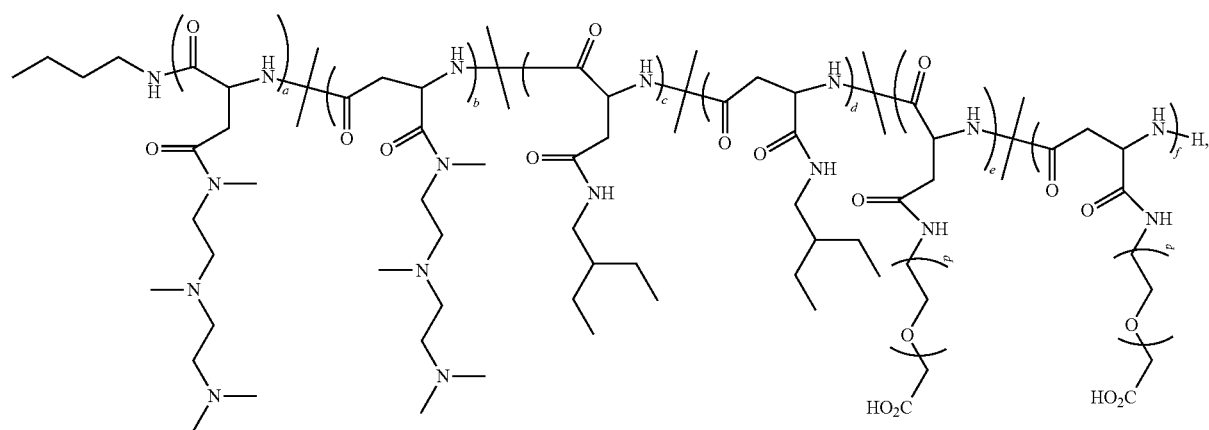
Polymer 87
