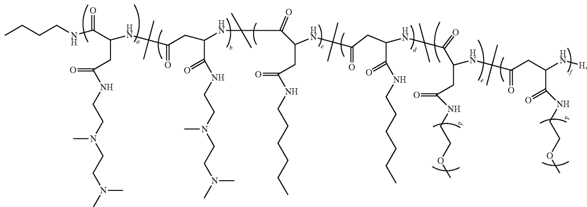
Polymer 72
