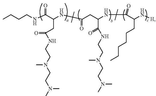
Polymer 17
