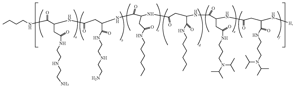
Polymer 55
