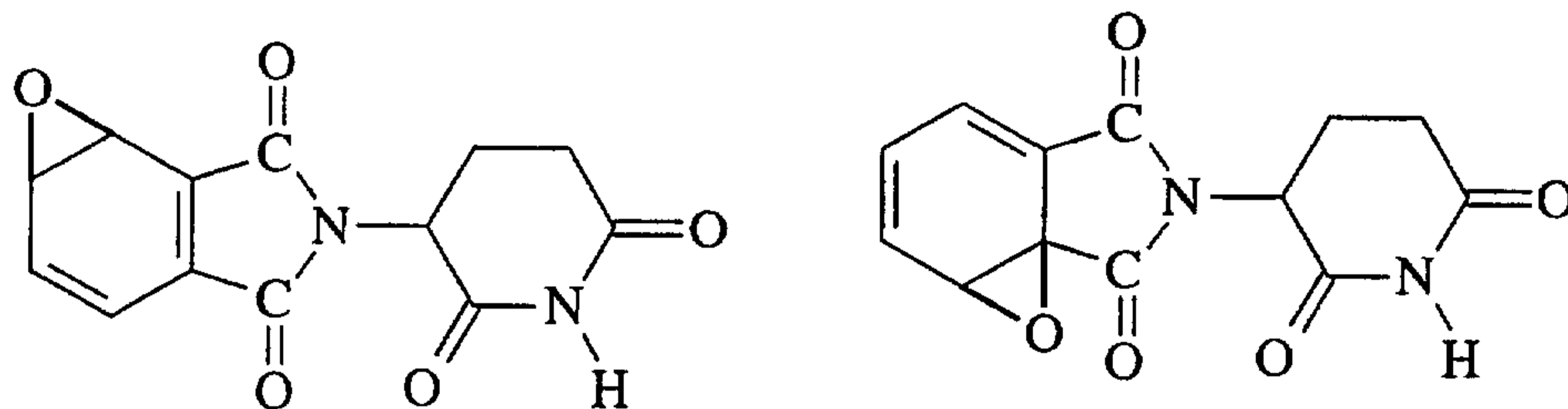
Epoxides of thalidomide
