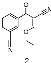
(3-[2-Cyano-2-(Ethoxymethylidene)Acetyl]Benzonitrile)
