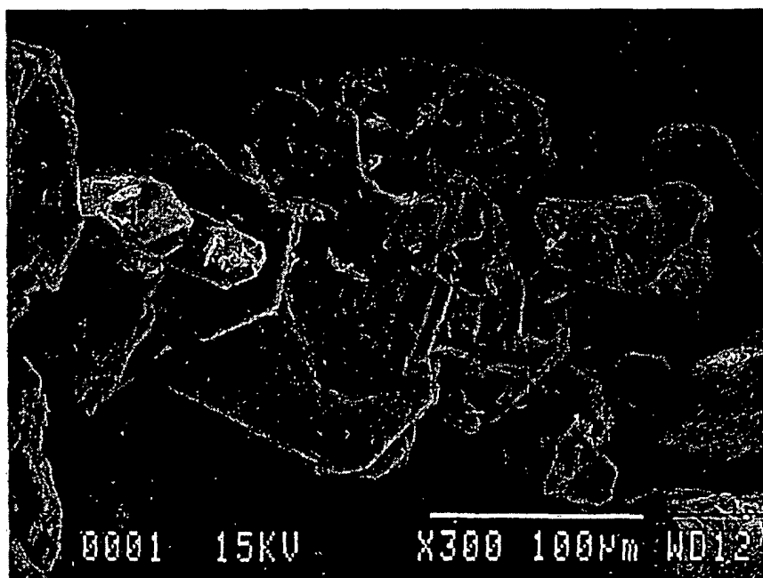
Figure 3: SEM image illustrating the plate like habit of the crystals of Form I:
