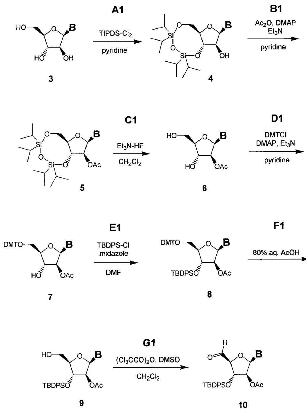
Scheme I: Synthesis of 1 ( R=CH_3 ) from aranucleoside
