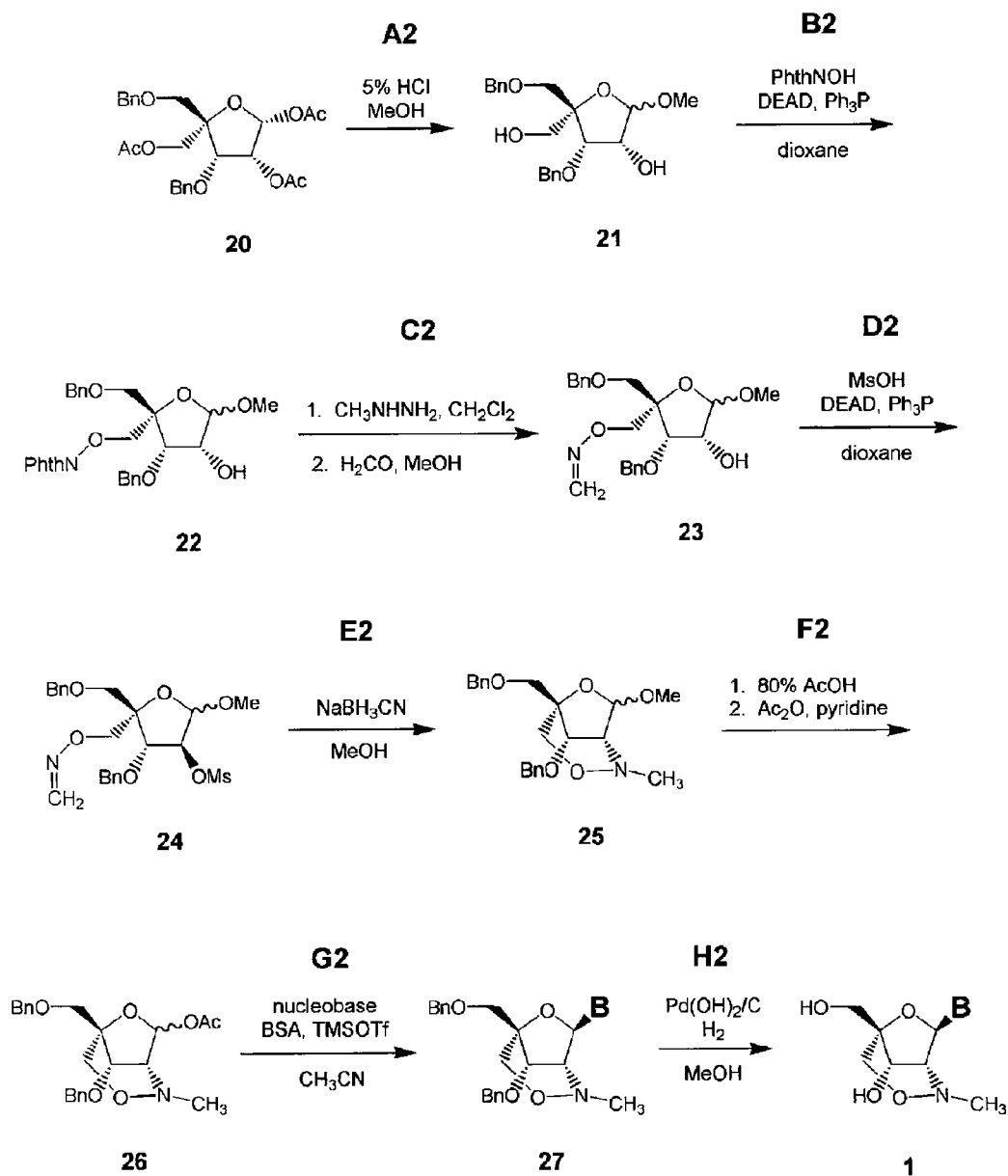
Scheme II: Synthesis of 1 ( R = CH_3 ) from protected 4-C-hydroxymethylribose
