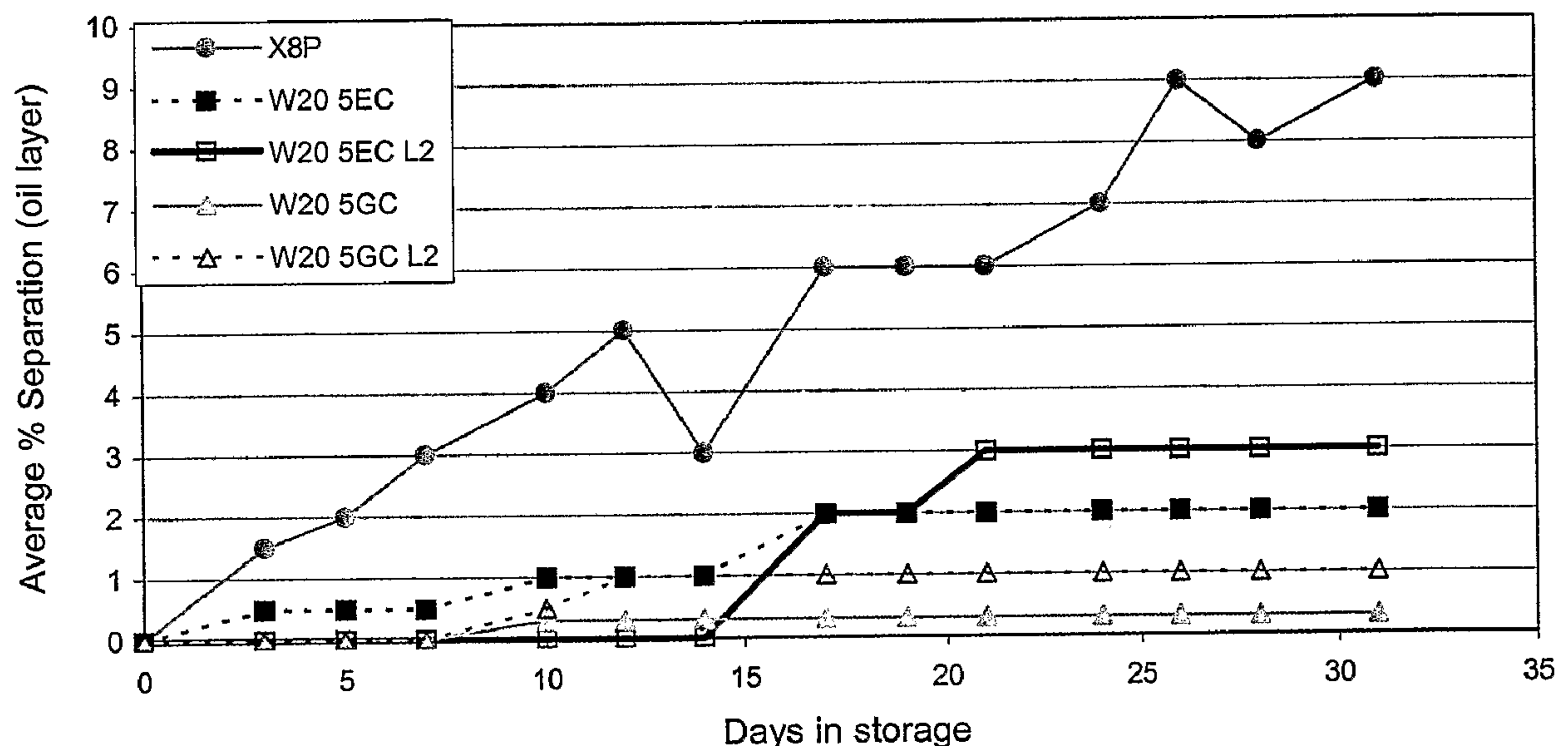
Average separation for neat emulsions stored at 55 °C
