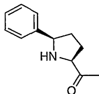
(2S,5R)-5-Phenyl- pyrrolidine-2-carbonyl
