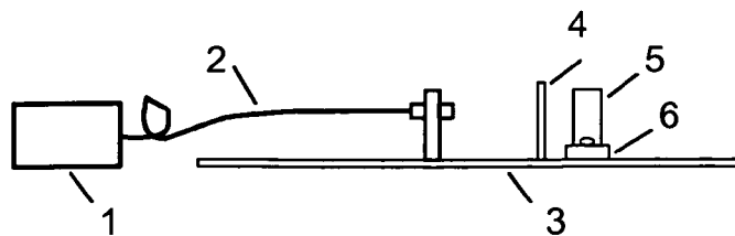
Figure 1: Set-up for irradiation of the samples. 1: metal halide lamp (Macam Flexicure), 2: liquid light guide, 3: optical bench, 4: cut-off filter, translucent for \lambda > 290 nm, 5: closed cuvette with UV-absorber solution, 6: magnetic stirrer
