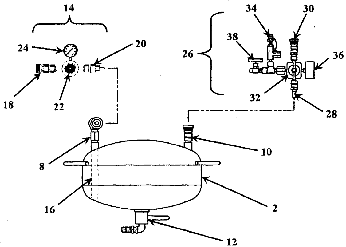
FIG. 2 (PRIOR ART)
