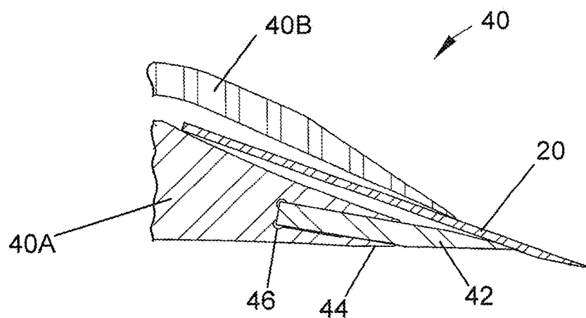
FIG. 5 PRIOR ART
