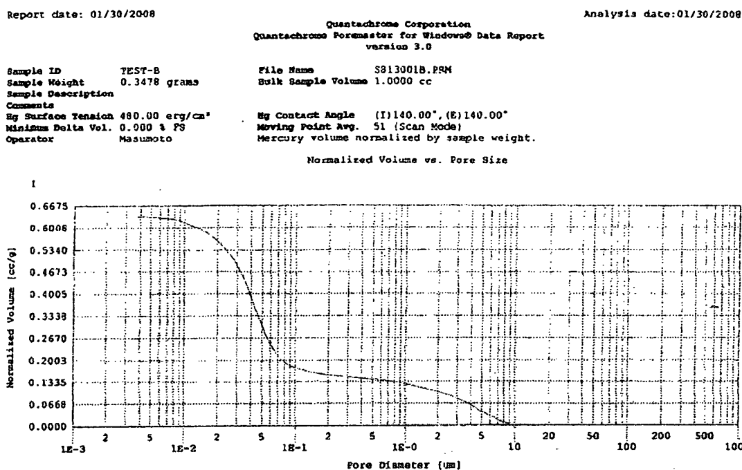
FIG. 1 shows the measurement results of the total pore volume of the cerium-zirconium based compound oxide obtained in Example 1 (Fresh) of the present invention.
