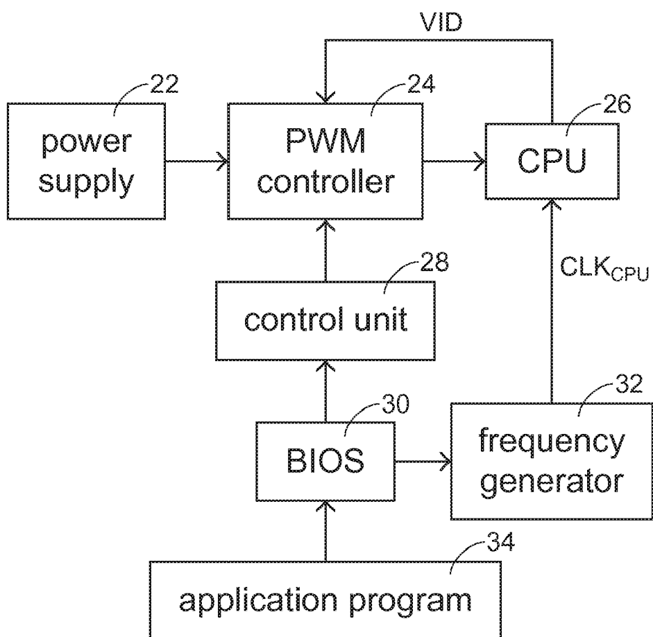
FIG.2 PRIOR ART
