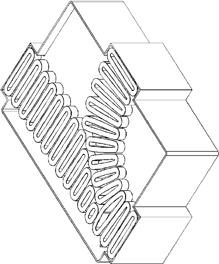
Figure 12. Cutaway view of right diverge showing coils for continuous propulsion
