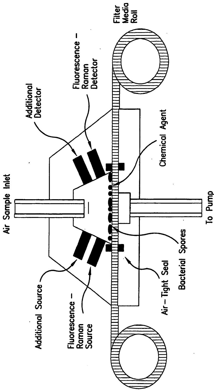
The Integrated Detector Sample Cell FIG.1
