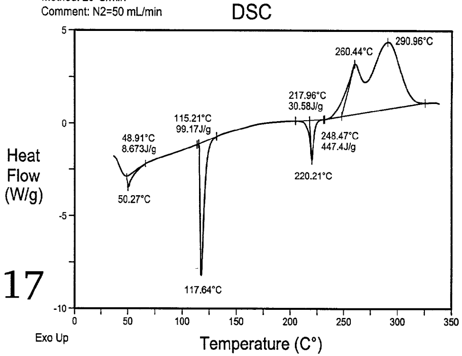
DSC thermogram of 2,3-dimethyl-2,3-dinitrobutane, sample weight is 0.184 mg
