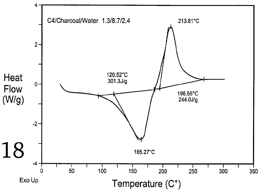
DSC thermogram of C4/Water/Charcoal, sample weight is 12.3 mg
