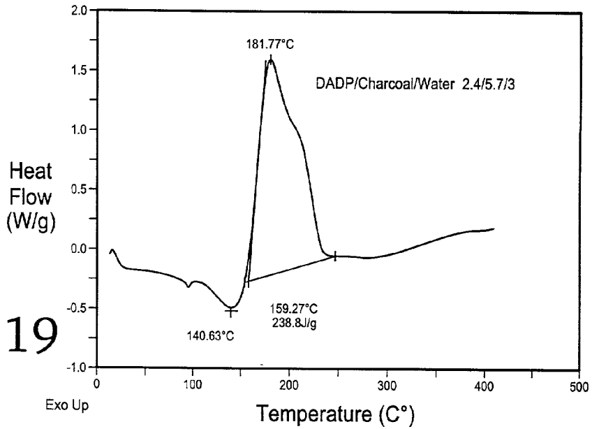
DSC thermogram of DADP/Water/Charcoal, sample weight is 11.1 mg
