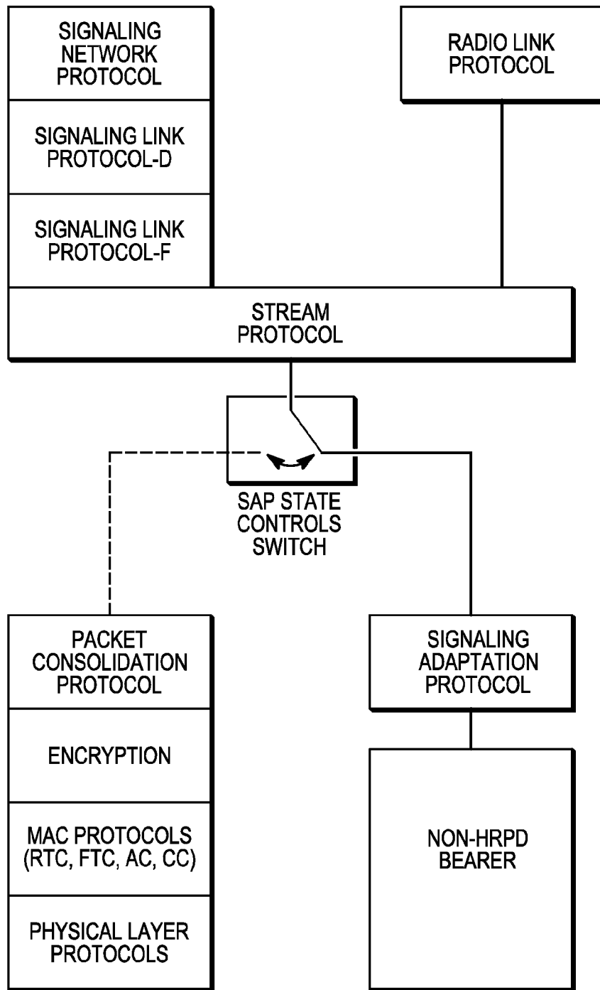
OPTION-3 SIGNALING ADAPTATION PROTOCOL CARRYING STREAM PACKETS
