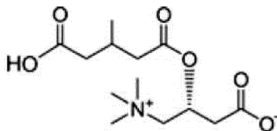
3Me-glutaryl carnitine (S192)
