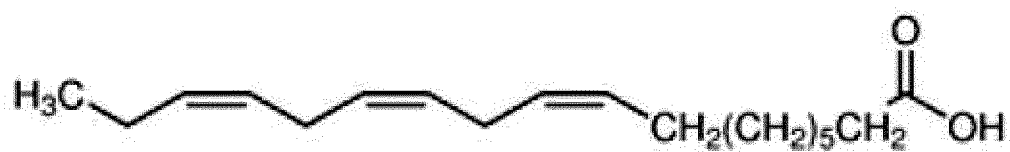
\alpha -linolenic acid (S69)
