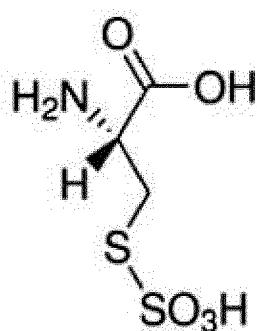
L-cysteine S-sulfate (S153)
