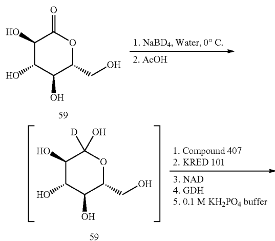
Scheme 19. Preparation of Compound 437(S).
