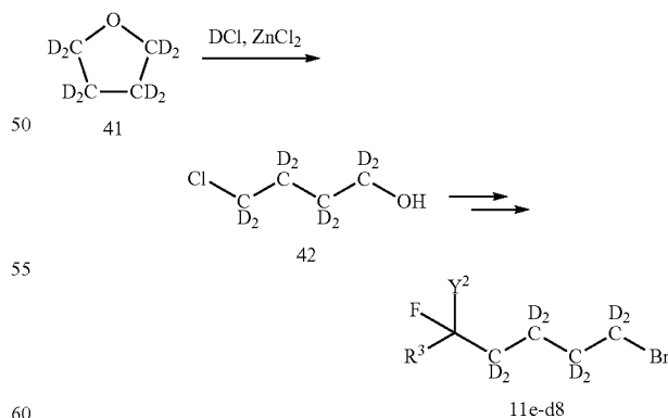
Scheme 8. Synthesis of Intermediate 11e-d 8 (X=Br)
