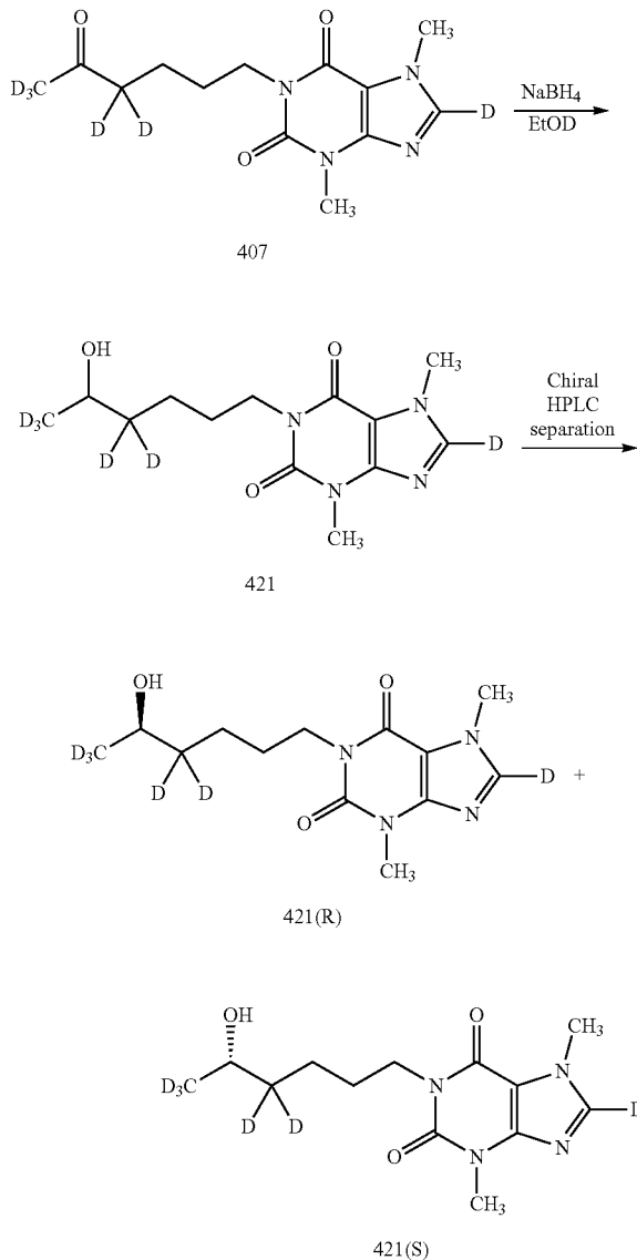
Scheme 21. Preparation of Compounds 421, 421(R) and 421(S).
