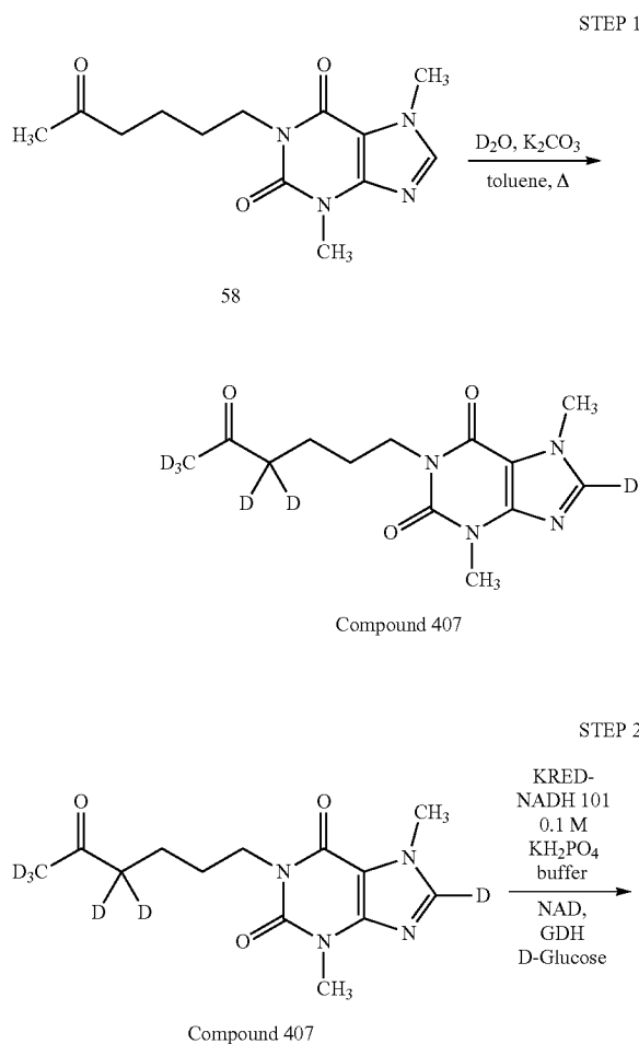
Scheme 24: Alternative Preparation of S-1-(4,4,6,6,6-d 5 -5-Hydroxyhexyl)-3,7-dimethyl-1H-purine-2,6(3H,7H)-dione (Compound 121(S)).
