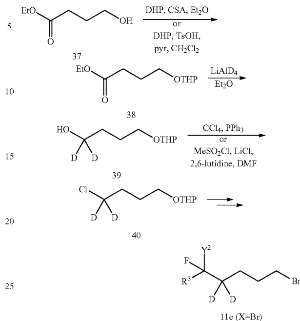
Scheme 7. Alternative Synthesis of Intermediate 11e (X=Br)
