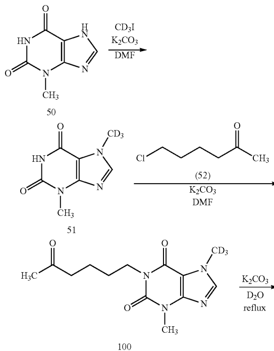
Scheme 13. Preparation of Compounds 100 and 409.
