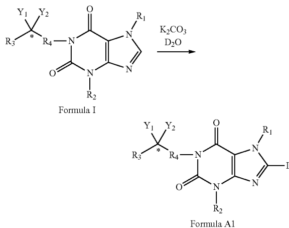
Scheme 11. Synthesis of Compounds of Formula A1
