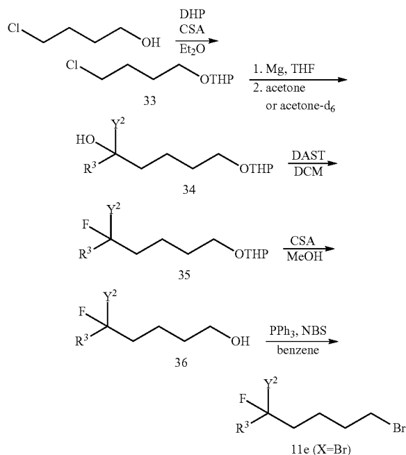
Scheme 6. Synthesis of Intermediate 11e (X=Br)
