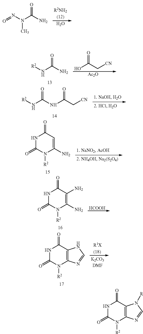
Scheme 2. Synthesis of Compound 10
