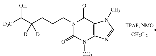
Scheme 25. Preparation of Compound 107.
