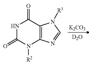
Scheme 12. Alternative Synthesis of Compounds of Formula A1
