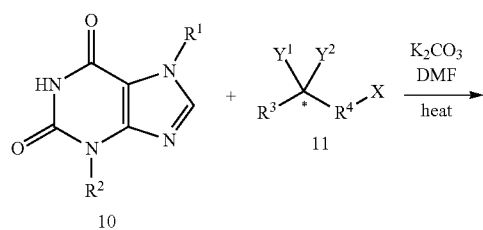
Scheme 1A. Synthesis of Compounds of Formula I
