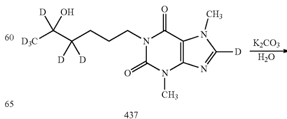
Scheme 22. Preparation of Compound 137.
