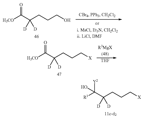
Scheme 10. Synthesis of Intermediate 11c-d 2 .
