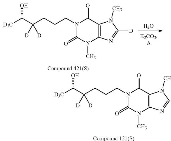
Scheme 24: Alternative Preparation of S-1-(4,4,6,6,6-d 5 -5-Hydroxyhexyl)-3,7-dimethyl-1H-purine-2,6(3H,7H)-dione (Compound 121(S)).
