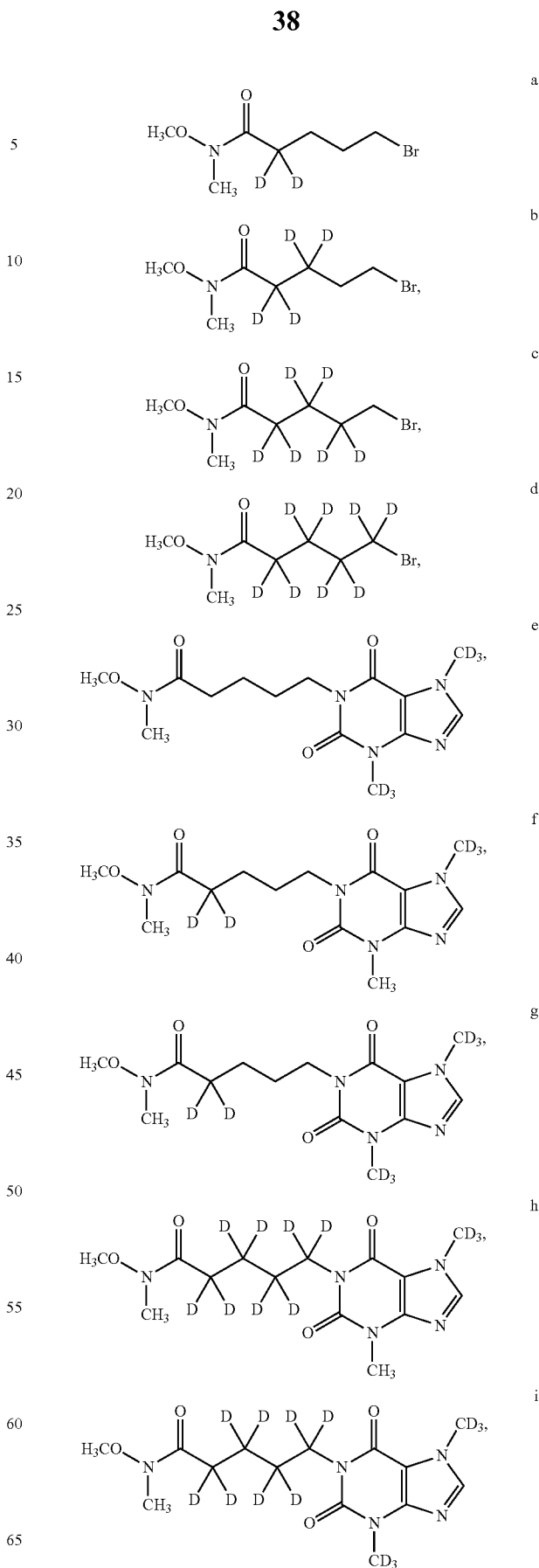
Scheme 12b. Alternative Synthesis of Compounds of Formula I.
