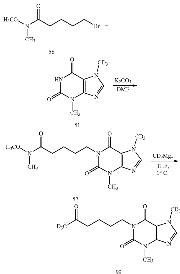
Scheme 15. Preparation of Compound 99.
