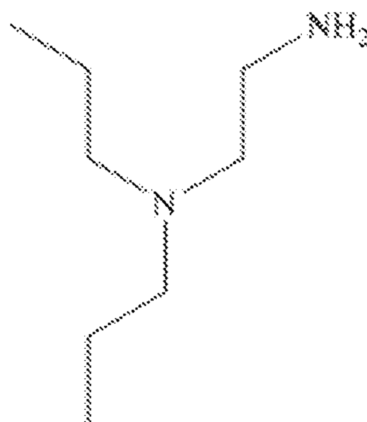
N,N'-dipropylpropane 1,3 diamine
