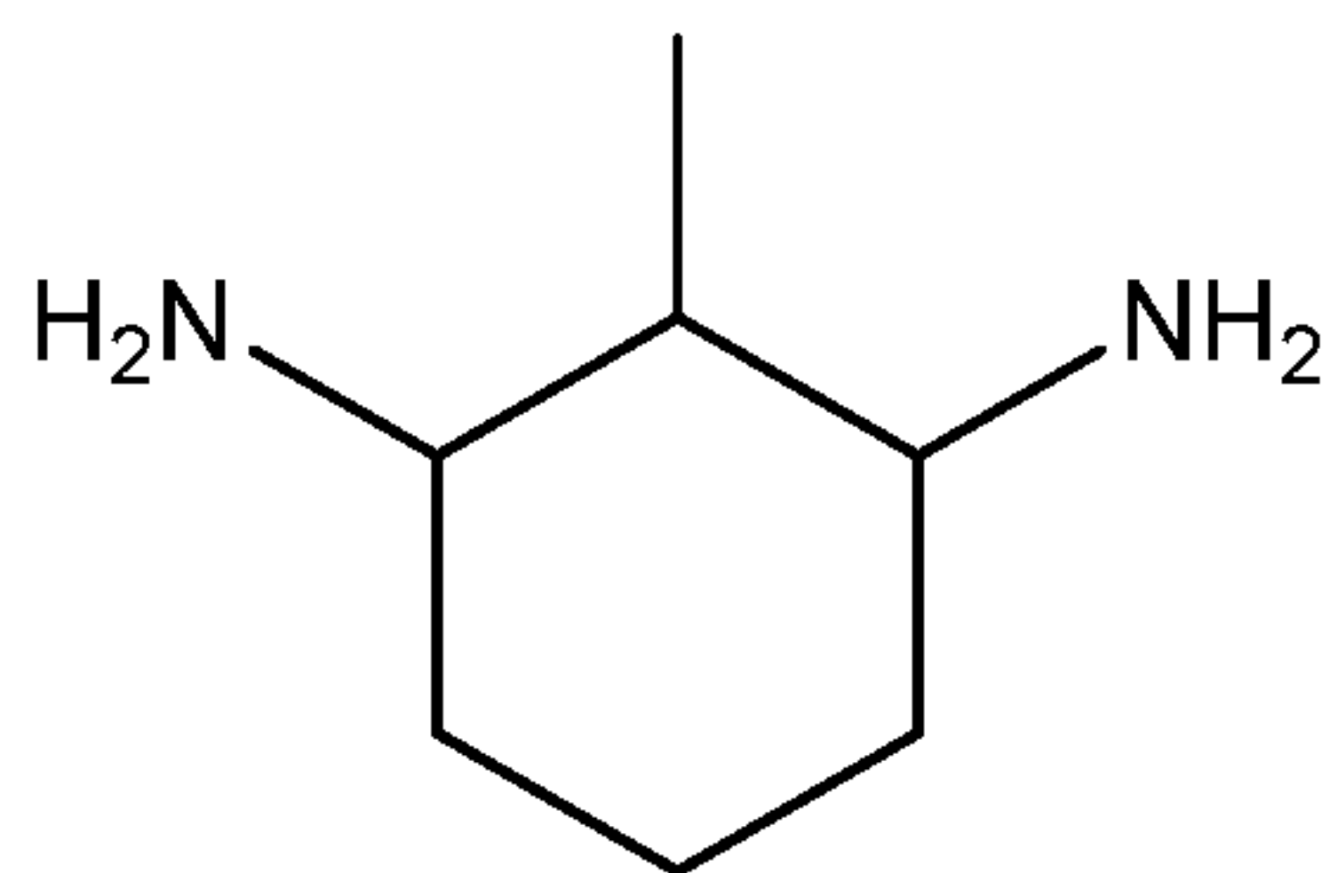
2-methylcyclohexane-1,3-diamine,
