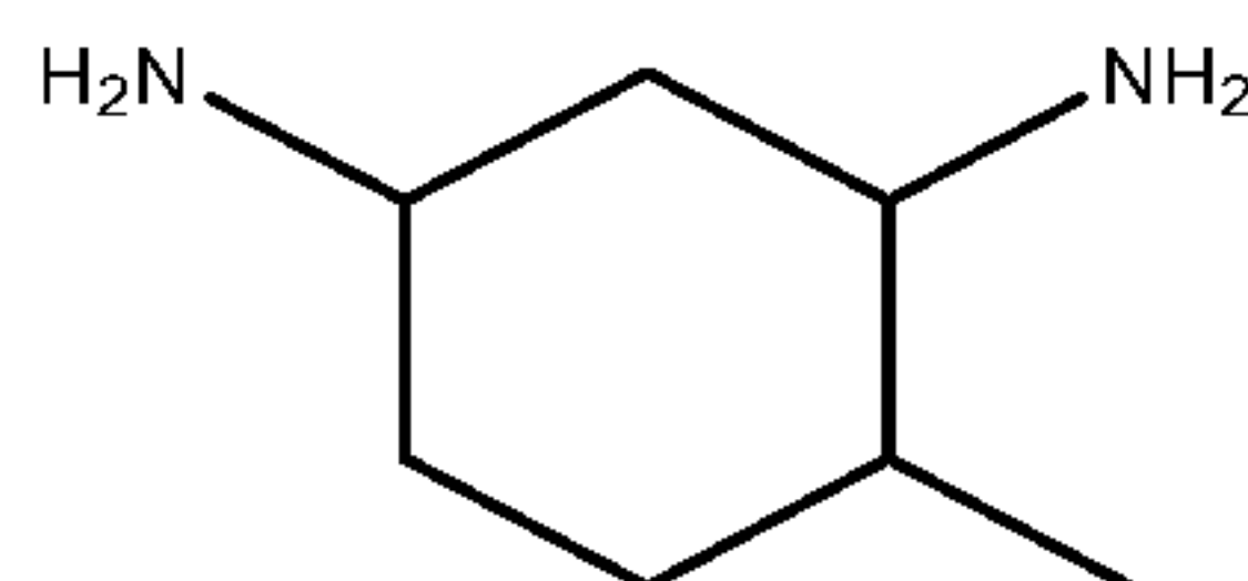
4-methylcyclohexane-1,3-diamine,
