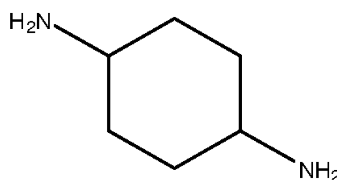
Cyclohexane-1,4-diamine,
