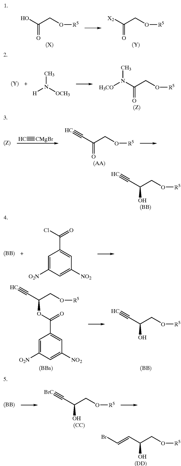
REACTION SCHEME 6
