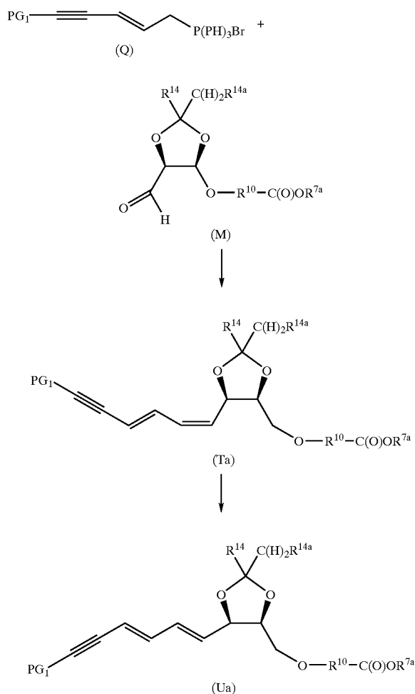
REACTION SCHEME 5
