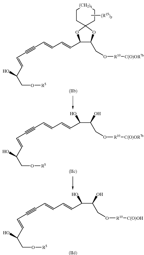
REACTION SCHEME 9
