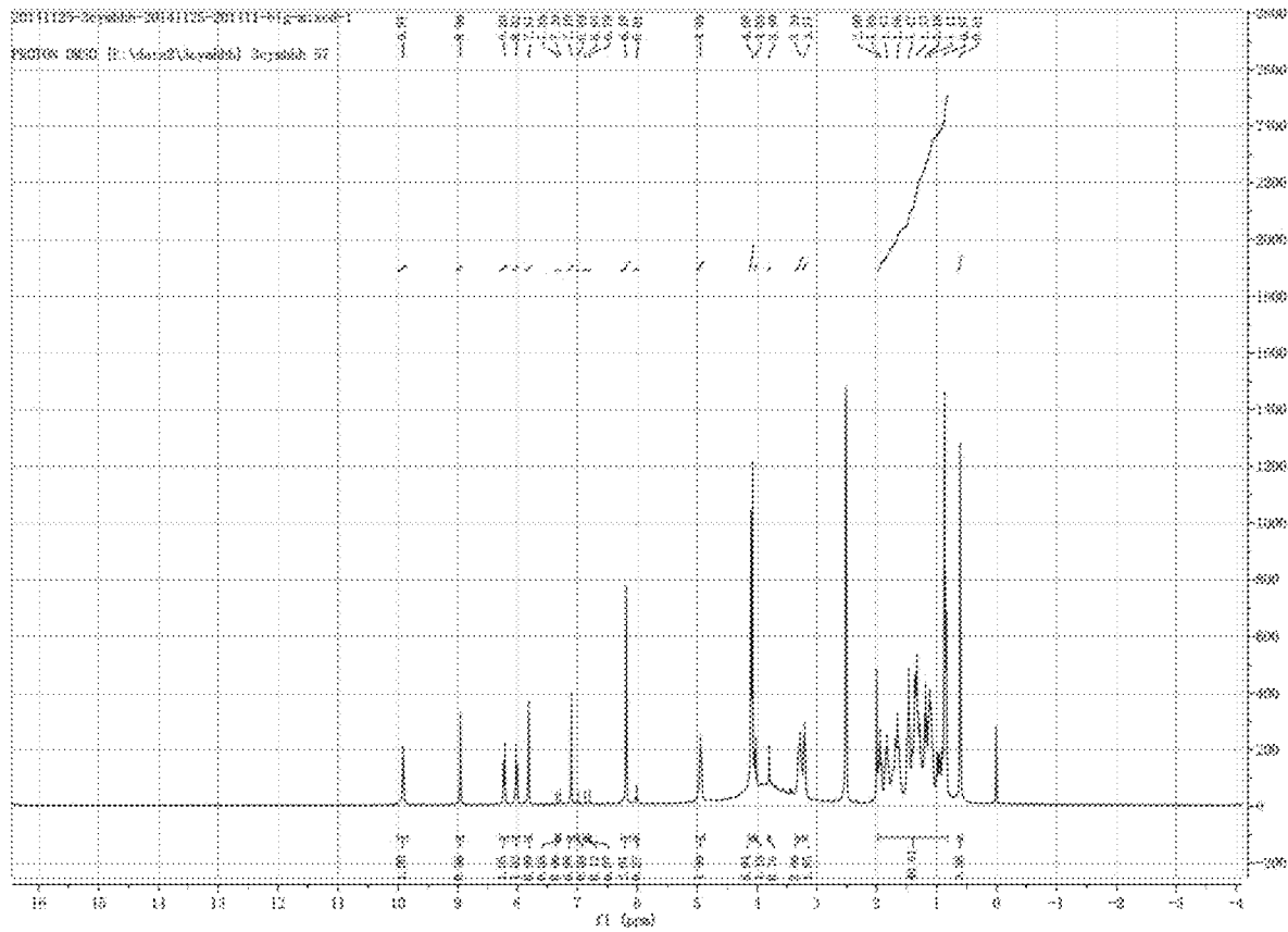
FIG. 7. 1 H NMR of berberine ursodeoxycholate (purified product).
