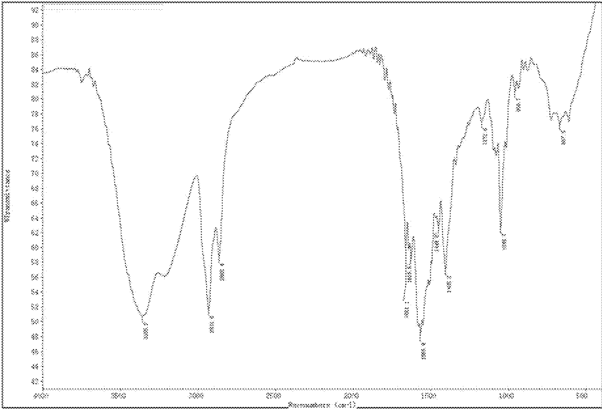
FIG. 6. IR spectrum of metformin ursodeoxycholate.
