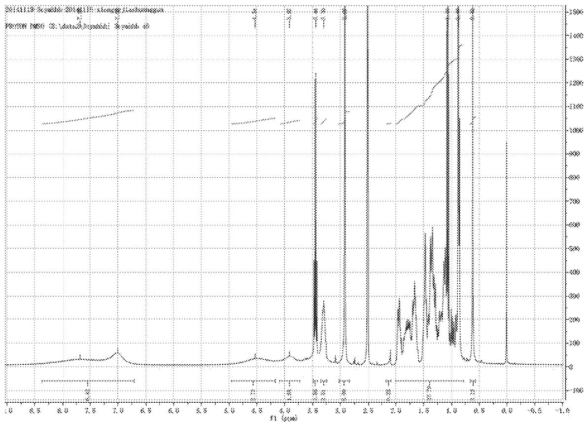
FIG. 5. 1 H NMR of metformin ursodeoxycholate in DMSO-D6.
