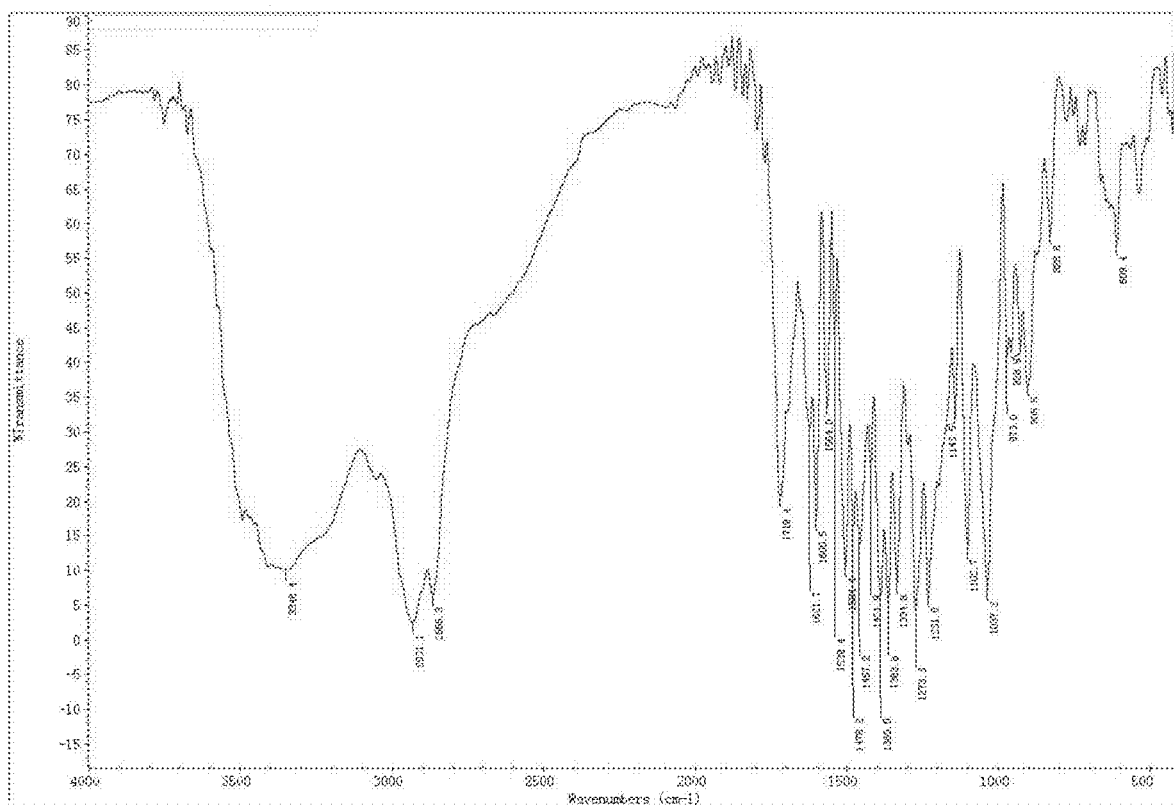
FIG. 10. IR spectrum of mixture of berberine hydrochloride (1.0 equiv.) and ursodeoxycholic acid (1.0 equiv.). The carbonyl stretching vibration band C=O of ursodeoxycholic acid appears at about 1719 cm -1 .
