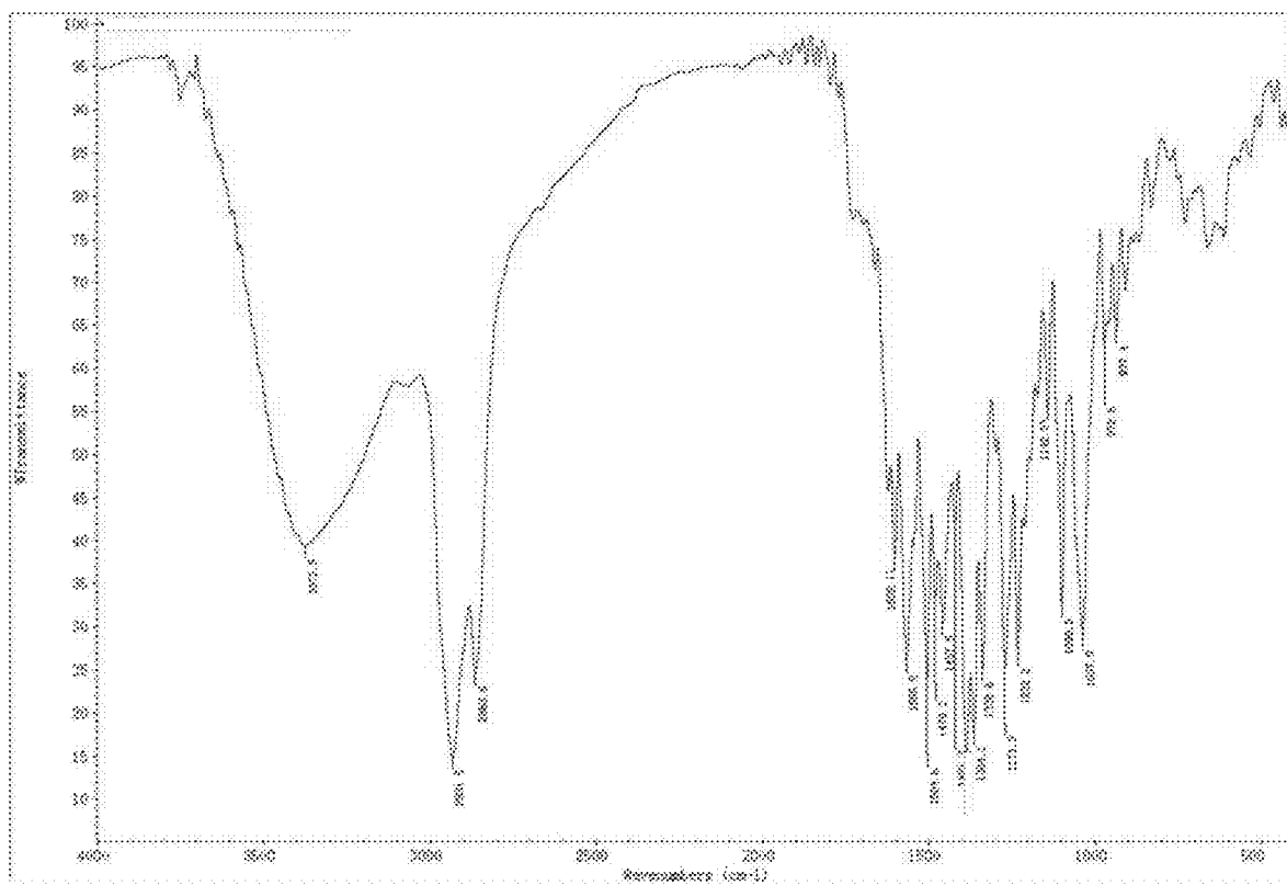
FIG. 9. IR spectrum of berberine ursodeoxycholate (crude product).
