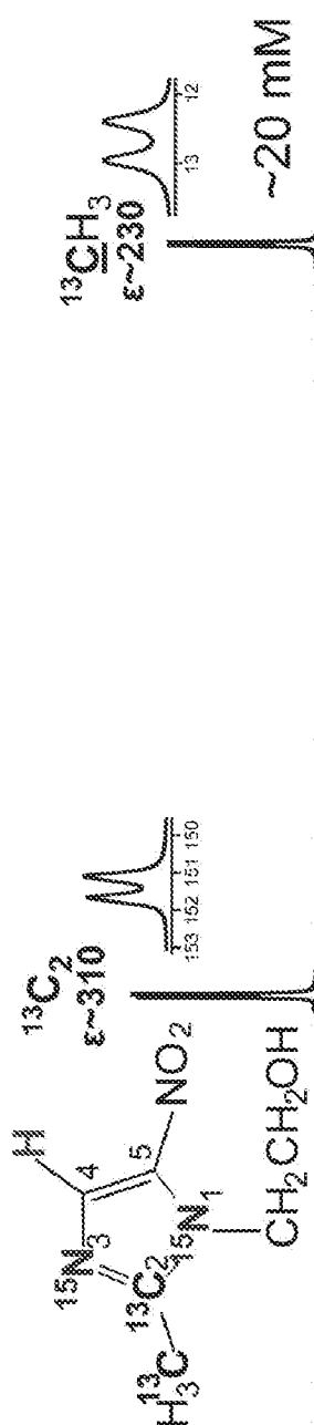
FIG. 16C 13 C SABRE-SHEATH
