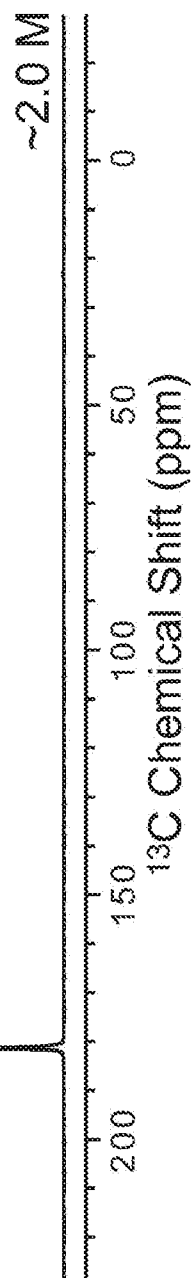
FIG. 16D 13 C Thermally polarized sodium acetate-1- 13 C
