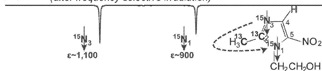
Re-hyperpolarization via MFC to the Earth's field w/o para- \text{H}_2 FIG. 19B (after frequency selective irradiation)
