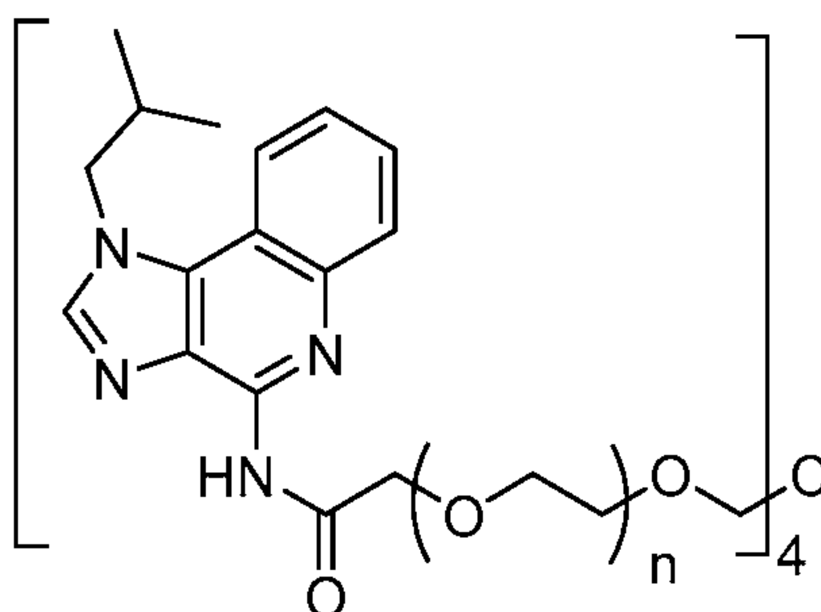
Compound 15
