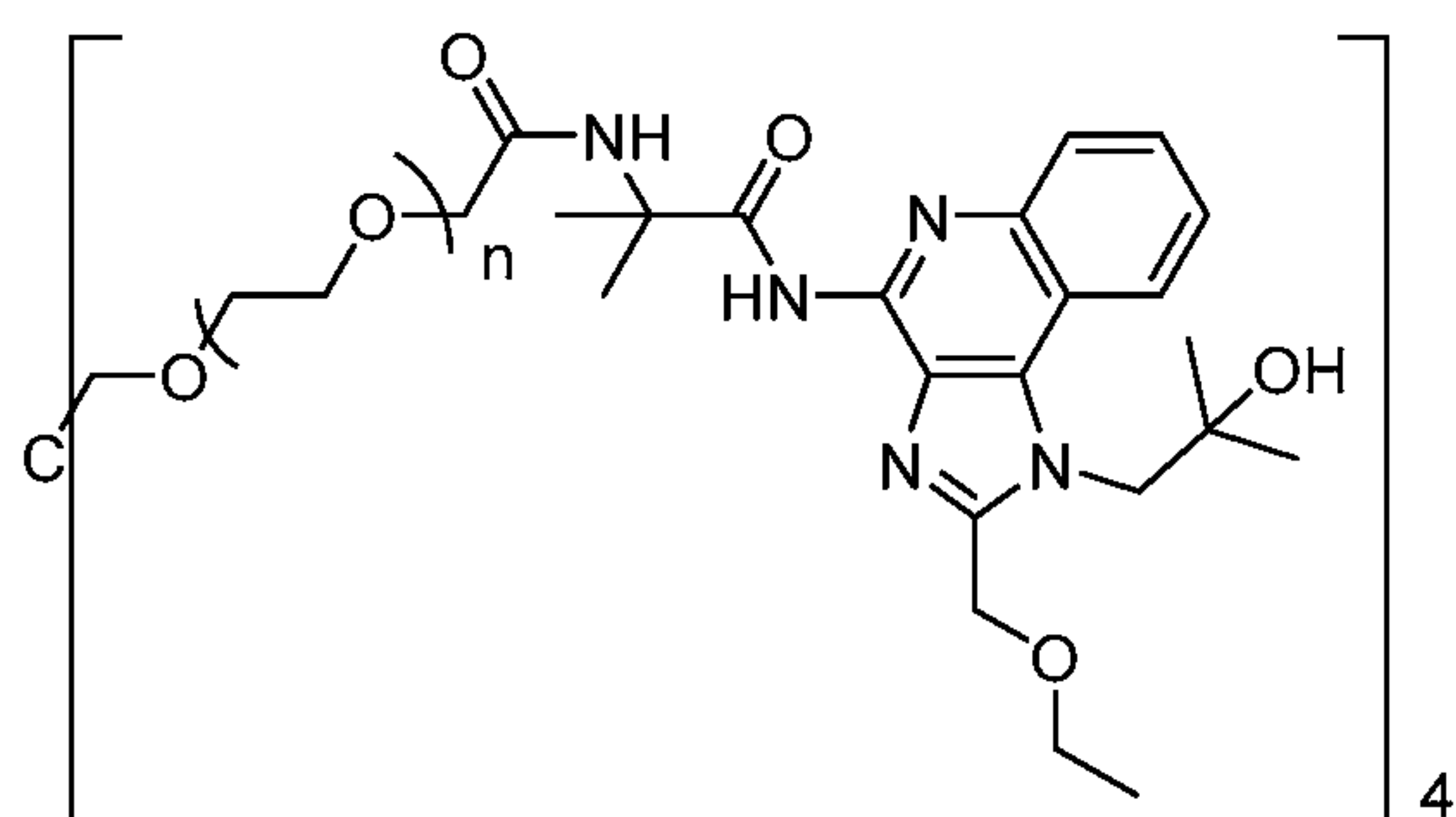
Compound 10
