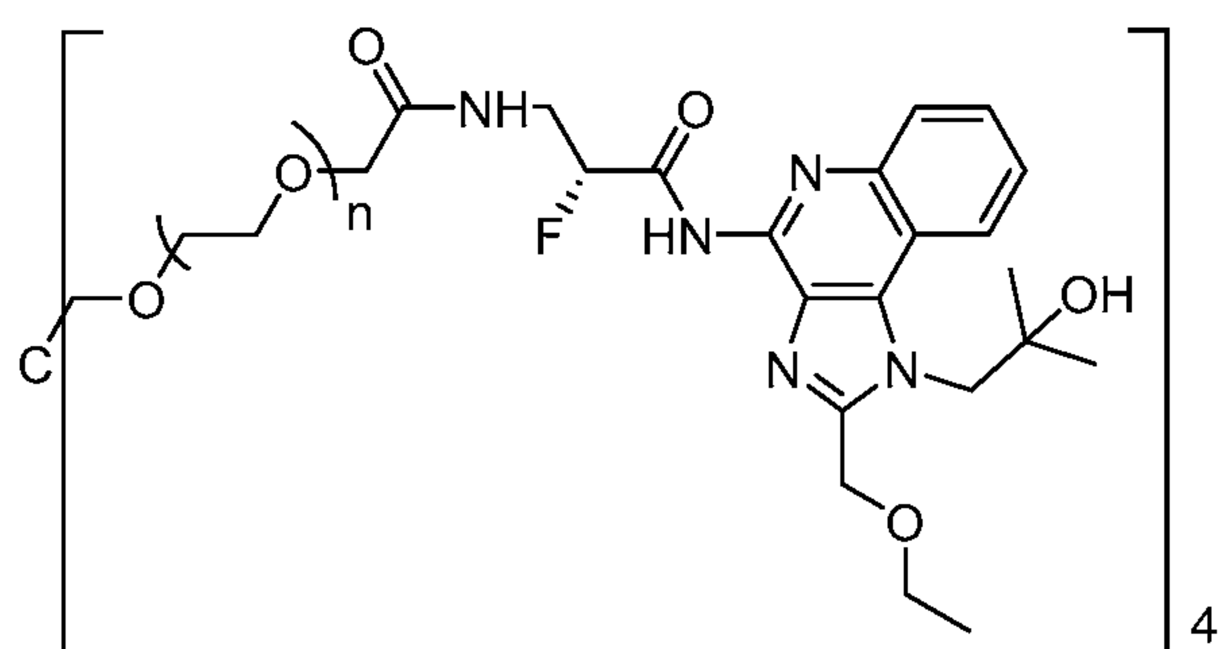
Compound 4
