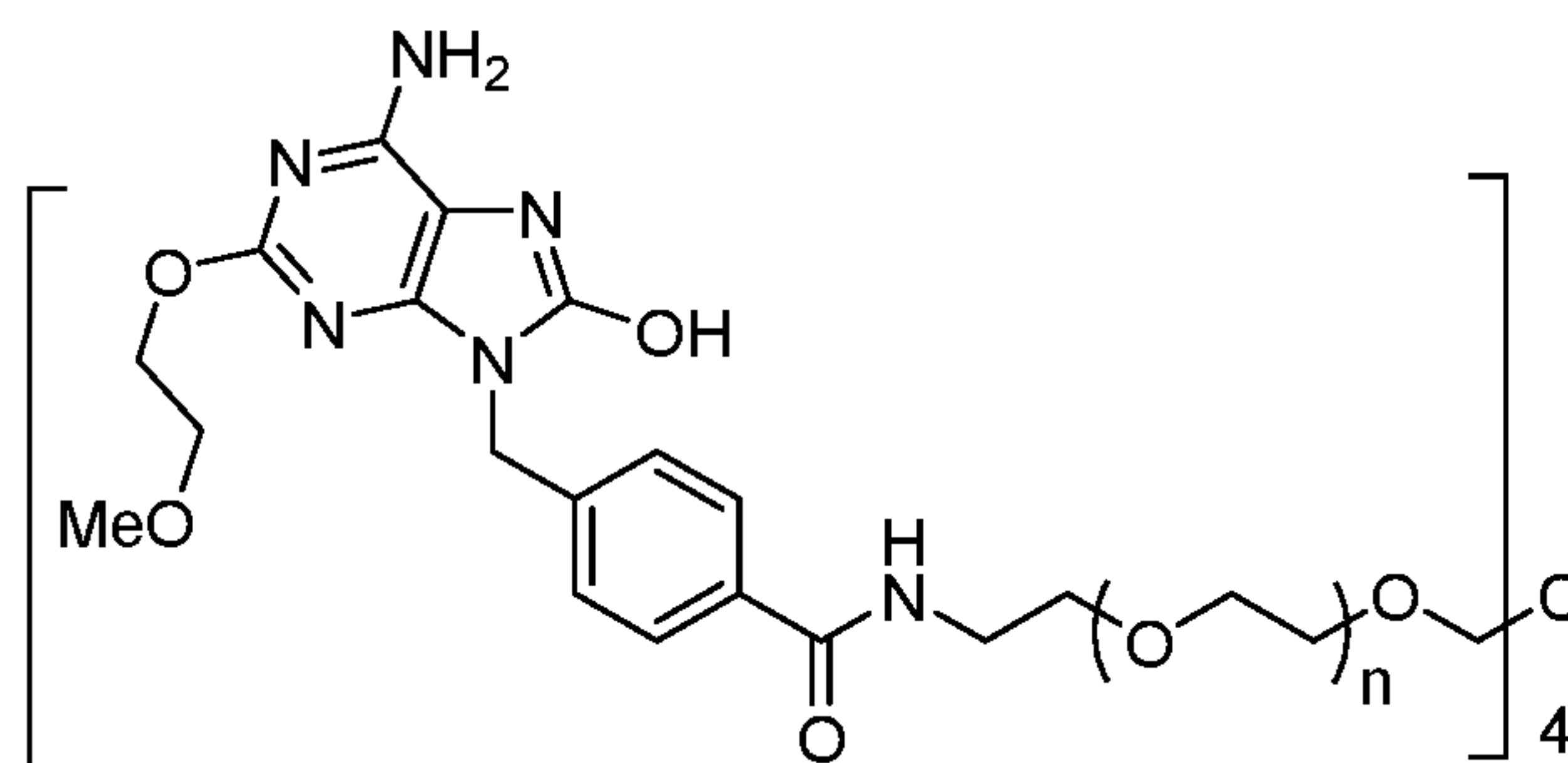
Compound 16
