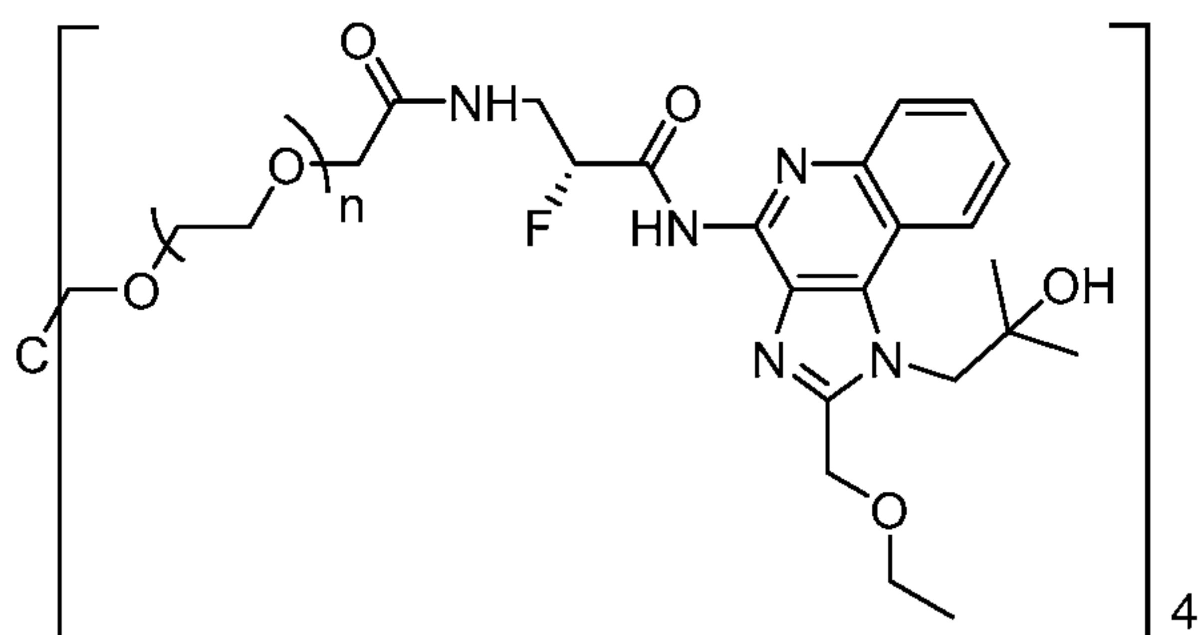
Compound 4
