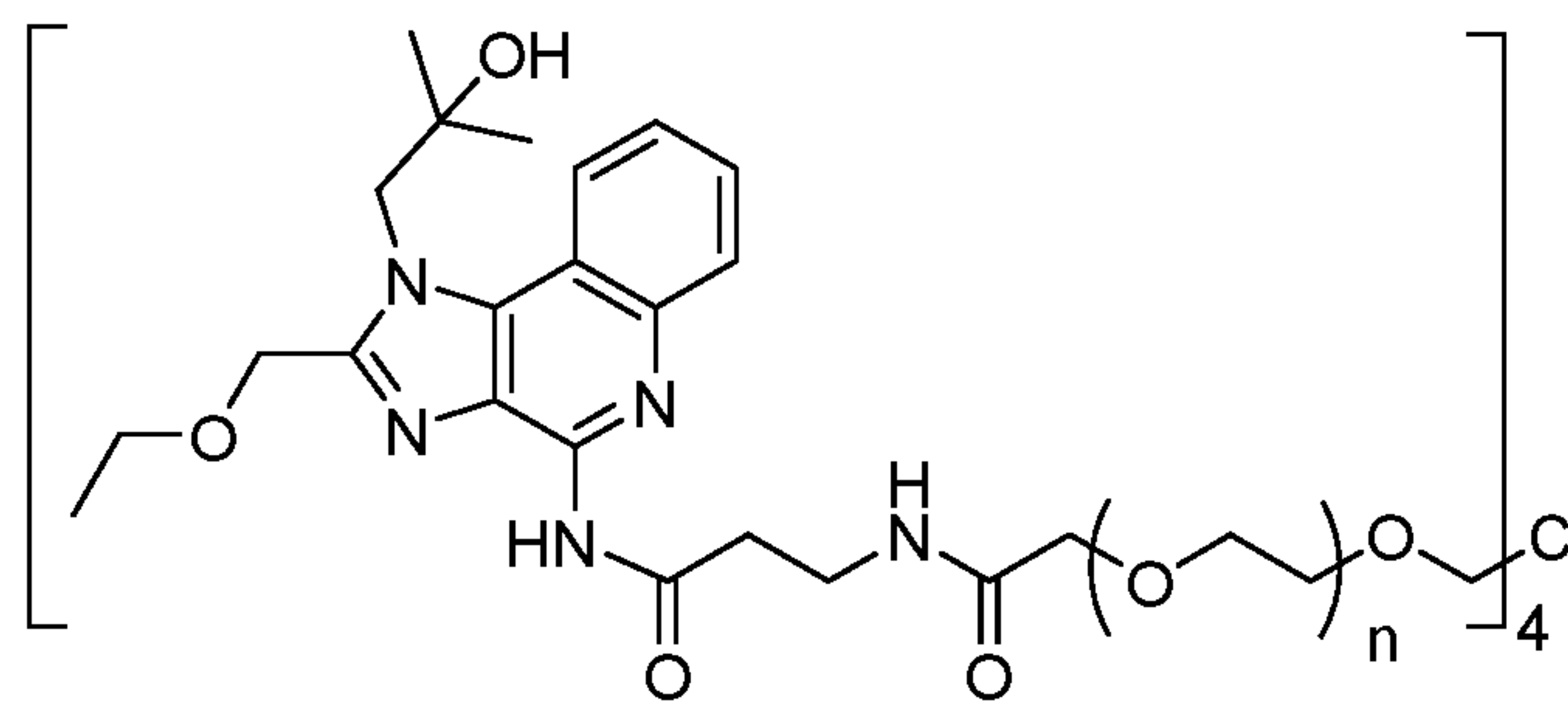
Compound 2
