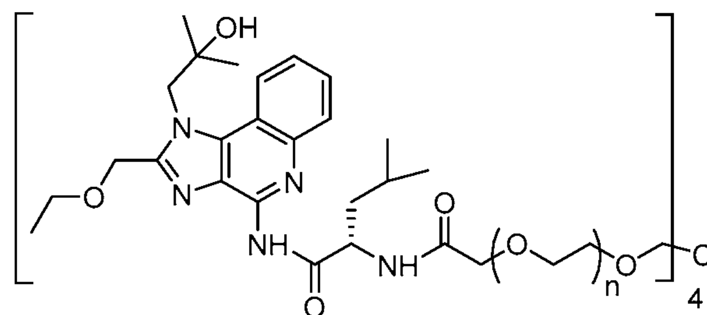
Compound 9
