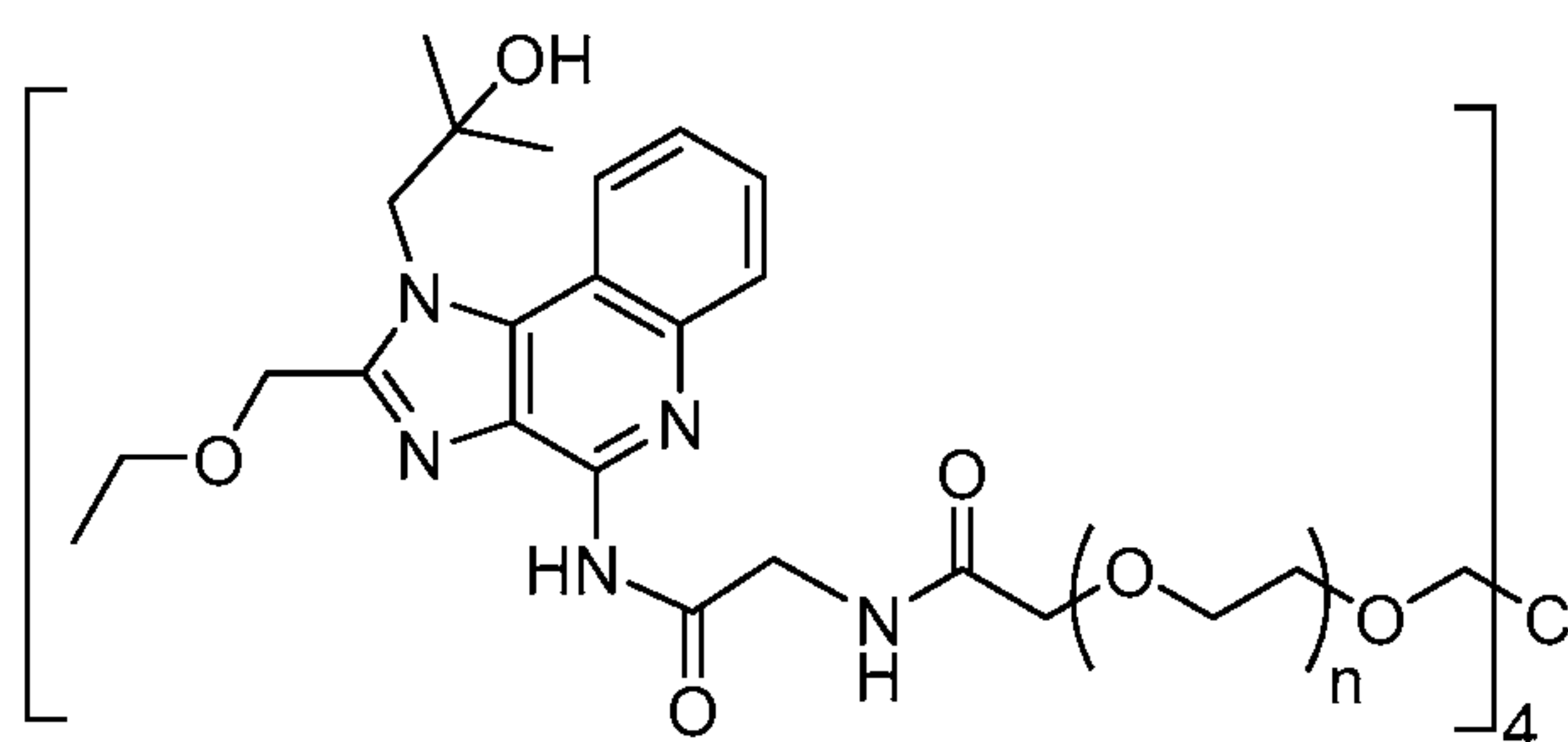
Compound 6
