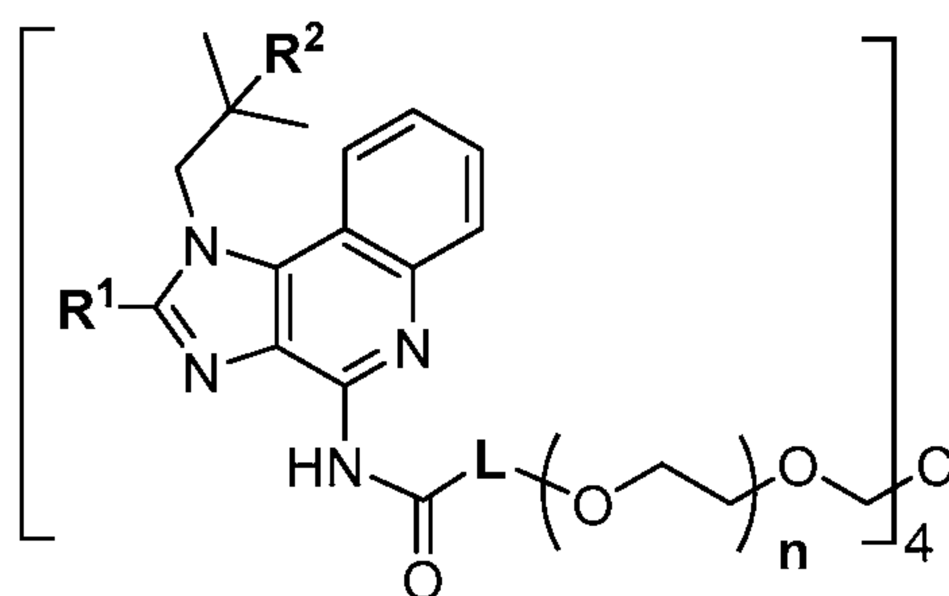
(Formula III)
