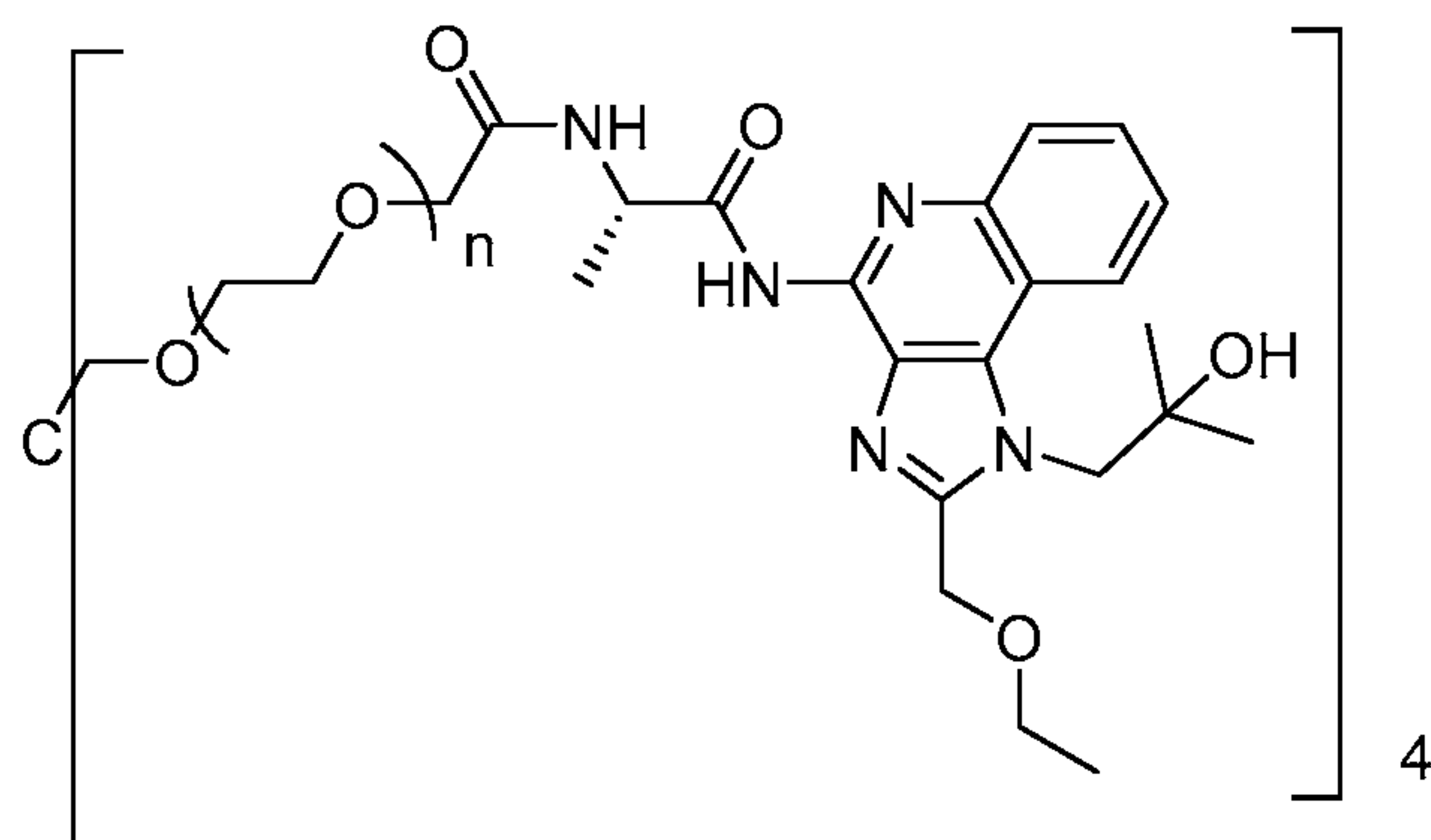
Compound 7
