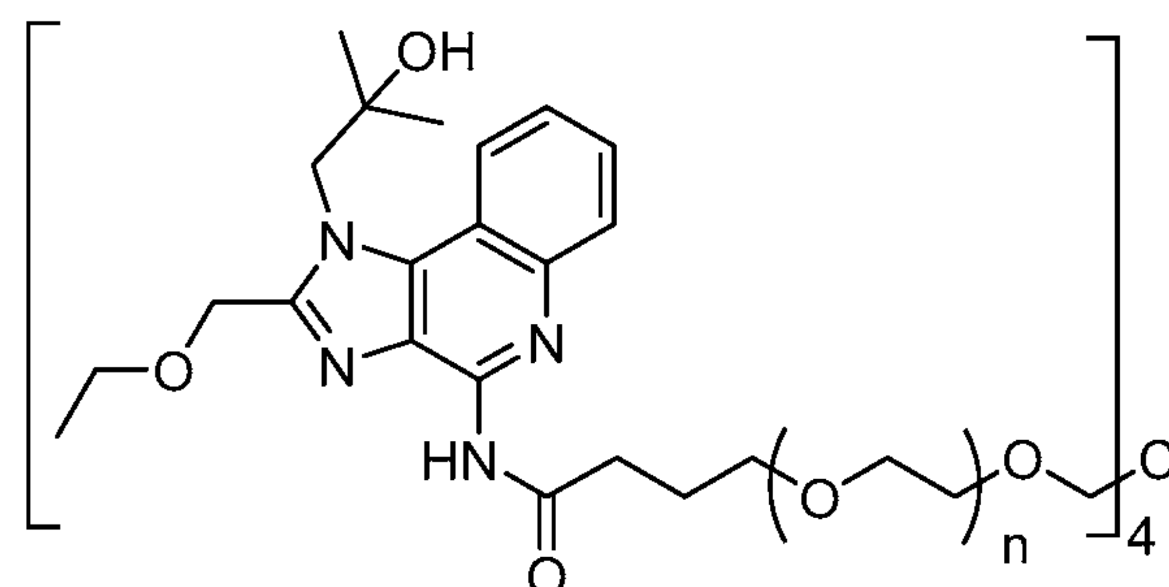
Compound 3
