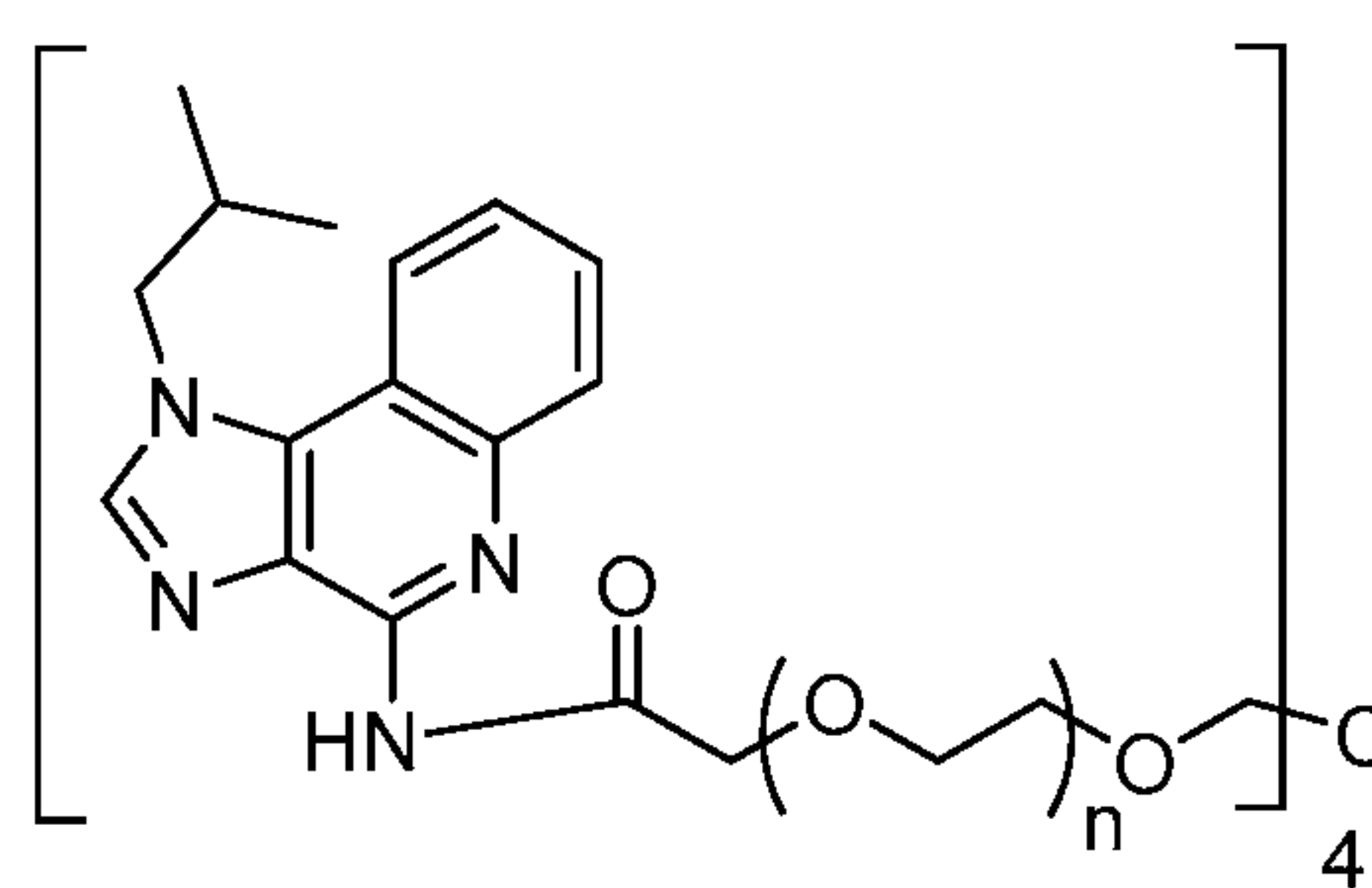
Compound 14
