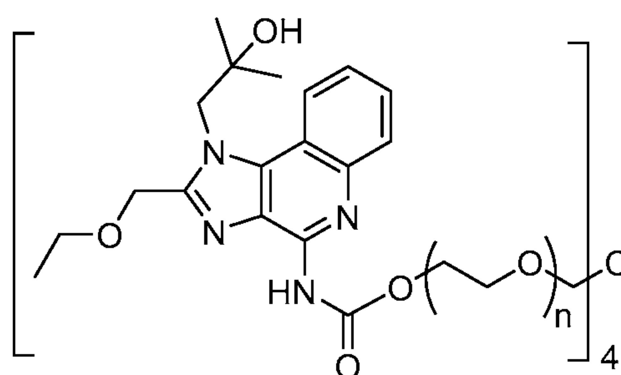
Compound 12
