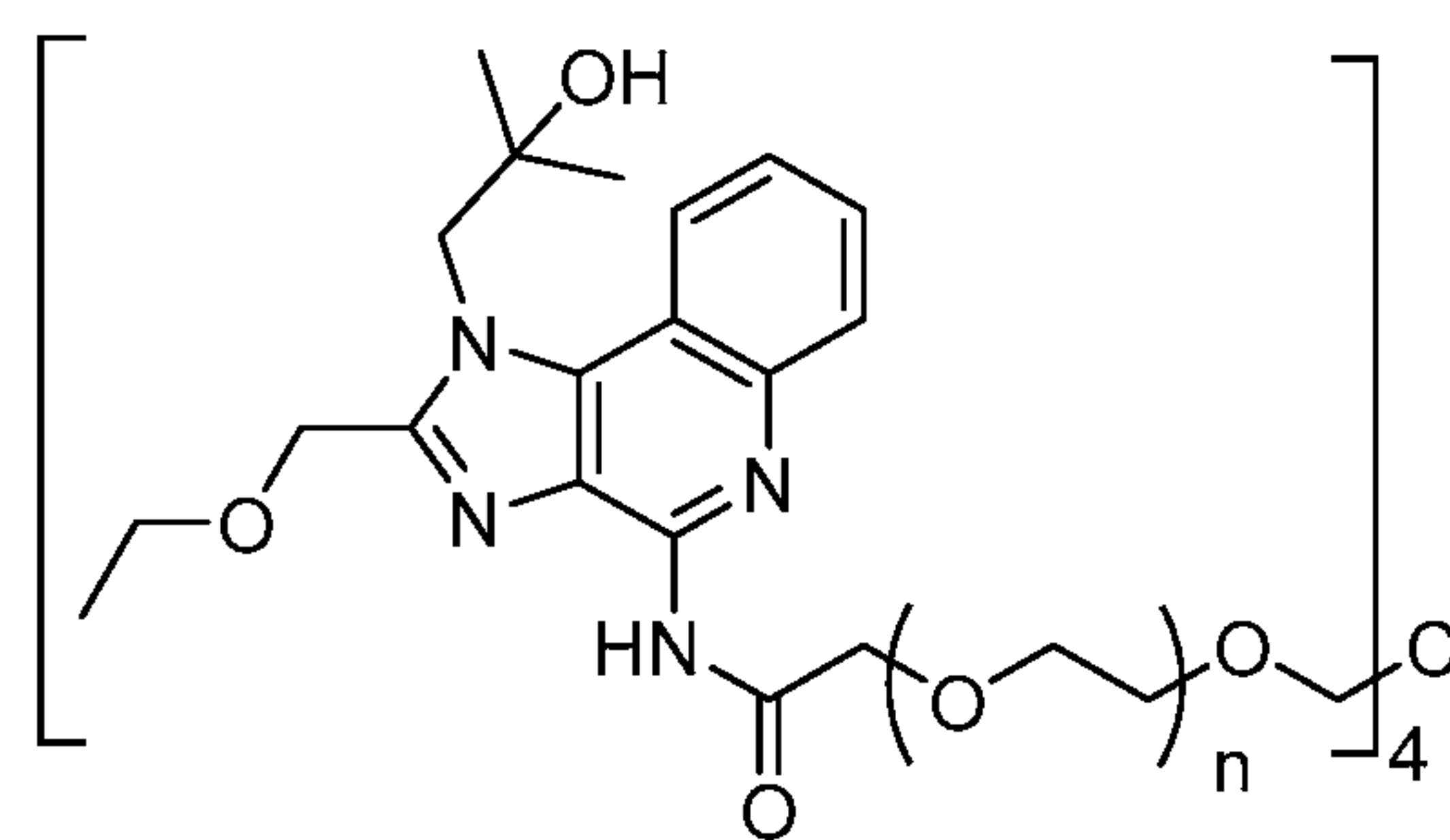
Compound 5
