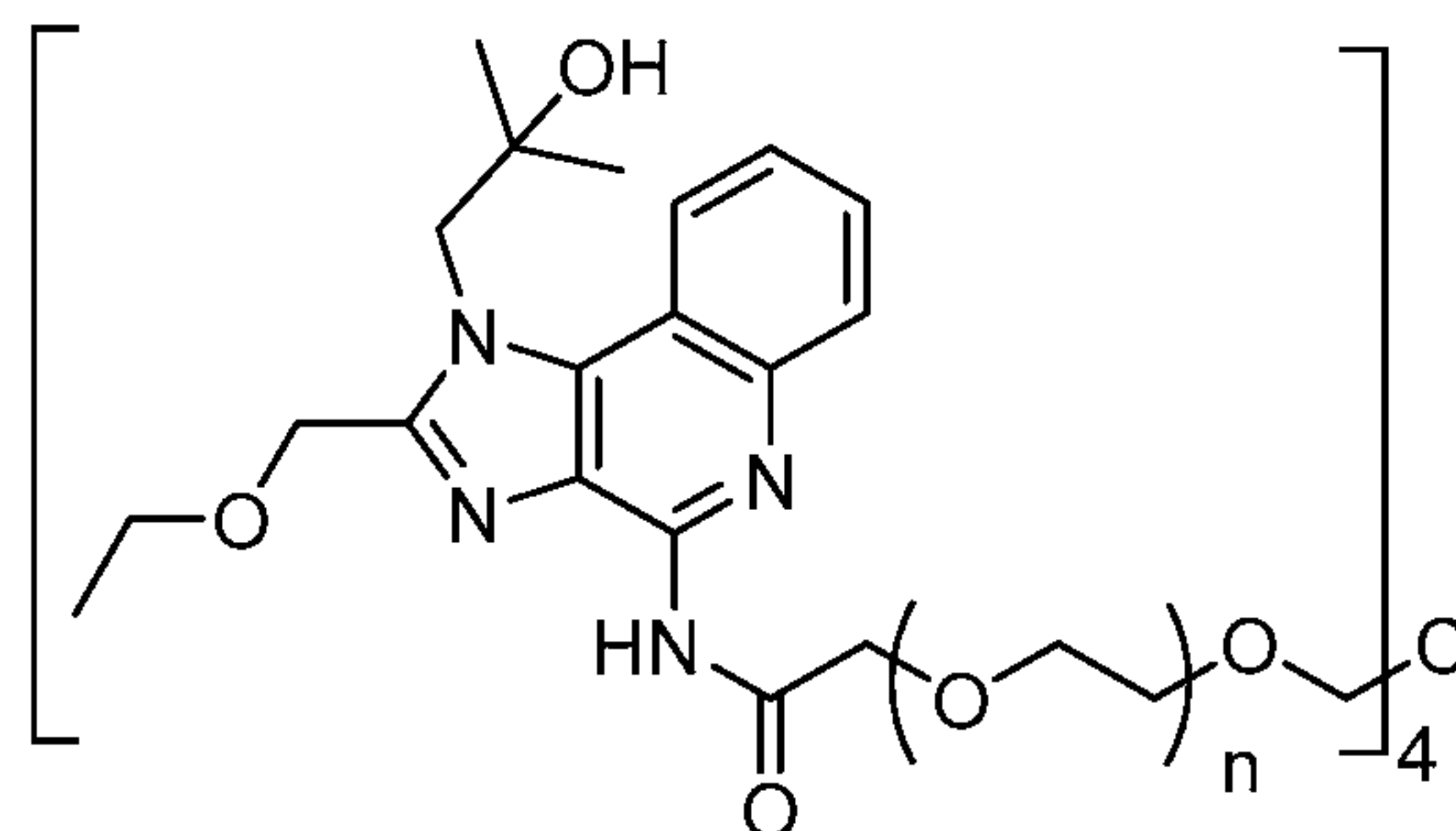
Compound 5
