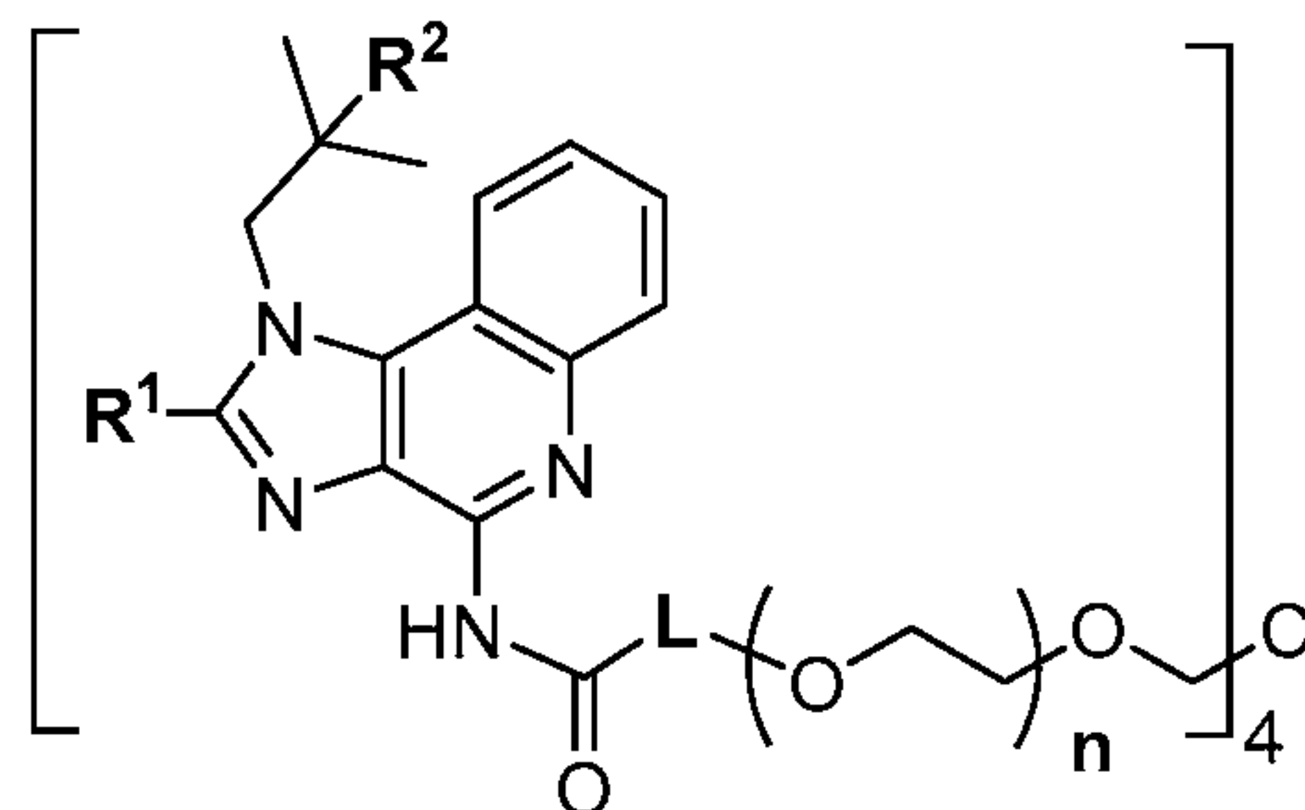
(Formula III)
