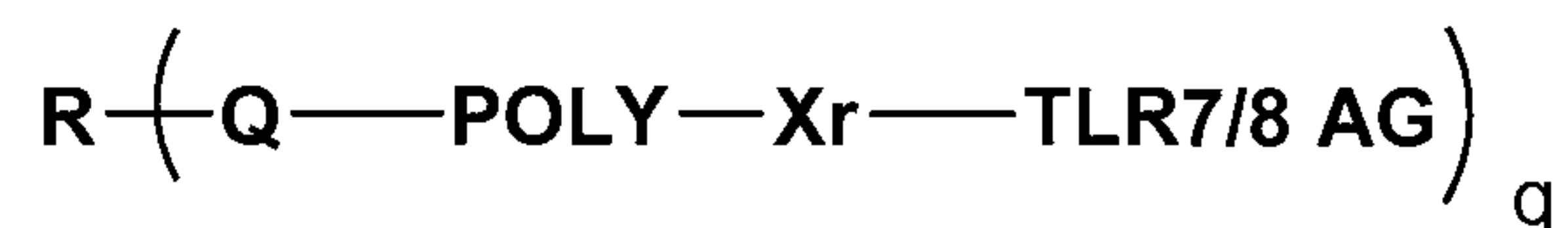
Formula I
