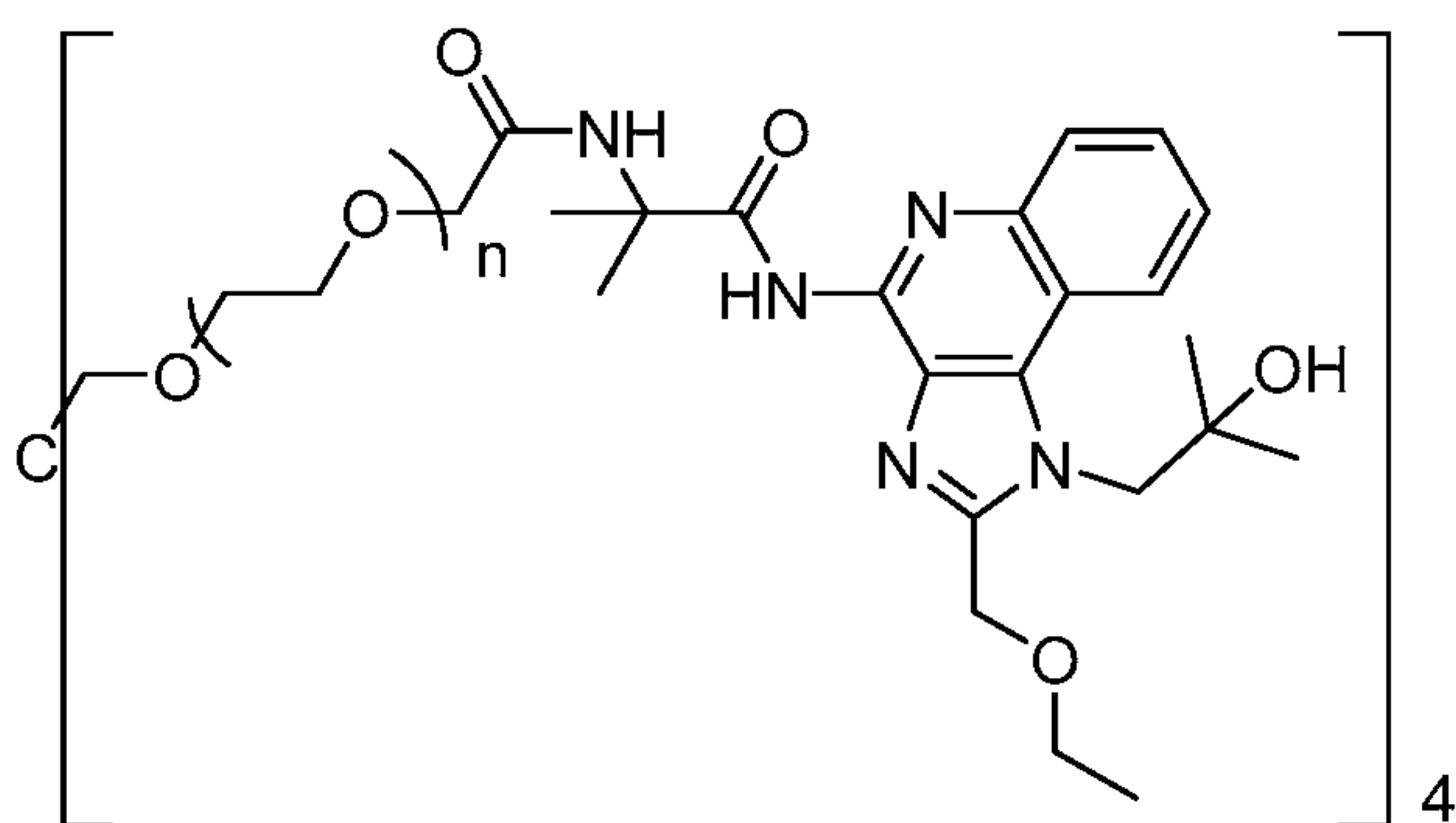
Compound 10
