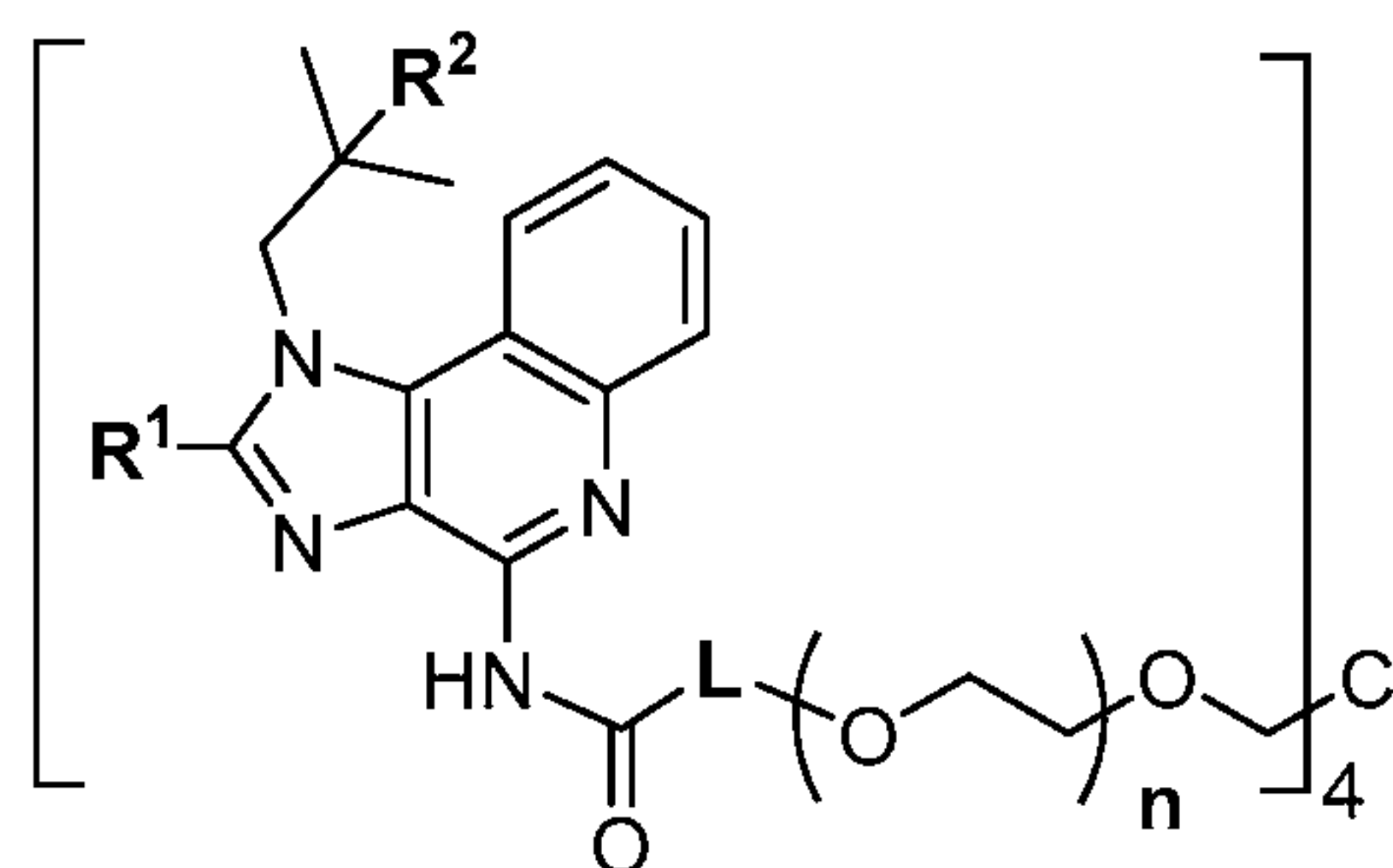
(Formula III)
