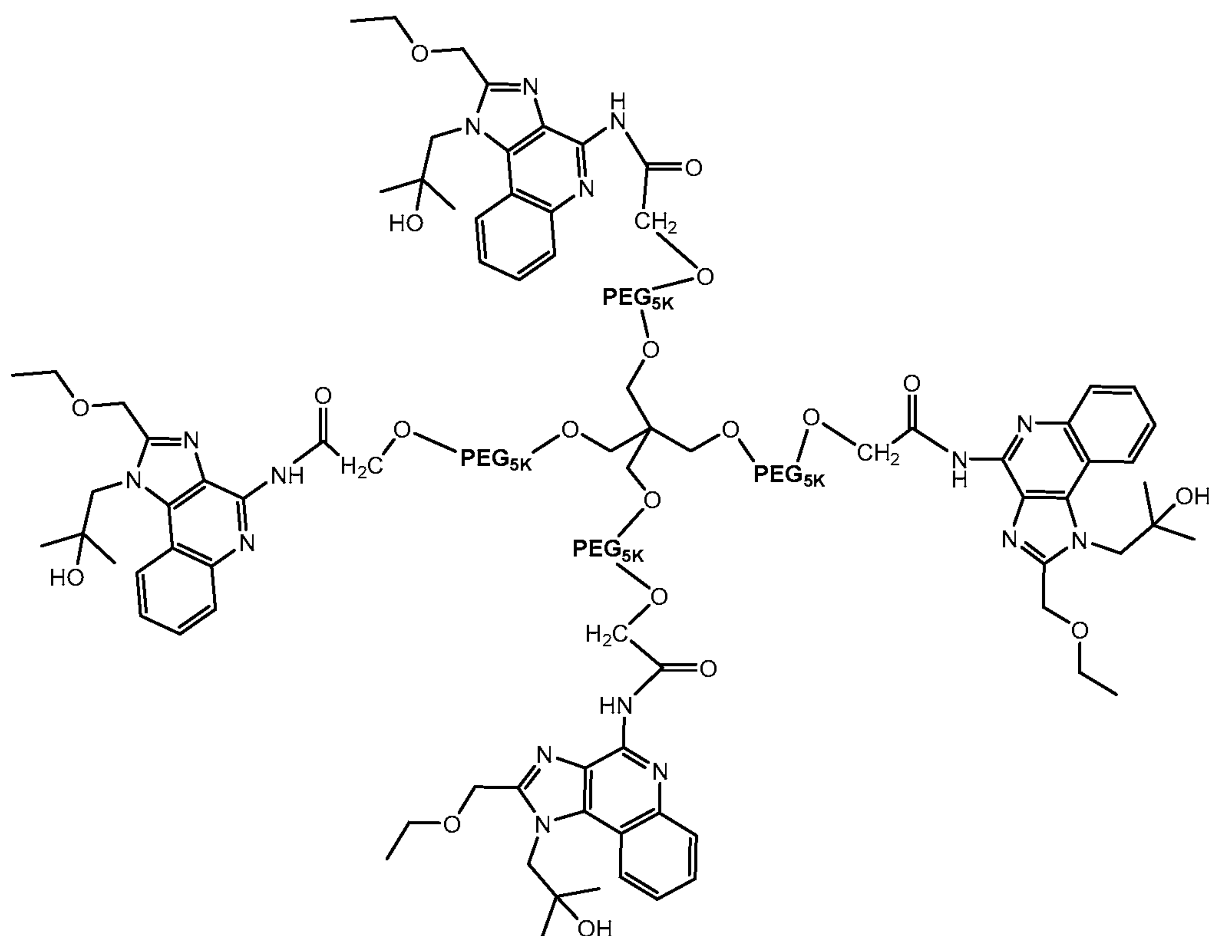
Compound 1
