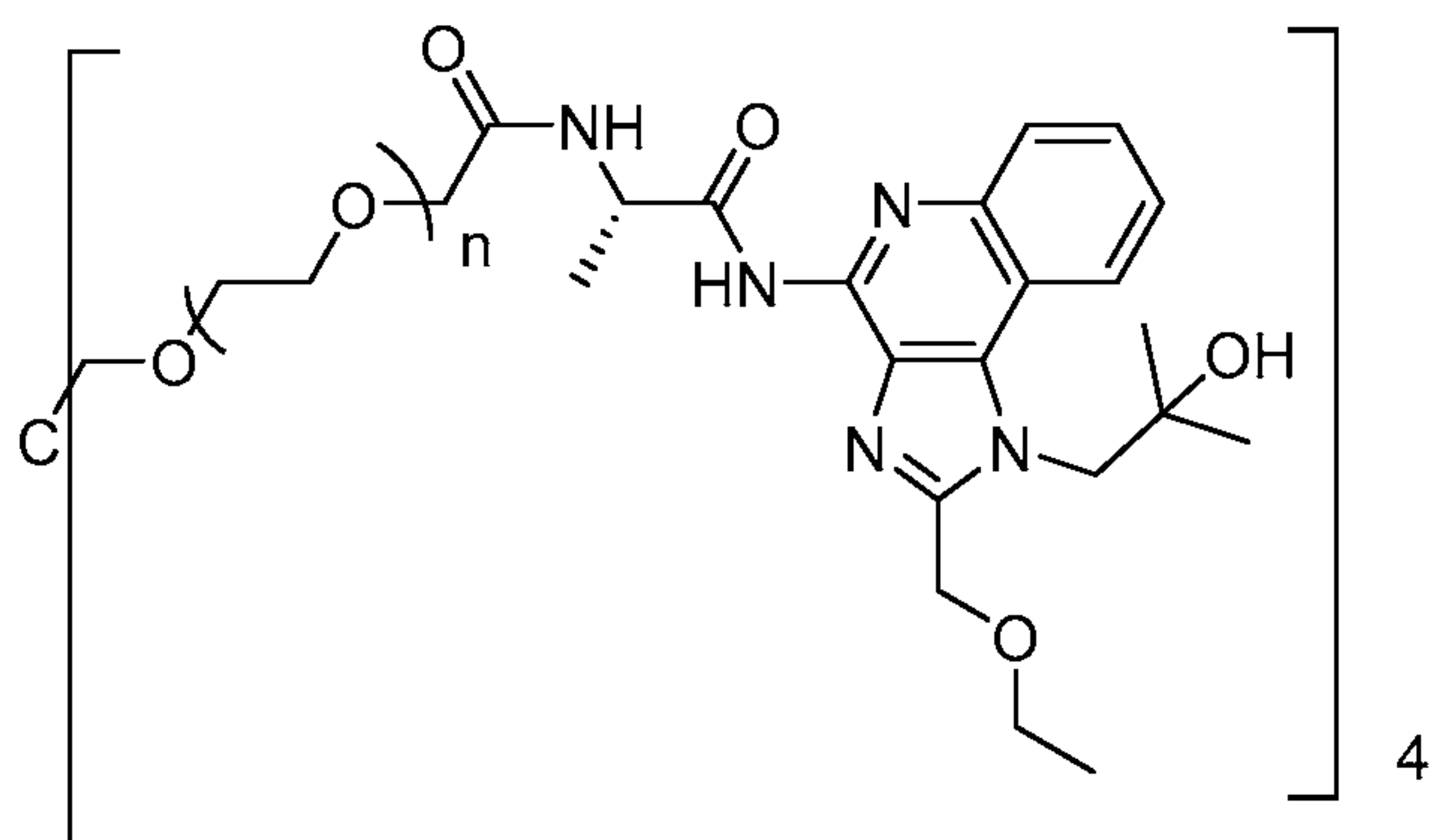
Compound 7
