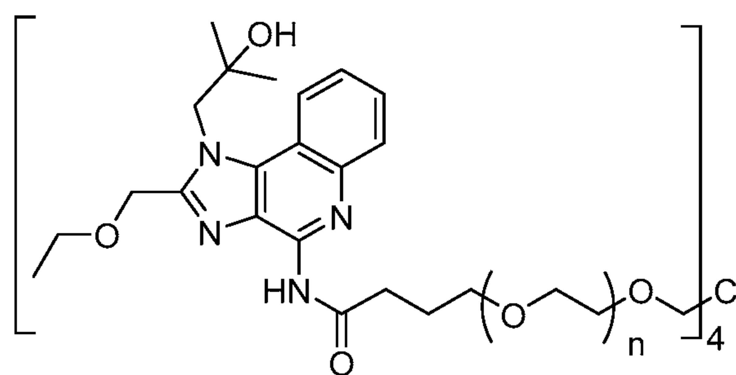
Compound 3
