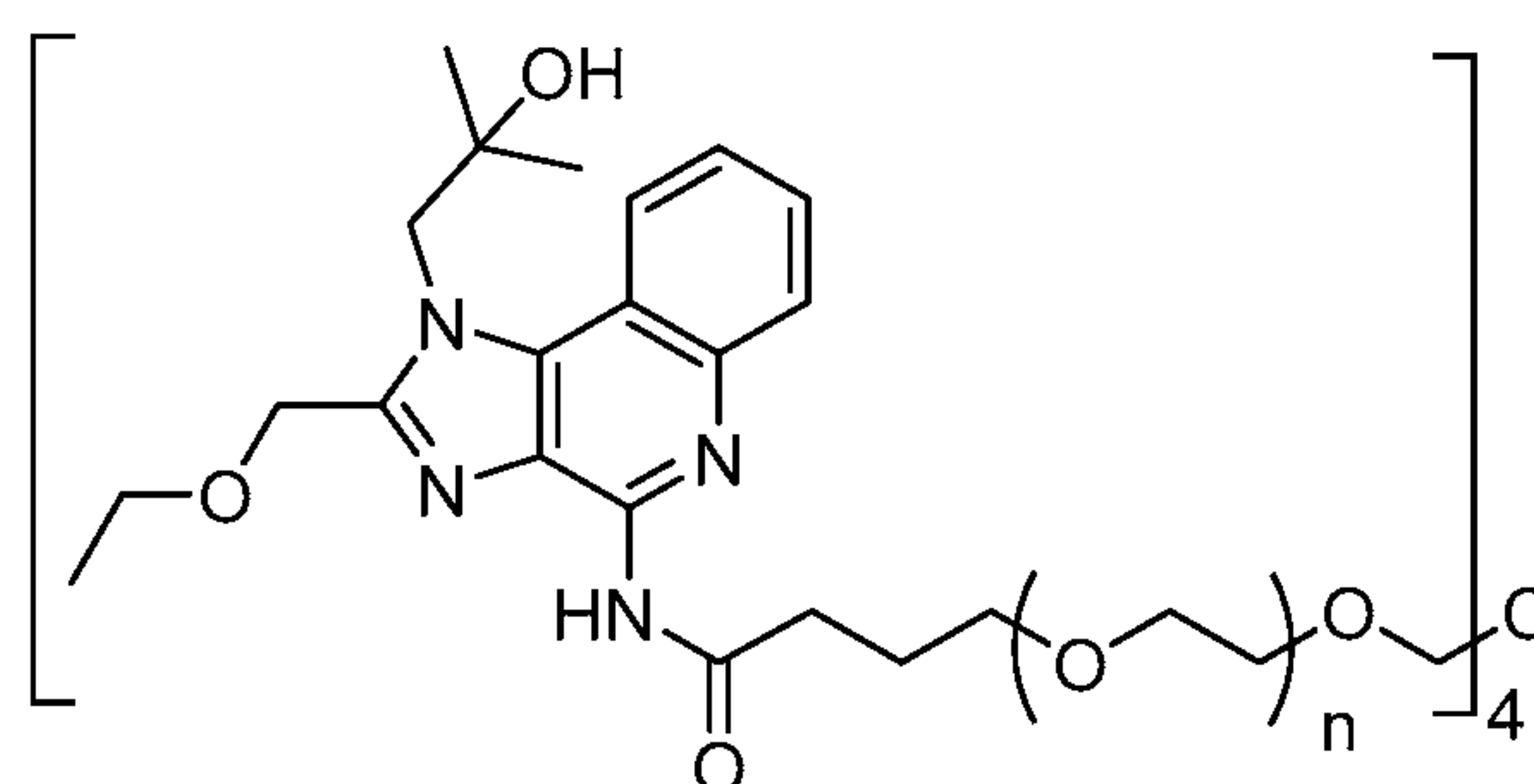
Compound 3
