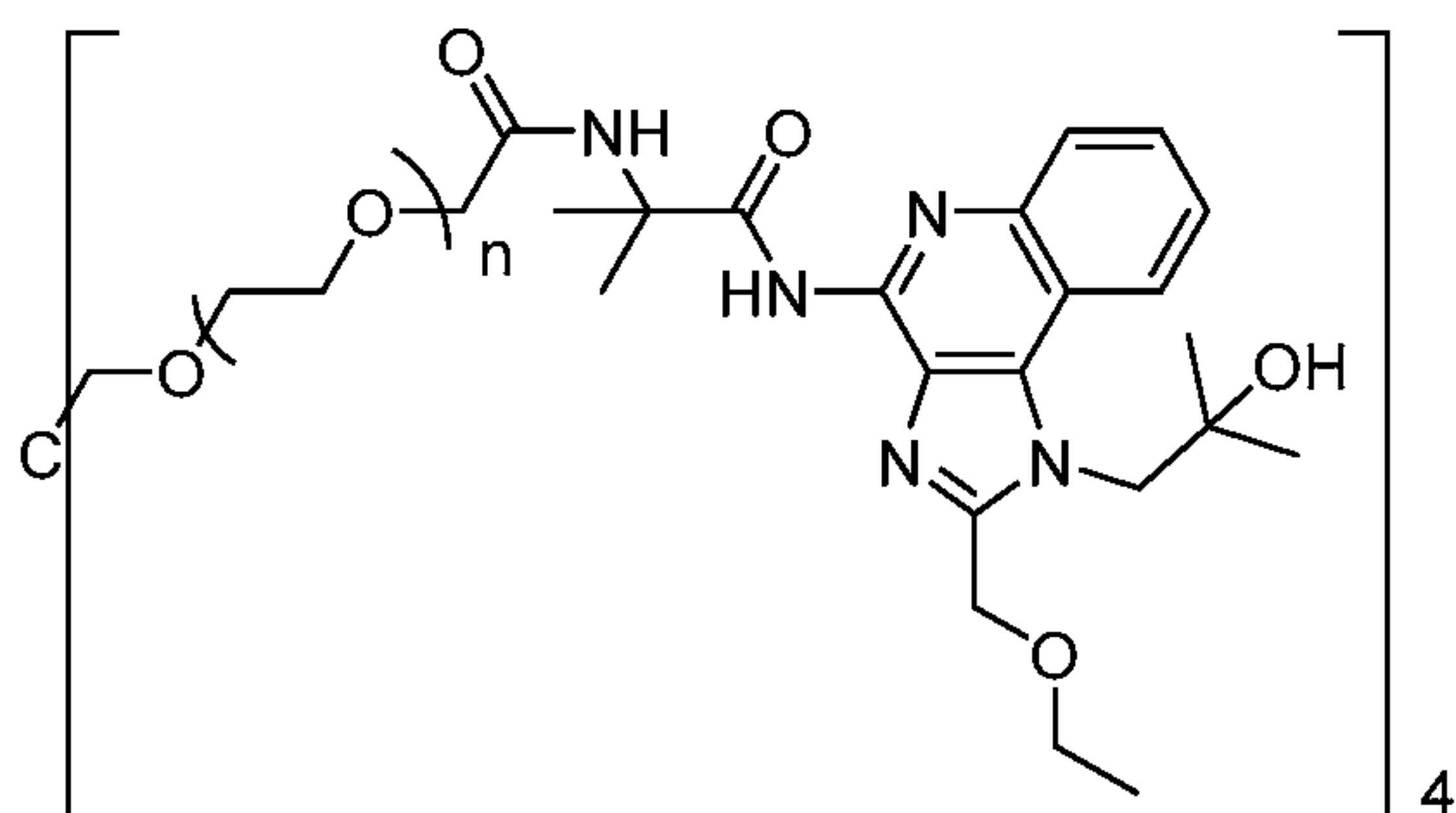
Compound 10
