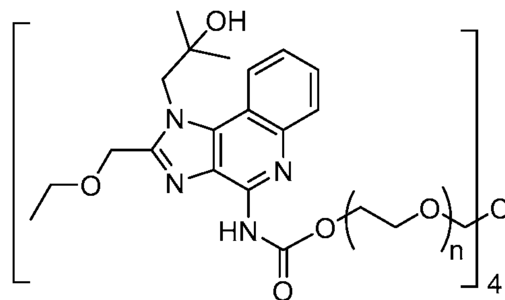
Compound 12
