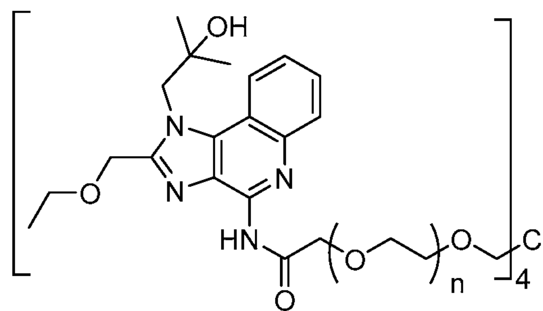
Compound 5
