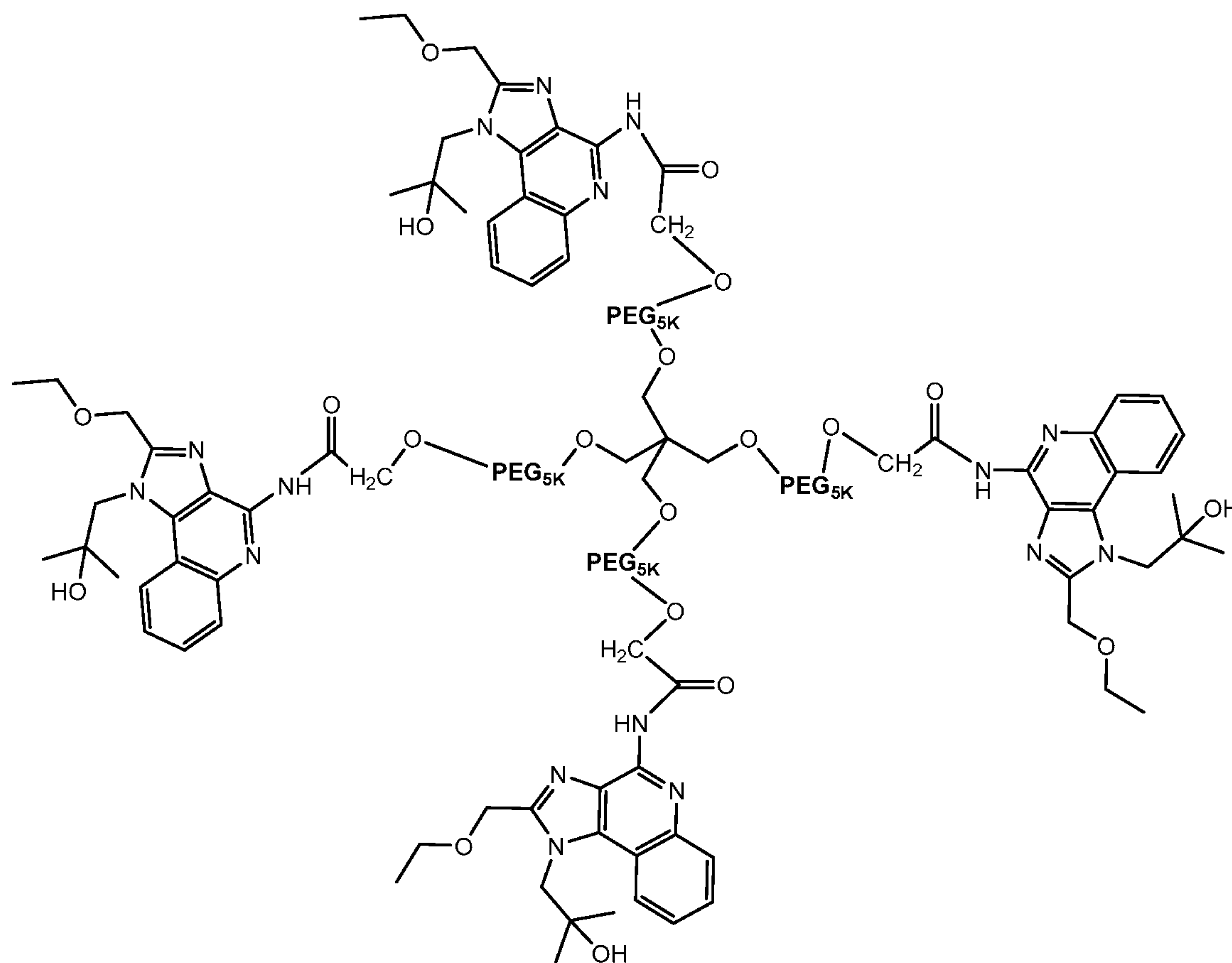
Compound 1
