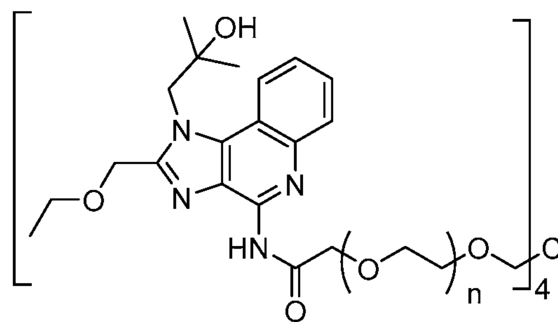
Compound 5
