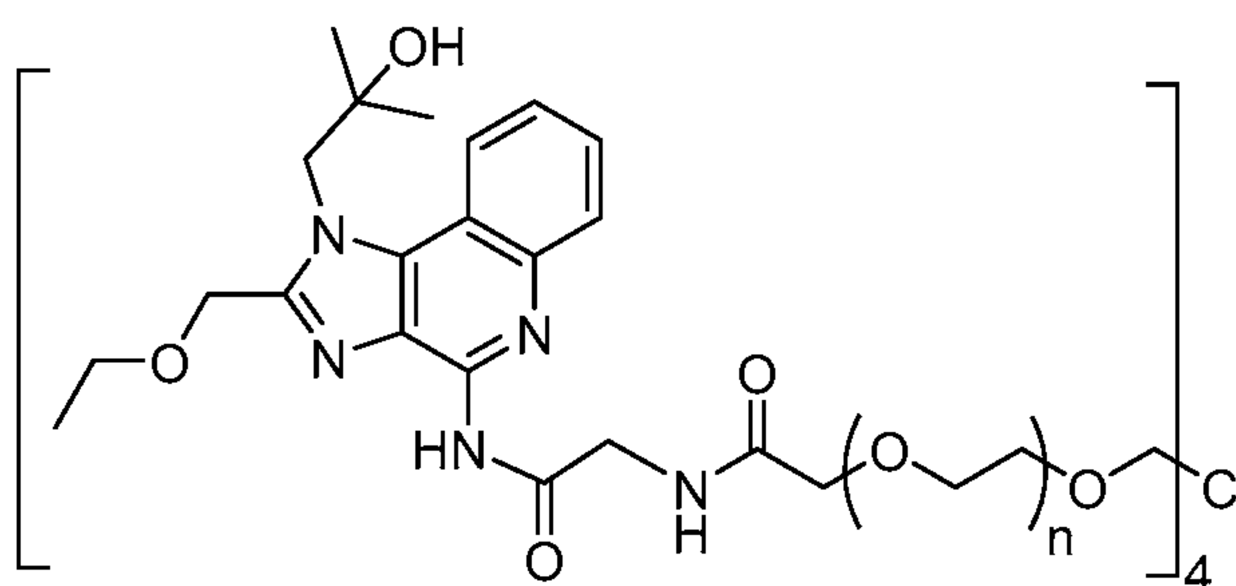
Compound 6
