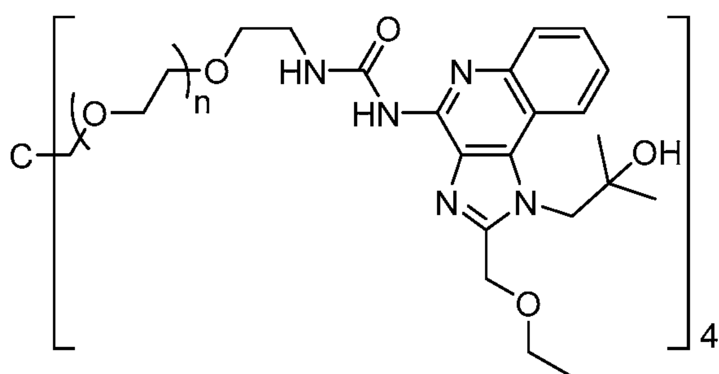
Compound 13
