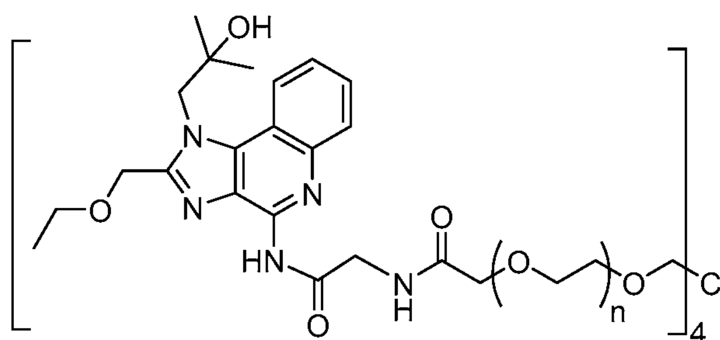
Compound 6
