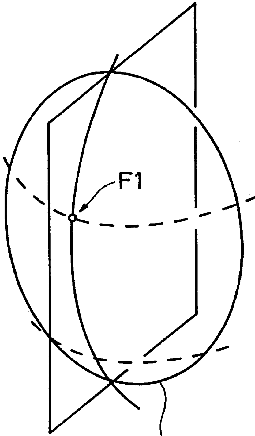
BI-ASPHERICAL TYPE PROGRESSIVE-POWER LENS
