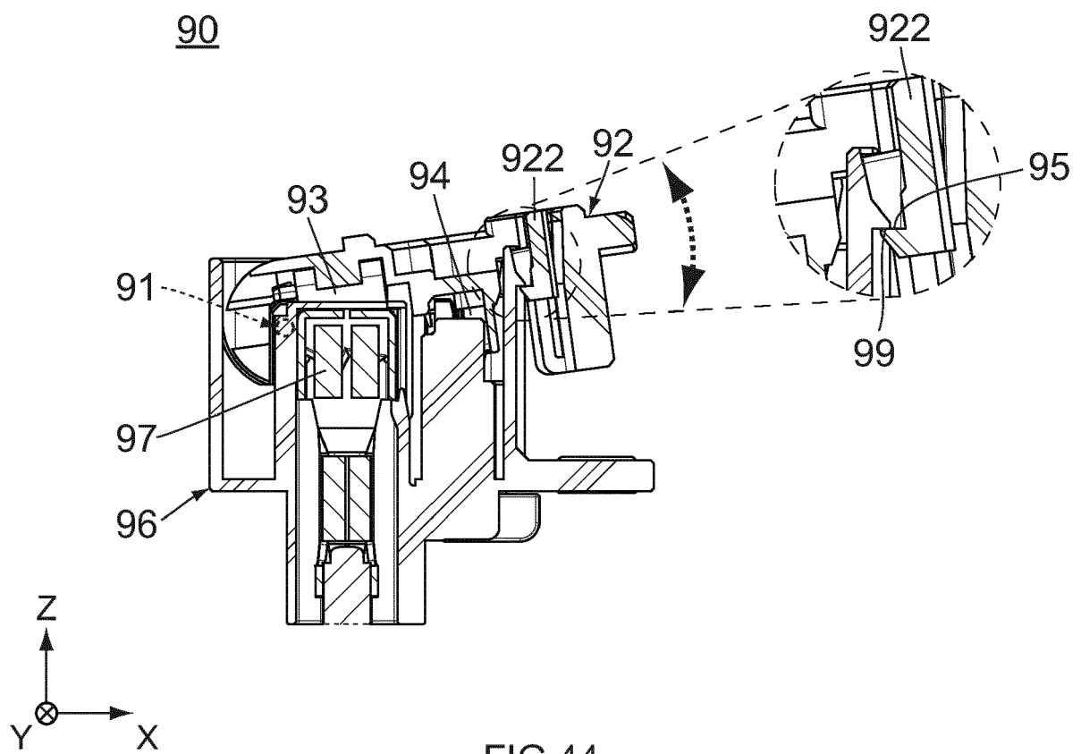
FIG.44 PRIOR ART
