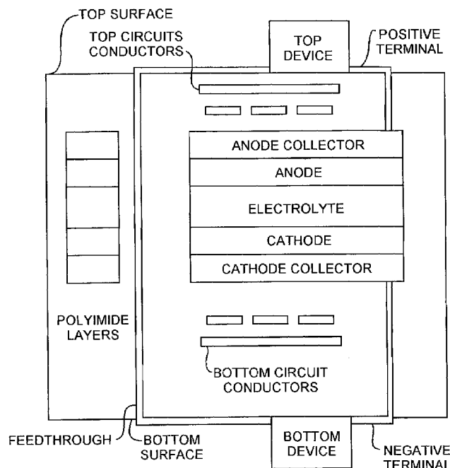
INTEGRATED THIN FILM BATTERY AND CIRCUIT MODULE
