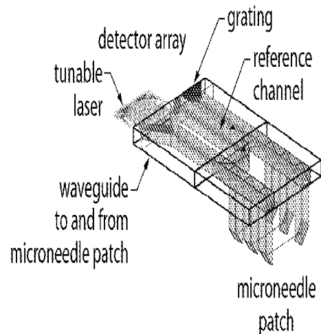
Figure 6: Optical Interrogator
