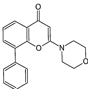
LY294002
