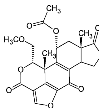
wortmannin
