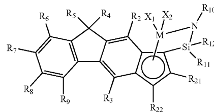
[Chemical Formula 3]
