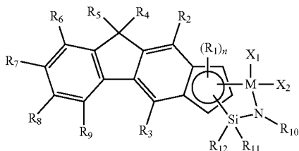
[Chemical Formula 1]
